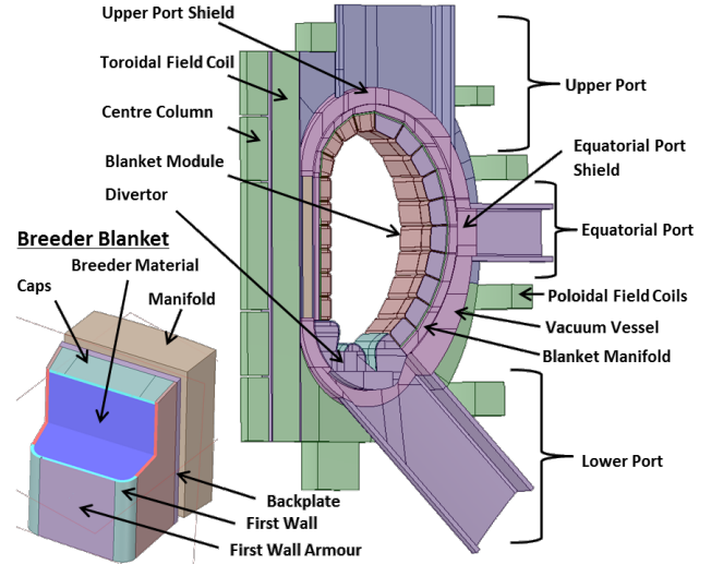
Figure 2: DEMO Generic HCLL MCNP model with homogeneous blanket modules
