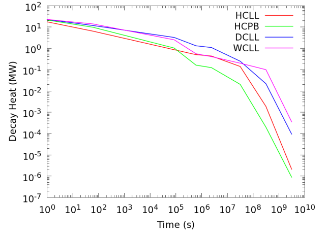
Figure 4: Decay heat for all blanket modules in the DEMO reactor for each concept
