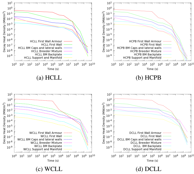
Figure 5: Decay heat density ( \text{MW/m}^3 ) for each of the four blanket concepts
