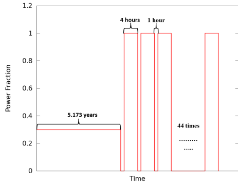
Figure 1: First Blanket Phase Irradiation Schedule
