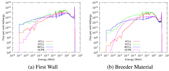
Figure 3: Neutron Spectra for each of the four blanket concepts
