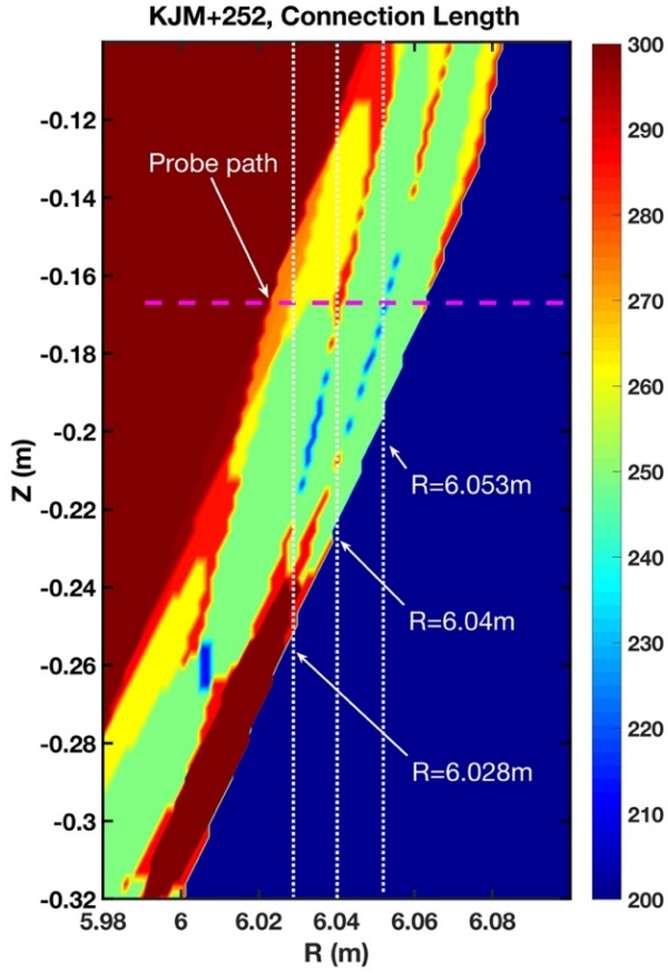
Figure 13. Two-dimension field line connection length for the KJM+252 configuration in the poloidal plane of probe.
