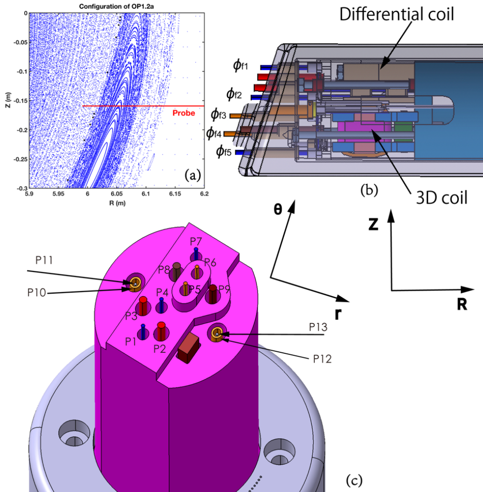
Figure 1. The sketch of the new combined probe used in OP1.2a. (a) A typical island divertor configuration in the poloidal plane of probe, and the red line denotes the probe path. (b) The projection of the probe head viewed along the toroidal direction. (c) The arrangement of all probe pins.
