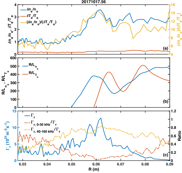
Figure 14. (a) Relative fluctuation levels of electron density and temperature. (b) Normalized gradient scale length of density and temperature. (c) Radial turbulent particle flux, the ratio of particle flux contributed by 0-30 kHz turbulence to the particle flux of the whole frequency, and the ratio of \Gamma_r from 40-160 kHz to the total particle flux.
