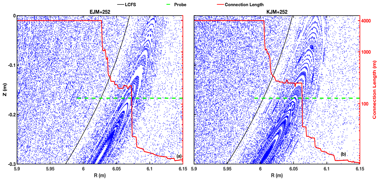
Figure 3. The Poincaré plot of the two configurations of OP1.2a on the poloidal plane of MPM. Panels from left to right are EJM+252 and KJM+252, respectively.
