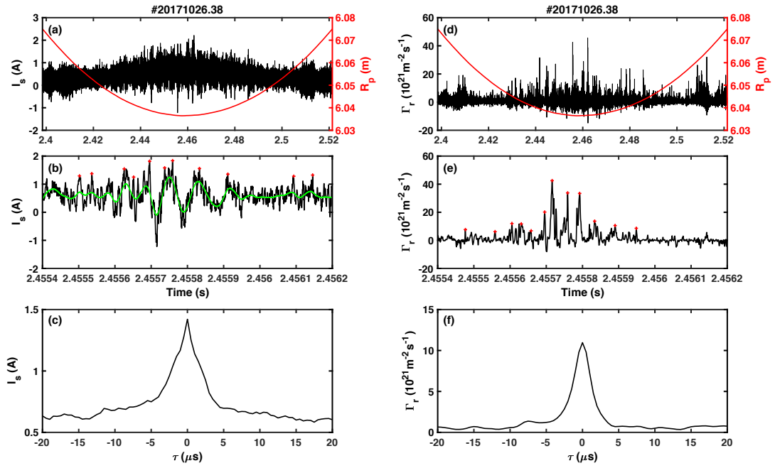
Figure 10. (a-b) Raw signal of the ion saturation current. The red crosses in (b) and (e) means that these spikes are selected by the conditional averaging procedure. The green line in (b) signifies the signal filtered by a 20 kHz low-pass filter. (c) The conditional-averaged ion saturation current in the time period of t = 2.45-2.47 s, i.e., R = 6.036-6.038 m. (d-e) Raw signal of radial turbulent particle flux. (f) The conditional-averaged radial turbulent particle flux in the same time period as (c).
