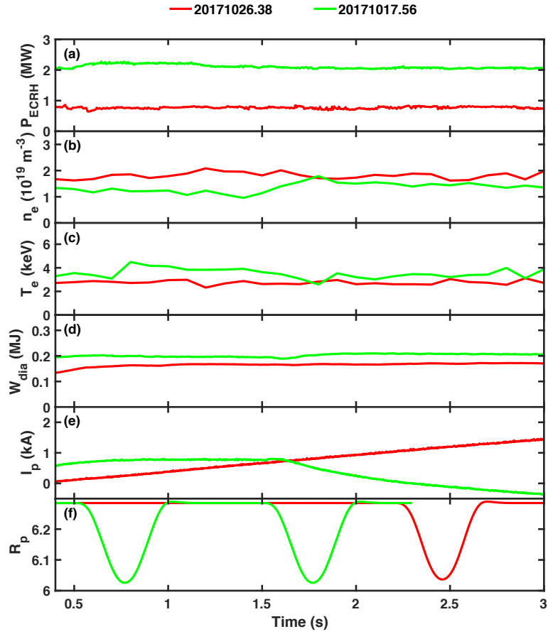
Figure 2. The plasma parameters for the two magnetic configurations in OP1.2a. (a) ECRH heating power. (b) Core electron density measured by Thomson scattering. (c) Core electron temperature measured by Thomson scattering. (d) Plasma energy. (e) Toroidal plasma current. (f) Radial position of the new combined probe.
