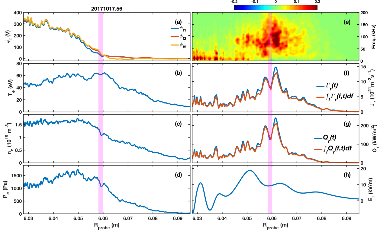
Figure 12. The radial plasma profiles, radial turbulent heat flux and particle flux of the high mirror configuration. The description is the same as Figure 5.
