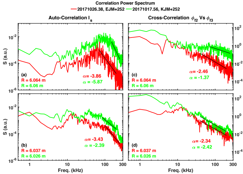
Figure 7. The APSD of the ion saturation current (left panels) and the cross-correlation spectral density (CPSD) between two radially separated floating potential pins (right panels), for both EJM+252 and KJM+252 configurations.
