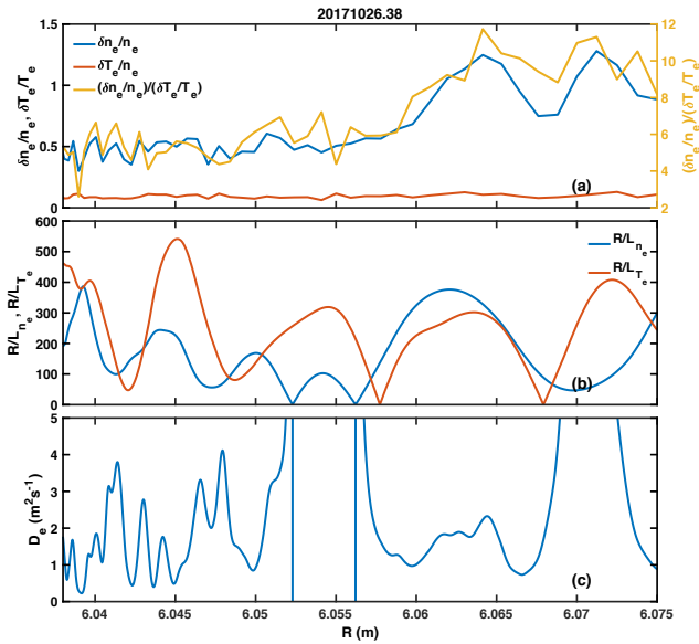
Figure 9. (a) Relative fluctuation levels of the electron density and temperature, and their ratio (\delta n_e/n_e)/(\delta T_e/T_e) . (b) Normalized gradient scale length of electron density and temperature. (c) Electron diffusion coefficient induced by turbulence.
