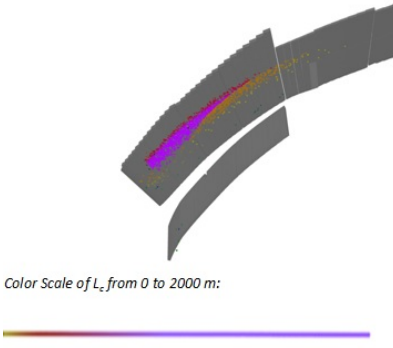
FIG. 3. Footprints of field lines on divertor targets for Low Iota Configuration using field-line diffusion wherein color at each point corresponds to the L_c at that point ( D=1 \text{ m}^2/\text{s} and V=0.5 \cdot 10^6 \text{ m/s} )
