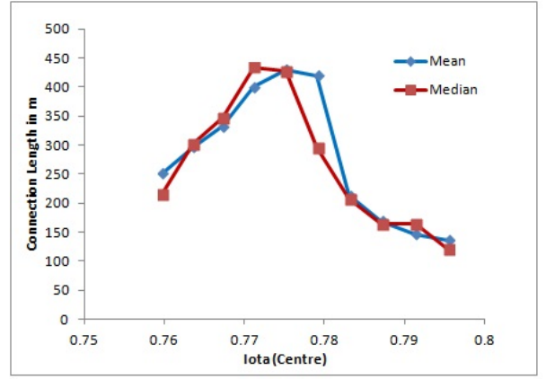
FIG. 5. The Iota Scan using iteration for the New Configuration depicting small variation in planar coil current altering the L_c significantly
