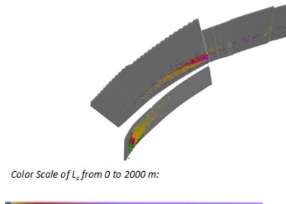
FIG. 2. Footprints of field lines on divertor targets for Limiter Configuration using field-line diffusion wherein color at each point corresponds to the L_c at that point. ( D=1 \text{ m}^2/\text{s} and V=0.5 \cdot 10^6 \text{ m/s} )
