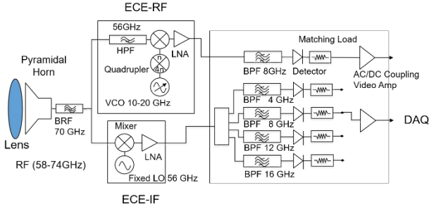
Fig. 2. Schematic view of the CECE radiometer in Heliotron J.
