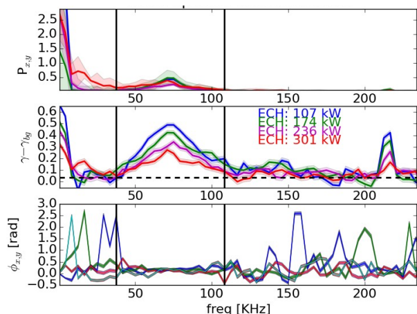
Fig 7. Cross-power, coherence, and phase (top to bottom) between the CECE-RF and CECE-IF channels during an experiment with varying ECCD in Heliotron J.
