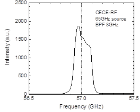
Fig. 4. Frequency conversion and bandwidth of the CECE-RF channel of the CECE radiometer.
