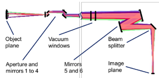
Fig. 2. Optical concept of the endoscopes (first of several beam splitters shown only).
