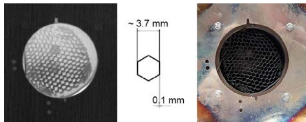
Fig. 10. IR image of cold honeycomb structure in front of a heated plate (350°C) seen from IR camera (left), and real image (right).
