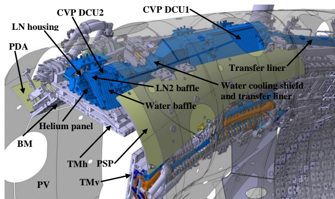
Fig. 1. View of CVP in divertor volume and the adjacent in-vessel components. PV – plasma vessel, BM – baffle, TMh – horizontal target module, TMv – vertical target module, PSP – Pumping gap panel, PDA – poloidal closure.
