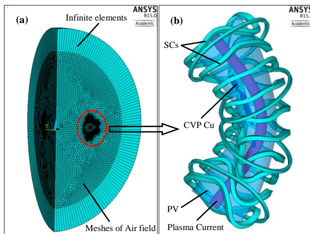
Fig. 6. EM model for CVP eddy current analysis. (a) Overall view of 72^\circ EM model; (b) Model of SCs, plasma current, PV and CVP (top view).
