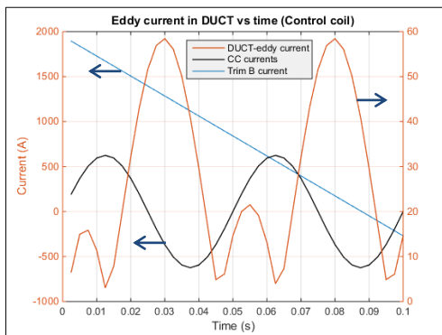
Fig. 12. Current decay of trim coil (discharge rate 22.2 kA/s per turn) and AC in control coil (8 turns × 625 A, 20 Hz), and the induced eddy current in duct (A).
