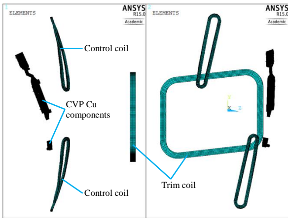
Fig. 8. EM model for CVP eddy current analysis, for the case of FD of trim coil (Type B) and alternative current in control coil.
