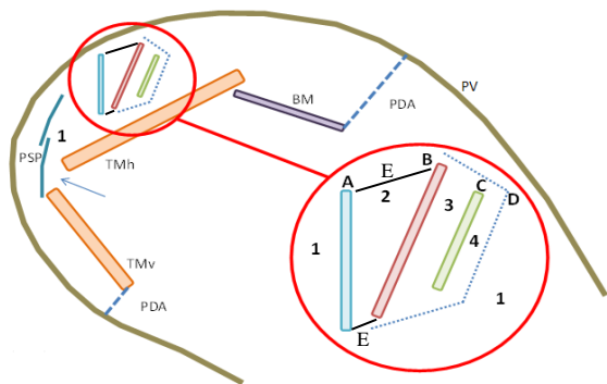
Fig. 2. Schematic view of the divertor chamber cross section (CVP is in red circle). A – water baffle (Cu), B – LN2 baffle (SS), C – helium panel, D – LN2 housing, E – Copper cover (to prevent ECRH power penetrated into CVP through the gap between A and B), 1 – ECRH load in whole divertor chamber, 2 – ECRH load in front of LN2 baffle taking into account the absorption of the water baffle, 3 – ECRH load behind the LN2 baffle, 4 – ECRH load in behind the helium panel.
