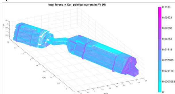
Fig. 15. Force distribution (N, in the center of each element) in CVP Cu components during FD of SCs current and with the consideration of current sharing with PV.
