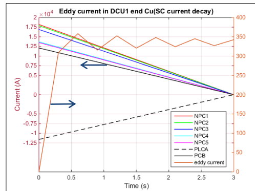
Fig. 10. Current decay curves of SCs (A/turn of each SC) and the integrated eddy current in DCU1 end Cu component versus time.
