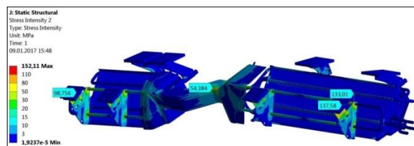
Fig. 20. Primary stresses in SS components due to EM forces and dead weight, MPa.
