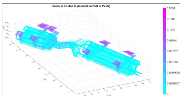
Fig. 16. Force distribution (N, in the center of each element) in CVP SS components due to current sharing with PV (during FD of SCs current).
