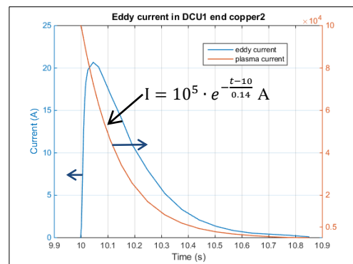
Fig. 11. Plasma current decay curve and the integrated eddy current versus time.
