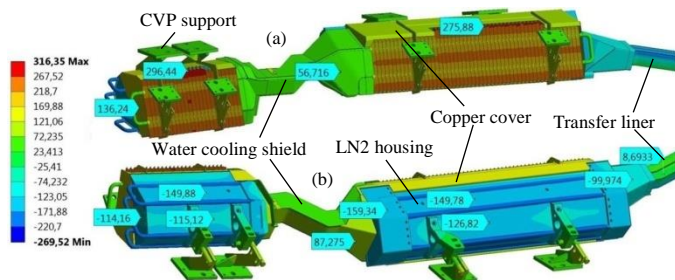
Fig. 4. Temperature distribution of CVP (case TH3, unit °C), (a). Temperature of water baffle, (b). Temperature of LN2 housing.
