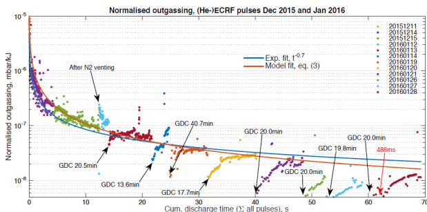
Fig. 7. Outgassing after each ECRH discharge during the first 12 operation days. After this period the gas was changed from He to H 2 with continuation of the trend (adapted from [9])
