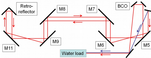
Fig. 3. Schematic picture of the MBS fed by the mirror 4 (M4) which is the last mirror of the SBS and is switchable between the water load (blue beam line) or the MBS to W7-X (red). Optional use of a retroreflector allows the additional power measurement after passing the MBS twice.
