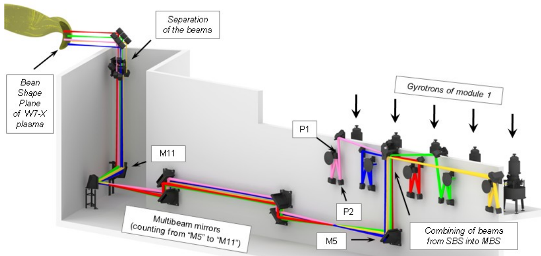
Fig. 1. Fully quasi-optical transmission line to the torus of Wendelstein 7-X
