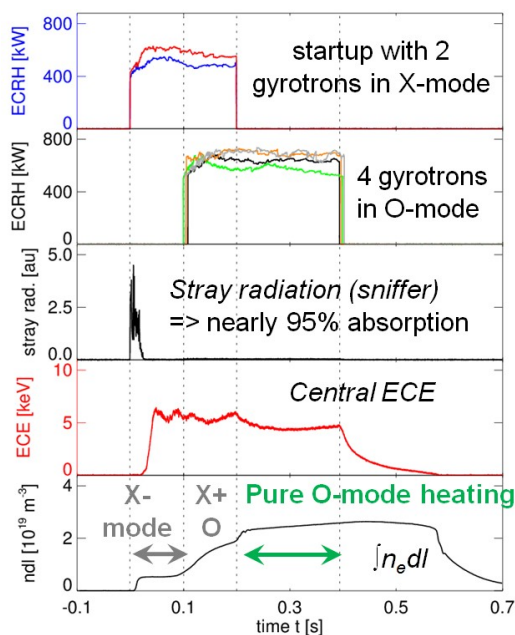
Fig. 15. Temporal evolution of a discharge in which the plasma was sustained by pure O-mode heating using a 3-path-scenario
