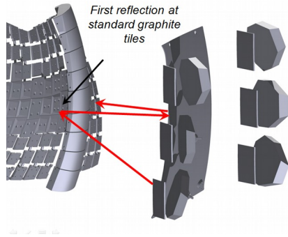
Fig. 14. 3-beam-path-scenario used in OP1.1 to increase the ECRH-absorption in O2-heating scenarios
