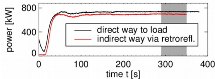
Fig. 4. Evaluation of the efficiency of the MBS by comparison of the gyrotron beam power on a direct way to the load with the indirect way via a retroreflector at the end of the MBS (the evaluated time windows are grey shaded)
