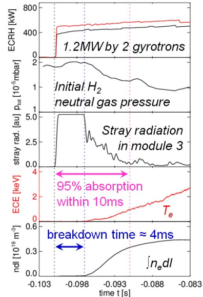
Fig. 8. Temporal evolution of the basic control and plasma parameters during a typical plasma startup in hydrogen
