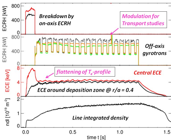
Fig. 11. Temporal evolution of an off-axis scenario with modulated gyrotrons for transport studies
