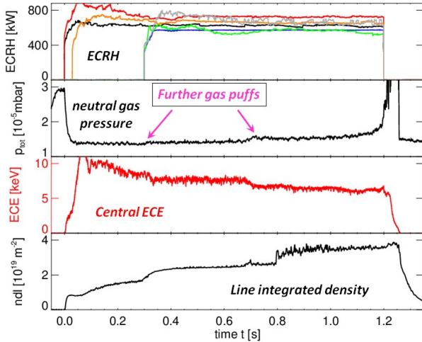
Fig. 10. Temporal evolution of a discharge with the maximum ECRH power available in OP1.1
