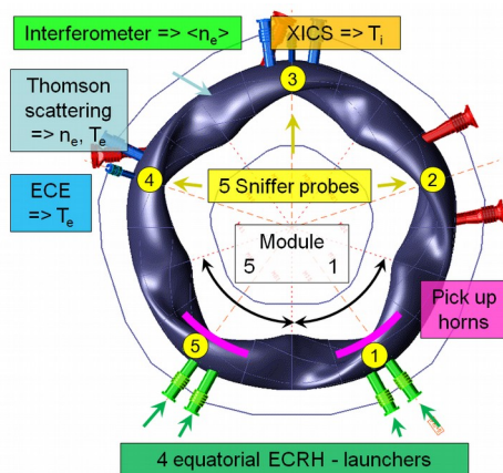
Fig. 5. Top view on the W7-X torus with the positions of the main diagnostics and the ECRH launchers in module 1 and 5.
