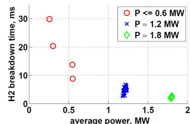
Fig. 9. Breakdown time in H 2 -plasmas in dependence on the used ECRH power
