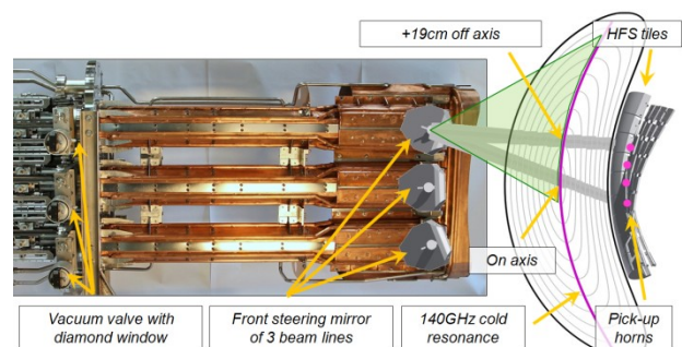
Fig. 2. Cross section of one of the 4 ECRH launchers in relation to the vacuum flux surfaces of the limiter configuration in OP1.1. The beam with a diameter of about 80mm in the plasma centre is shown for two examples of the upper beam line. Its whole steering range is visualized by the green shaded area.
