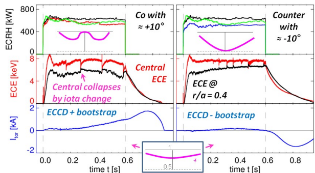
Fig. 13. Comparison of ECCD scenarios with Co- and Counter-driven currents to the rotational transform (expected change of iota profile is sketched in pink)
