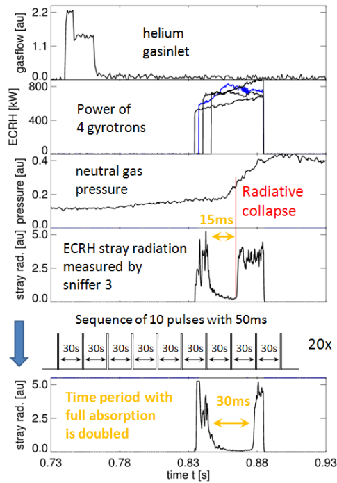
Fig. 6. Temporal evolution of a cleaning discharge after 0.1s cumulated discharge time compared with the stray radiation after 3s cumulated discharge time
