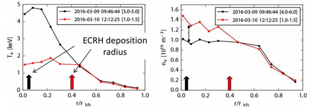
Fig. 12. T_e and n_e profiles of an on- and off-axis heated discharge with a heating power of 0.6 MW (adapted from [11])
