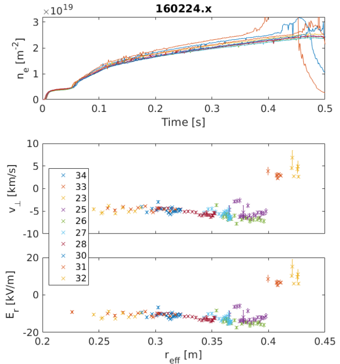
FIG. 5: Line averaged density (a) of a series of discharges. The v_{\perp} and related E_r as function of r_{eff} . The different colours indicate the different discharges. Note the change in sign at the plasma edge.
