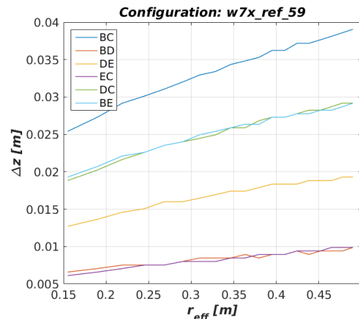
FIG. 4: Distance between the all receiver combination in z direction as function of r_{eff}
