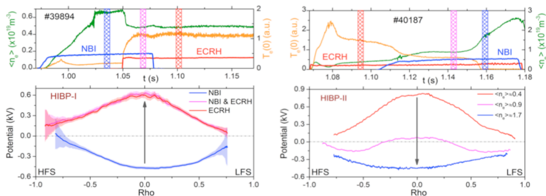
Fig. 2 Time evolution of plasma density and electron temperatures with combined ECRH / NBI regimes and corresponding plasma potential profiles in the TJ-II stellarator. The plasma potential reverses from negative values to positive values in low density plasma (left) but not at high density (right) regimes with combined ECRH and NBI heating. ECRH was on axis for shot #39894 (left) and off-axis for shot #40187 (right).
