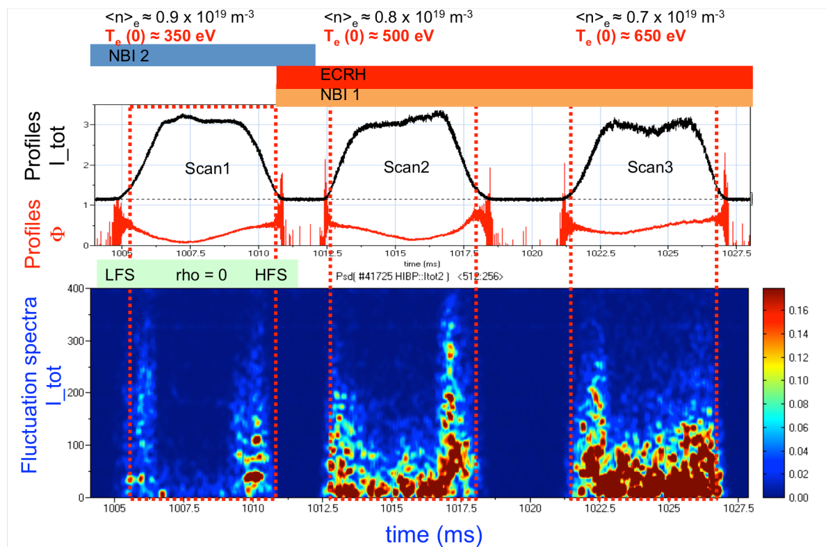
Fig. 3 Influence of ECRH on density fluctuation profiles (shot 41725) measured with the HIBP-I system in the scanning mode.
