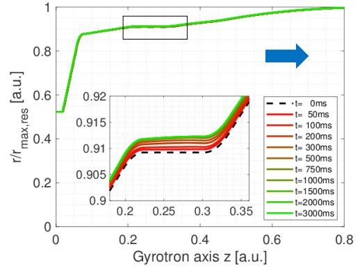
Fig. 6. Evolution of the radial profile of the heated surface of the resonator. The water flow direction is indicated by the blue arrow.
