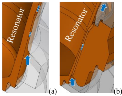
Fig. 7. CAD models of the annular (a) and of the mini-channels (b) cooling options of the coaxial cavity resonator. Blue arrows indicate the main water flow directions.
