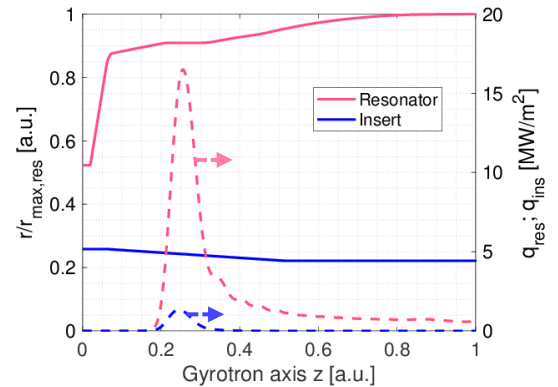
Fig. 3. Initial heat loads (dashed lines) and initial (non-deformed) heated surface radial profiles (solid lines) for the resonator and of the insert is scaled with the maximum radial radius of the resonator.
