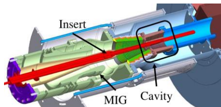
Fig. 1. CAD model of the coaxial cavity [2].
