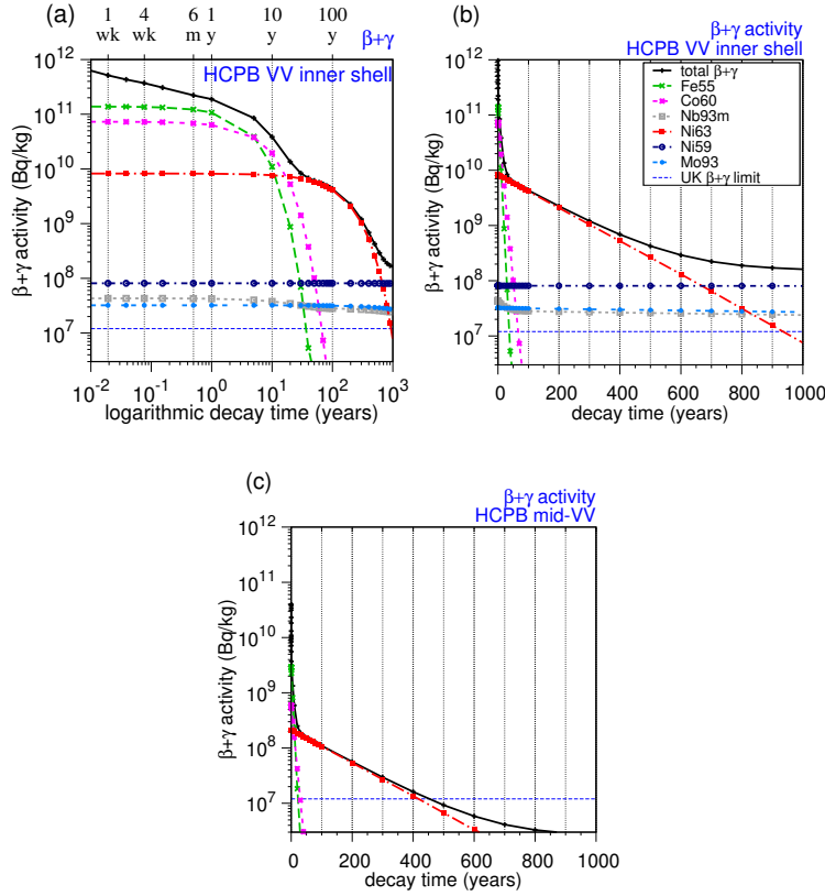
Figure 5. Nuclide contributions to SS316 activity under the predicted conditions in the inboard equatorial Vacuum Vessel (VV) behind the HCPB breeder blanket concept. In (a) the variation in activity for the VV inner shell (nearest the plasma) is shown against a logarithmic decay timescale (measured from DEMO EOL), while in (b) a linear timescale is used for the same VV zone. (c) shows the activity decay profile (on a linear time x-axis) for a middle layer of the VV interspace (between the inner and outer shells). In each plot the total activity is shown, together with curves representing the contributions from important radionuclides. The UK-specific low-level waste (LLW) limit for \beta + \gamma emissions (none of the dominant radionuclides in this case are alpha emitters) is also shown as a horizontal dashed line.
