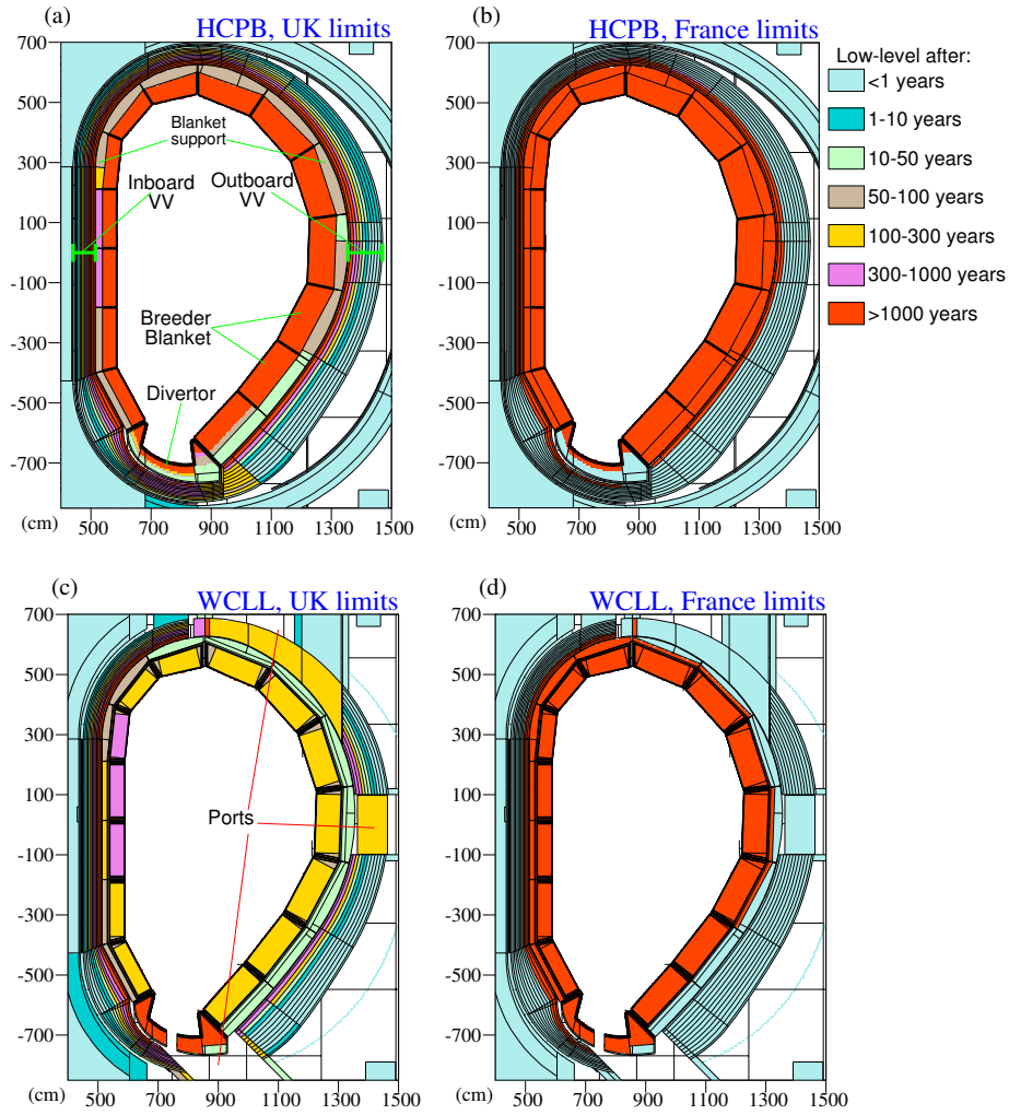
Figure 3. Toroidal slices of the DEMO model with (a,b) HCPB and (c,d) WCLL breeder blanket concepts. In each cross-section, homogenised material regions (cells) are coloured according to the time-interval (shown in the key and measured from DEMO EOL) during which the material is predicted to satisfy the criteria to be classified as low-level waste (LLW) according to (a,c) UK or (b,d) French regulations.
