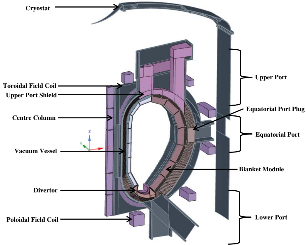
Figure 1. MCNP model geometry of the helium-cooled pebble-bed (HCPB) DEMO design concept.
