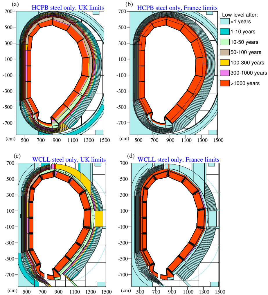
Figure 4. Toroidal slices of the DEMO model with (a,b) HCPB and (c,d) WCLL breeder blanket concepts. In each cross-section, regions (cells) are coloured according to the time-interval (shown in the key) during which the steel in that region is predicted to satisfy the criteria to be classified as low-level waste (LLW) according to (a,c) UK or (b,d) French regulations.
