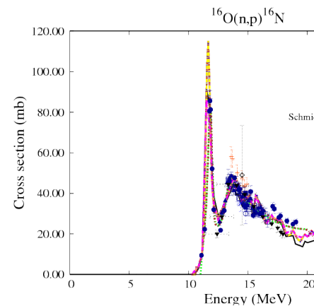
Fig.6: Evaluated and measured cross-sections for ^{16}\text{O}(n,p)^{16}\text{N} . (The curve labelled "TALYS" refers to the updated cross-section)
