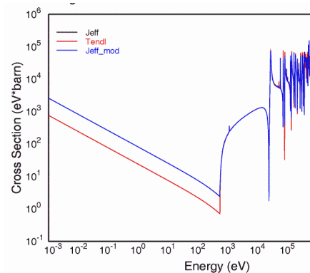
Fig. 3: Displacement damage cross-section of n + {}^{56}\text{Fe} (Jeff_mod denotes the data included in the dpa library).
