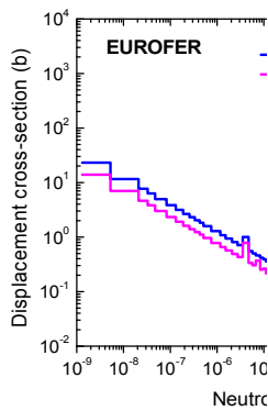
Fig. 4: Displacement damage cross-section evaluated for Eurofer steel with BCA-MD and NRT damage models.
