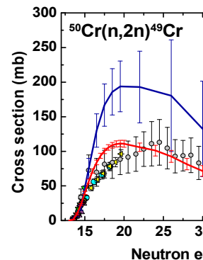
Fig. 2: Calculated (blue line) and evaluated (red line) cross-sections for the {}^{50}\text{Cr}(n,2n){}^{49}\text{Cr} reaction.
