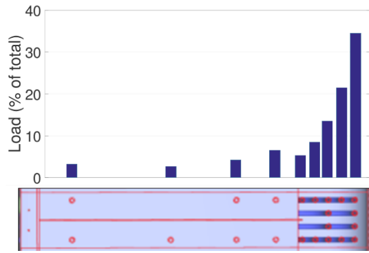
Fig. 7. Power distribution in one elementary cell.
