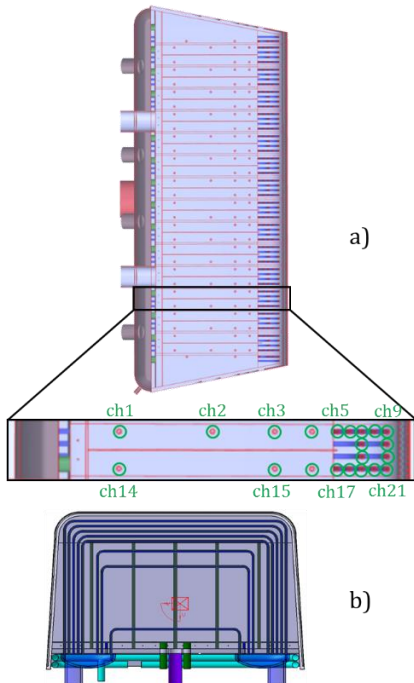
Fig. 6. Radial-poloidal (a) and radial-toroidal (b) cut of OB4, showing the details of the elementary cell in the inset; the 21 channels are circled in green in the inset (adapted from [3]).
