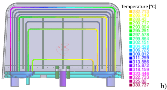
Fig. 8. 1D profile along the channel (a) and distribution in the radial-toroidal plane (b) of the coolant temperature in four selected cooling channels out of the 21 of an elementary unit of the OB4 module.
