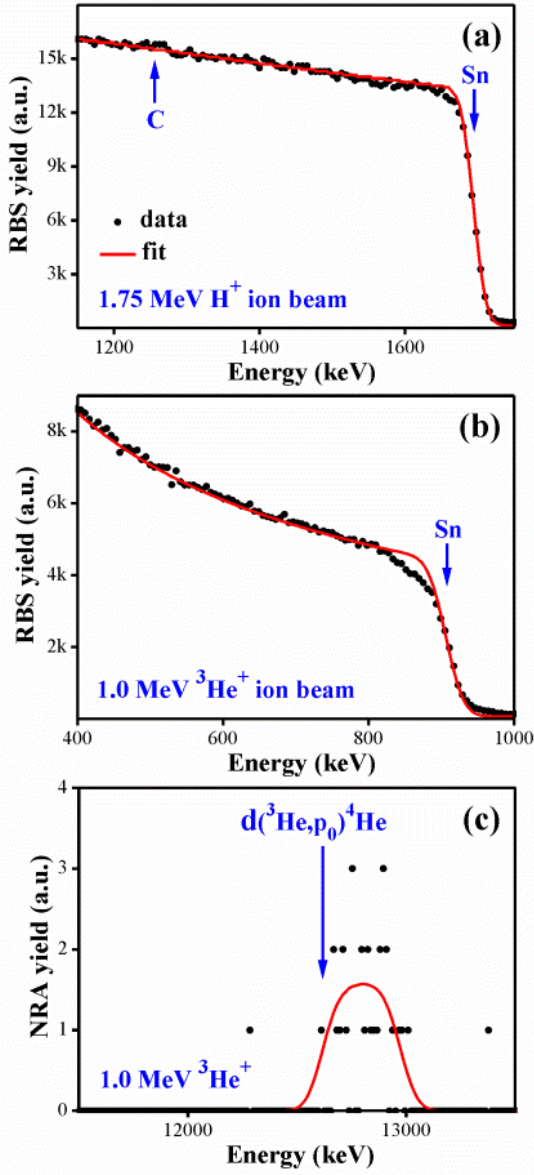
Fig. 5. (a) RBS with incident 1.75 MeV proton beam; (b)(c) RBS and NRA analyses with incident 1.0 MeV ^3\text{He}^+ ion beam, respectively.
