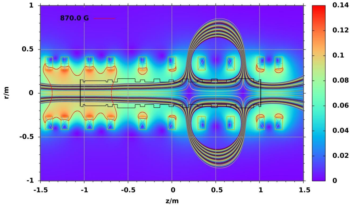
Fig. 2. Double-cusp magnetic configuration in GyM device. The red line indicates the resonance position, the black line the silhouette of the chamber.
