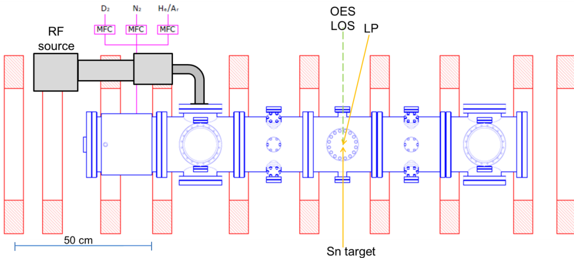
Fig. 1. Schematic of Gym plasma device.
