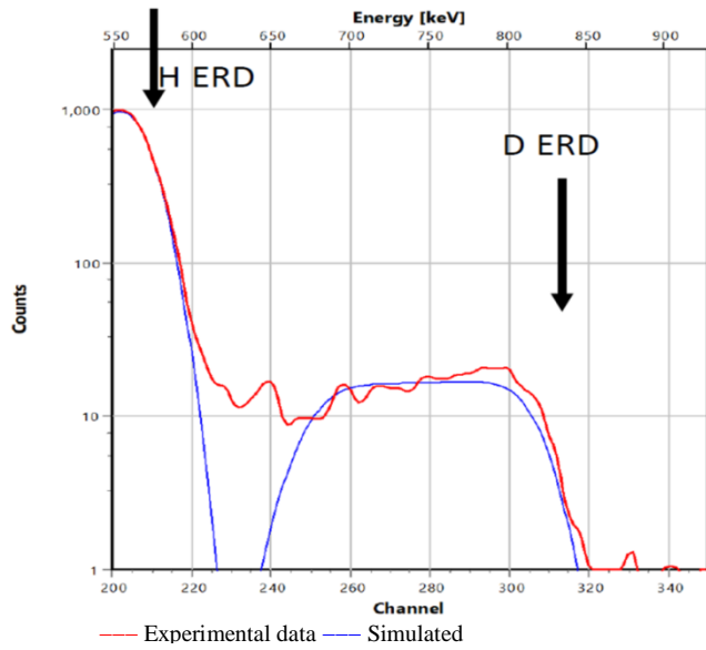
Fig. 4. ERDA experimental spectrum (only deuterium part) taken at \theta_{IN} = 75^\circ , \theta_{OUT}=30^\circ , E_\alpha = 2000 keV using a 10 \mu\text{m} Mylar absorber foil. I_{\text{Beam}} \sim 15 nA. Deuterium uptake calculated up to a depth of 3 to 4 \times 10^{17} at/cm 2 of Sn (corresponding to a maximum of about 90 -100 nm - see simulation) is about 0.25 at%. Deuterium is clearly seen to penetrate at larger depths.
