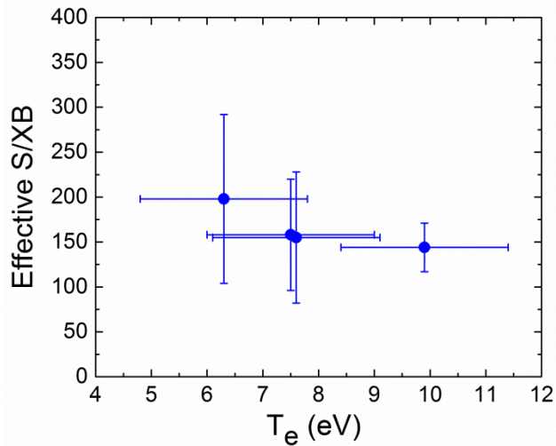
Fig. 6. Effective S/XB for Sn I line at 380.1 nm ( n_e = 1.5 \times 10^{11} \text{ cm}^{-3} ).
