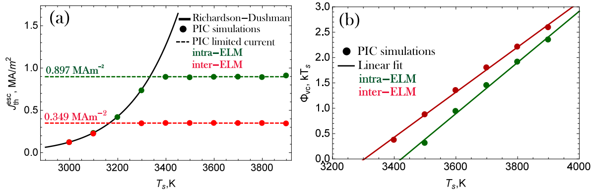
Figure 2. Sloped geometry results of the PIC simulations for the selected plasma scenarios. (a) The escaping thermionic current as computed by the particle counting method (●) and the average limited current (dashed lines). (b) The virtual cathode depth normalized by the surface temperature (●) and its linear least-squares fit (continuous lines).
