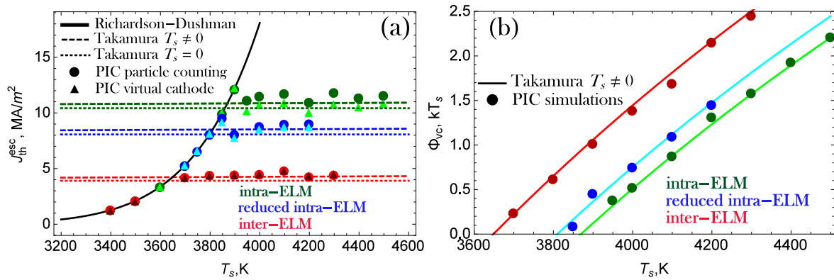
Figure 1. Leading edge geometry results for the selected plasma scenarios. (a) The escaping thermionic current from the PIC simulations as computed by the particle counting method (●) and the virtual cathode method (▲) together with the space-charge limited current as calculated by the Takamura model for T_s \neq 0 (dashed lines) and T_s = 0 (dotted lines). (b) The virtual cathode depth normalized by the surface temperature resulting from the PIC simulations (●) and the finite- T_s Takamura model (continuous lines).
