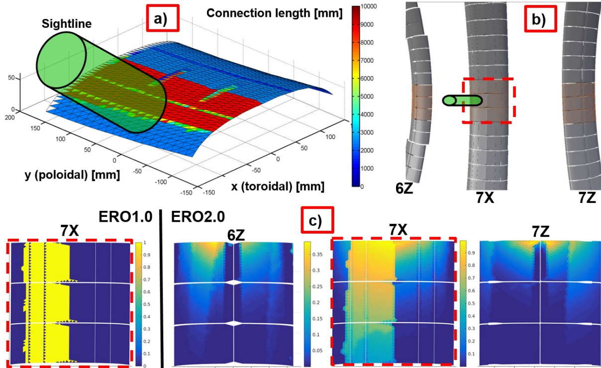
FIG.1. The passive spectroscopy at IW ‘7X’ guard limiter: a) The connection length pattern simulated by the PFCFlux code for the midplane part of the 7X limiter [22]; b) The inner wall guard limiters ‘6Z’, ‘7X’ and ‘7Z’ and sightline location; c) shadowing patterns simulated with crude (‘ERO1.0’) and refined (‘ERO2.0’) assumptions [18].
