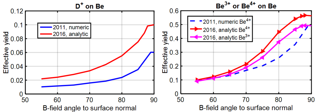
FIG.4. The effective yields Y_{eff}(\eta) integrated on the basis of the pre-calculated angle and energy distributions of the sputtering ions on impact. The older pure numeric ERO simulations used in [3] and recent simulations on the basis of analytic expressions [6]. T_e=10 , T_i=20 are constant for the whole surface of the ITER blanket module considered in [3] in the assumed 'high density' conditions.
