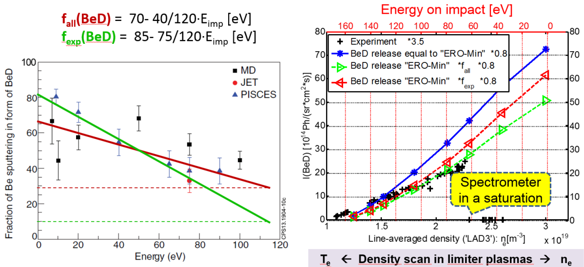
FIG.2. The BeD band emission simulated by ERO (total) and observed in experiment (right) using the fits for the fraction of BeD release from obtained on the experimental (‘PISCES’, ‘JET’) and simulated (‘MD’) data from [5]. Measurements are multiplied by 3.5 to obtain the total band intensity whereas only a fraction of it depending on the vibrational and rotational temperatures is coming into the spectral window.
