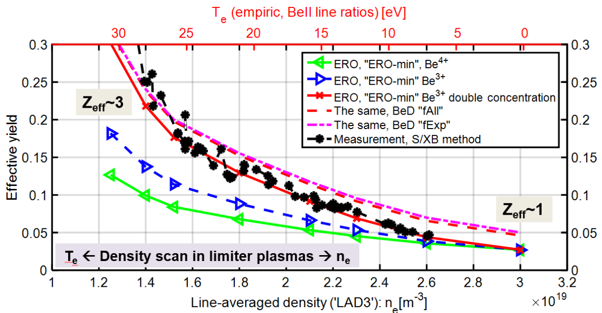
FIG.3. The effective sputtering yields in ERO and S/XB method measurements. The physical sputtering yield fit for Be with 50%D in the interaction layer ('ERO-min') is used [3]. The effect of self-sputtering assumptions (all Be ions charge and concentration) is illustrated. The analytical expressions [10] are used to produce the effective yields. The remaining uncertainties in the influence of CAPS and the intrinsic Be impurity concentration (leading to self-sputtering) are illustrated. The BeD release fractions "fAll" and "fExp" are explained in FIG.2 (left).
