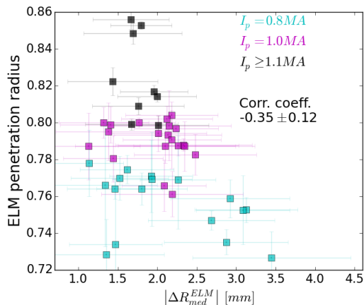
Figure 7: ELM penetration radius as a function of the median value of the ELM-induced (inward) jump of R_{med} , |\Delta R_{med}^{ELM}| .
