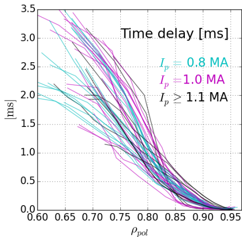
Figure 8: Radial profiles of the average cold pulses time-delay (defined in the text) for all the considered plasmas. Note that the unclear dependence of the time-delay on the plasma current is briefly discussed at the end of section 4.
