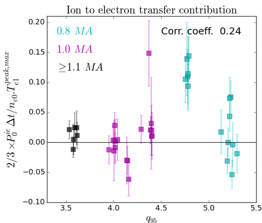
Figure 9: Contribution of the unperturbed ion to electron energy exchange to the T_e drop (cf. equation 2), taking \Delta t = 1 ms, and evaluating the energy exchange at \rho_{pol} = 0.8 . No correlation is observed.
