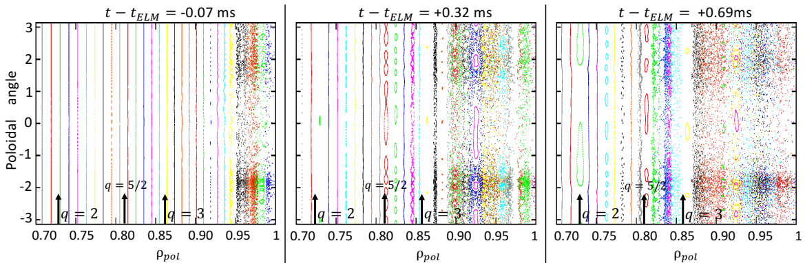
Figure 11: Poincaré plots of the magnetic field lines calculated by JOREK using as an input the kinetic profiles of shot #33616 at 7.2s ( I_p = 0.8 MA), and shown at three values of t - t_{ELM} (where t_{ELM} is the onset of the ELM crash): -0.07 ms, 0.32 ms, 0.69 ms. The magnetic topology is represented in the (\rho_{pol}, \theta) plane. A stochastic layer at the edge, and the formation of island chains at rational surfaces (e.g. q = 2 , q = 5/2 ) are observed.
