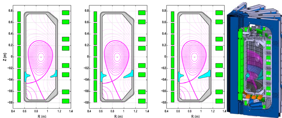
FIG. 3. (Left) Sketches of baffles for varying divertor closure, limiting the SOL at the flux surface with an outboard midplane separatrix separation of \sim 1 cm, 2 cm, and 3 cm, respectively, with centered X-point. (Right) 3D view for the case with the longest baffles. (Reproduced from [4].)
