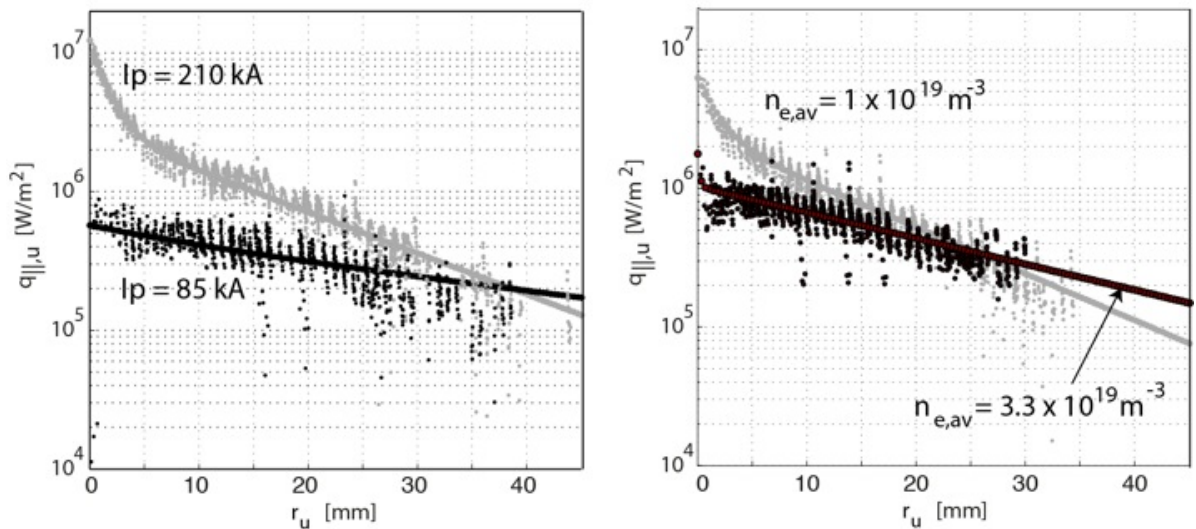
FIG. 8. Profiles of parallel heat flux to the target mapped to the outboard midplane in inboard limited plasmas for (left) two current values at line-averaged density 1.7 \times 10^{19} \text{ m}^{-3} and (right) two density values at a plasma current of 140 kA. (Reproduced from [28].)
