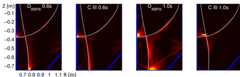
FIG. 5. D_\alpha and C III emissivity profiles 0.4 s before and at the onset of detachment (occurring at 1.0 s). (Reproduced from [20].)
