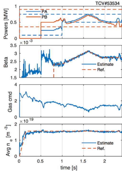
FIG. 10. TCV shot with simultaneous \beta and density control, using two ECRH sources (PA and PB). (Reproduced from [42].)
