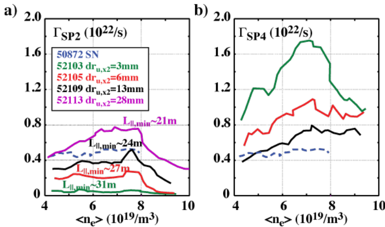
FIG. 7. Ion currents to (a) SP2 (lower primary inner-wall strike point) and (b) SP4 (outermost secondary strike point) for density ramps in LFS SF- configurations for varying X-point separation dr_{u,x2} . (Reproduced from [16].)
