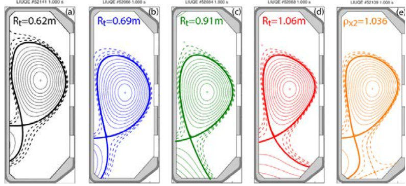
FIG. 6. Flux-surface contours of TCV equilibria for (a-d) varying major radius of the outer strike point, up to the super-X case, (e) X-point-target divertor. (Adapted from [17].)
