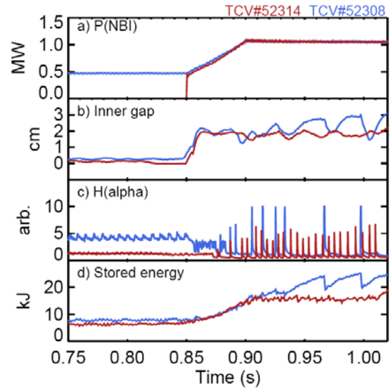
FIG. 4. (a) NBH power, (b) inner gap, (c) H_{\alpha} emission, (d) stored energy in two shots with and without L-mode pre-heating. (Reproduced from [10].)
