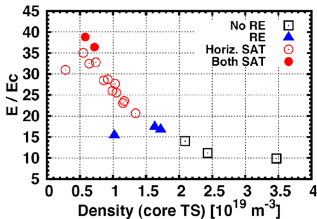
FIG. 9. Classification of runaway-electron discharges vs central density and normalized toroidal electric field, based on signals from heavily shielded HXR detectors: no RE = no signal, RE = finite signal, Horiz. SAT = midplane detector saturated, Both SAT = midplane and top detectors saturated. (Reproduced from [36].)
