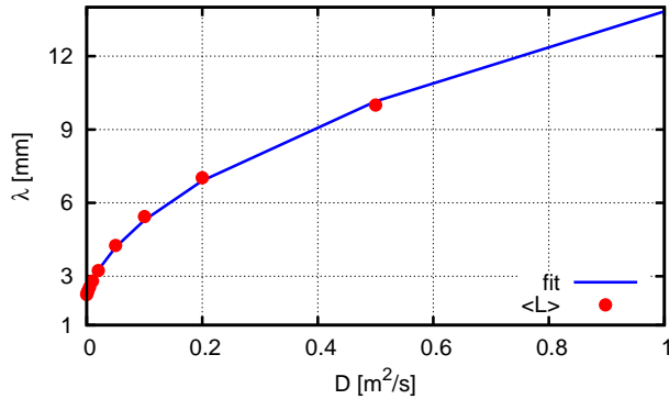
FIG. 11 (Color online) Dependence of \Lambda on the additional particle diffusion characterized by D_{\perp} . The points in red are the \theta -averaged values \langle |\partial \ln n / \partial r|^{-1} \rangle as found in Fig. 10 from the numerical solution of the 2D model. The blue line represents a fit of the form \Lambda_0/2 \left( 1 + \sqrt{1 + D_{\perp}/D_*} \right) motivated by the 1D estimate Eq. 33 with fit parameters \Lambda_0=2.27 mm and D_*=8.08\cdot 10^{-3} m 2 /s.
