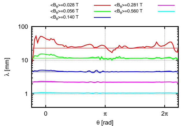
FIG. 9 (Color online) Dependence of \Lambda on the poloidal magnetic field \hat{B}_\theta . Shown are the profiles of the inverse logarithmic derivatives |\partial \ln n / \partial r|^{-1} overlaid by straight lines representing the results of Eq. 22 for \Lambda .
