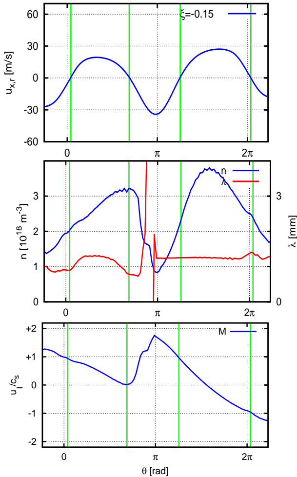
FIG. 7 (Color online) Simulation for the parameters chosen for Fig. 3 but with reversed toroidal magnetic field. From top to bottom: profiles of the radial physical component of the drift velocity \mathbf{u}_x , the density n and Mach number vs poloidal angle \theta for the magnetic field configuration with \xi=-0.15 . The green lines label the points where u_x^r=0 . Additionally the center plot includes the profile of the decay length \Lambda given by the numerical values of |\partial \ln n / \partial r|^{-1} .
