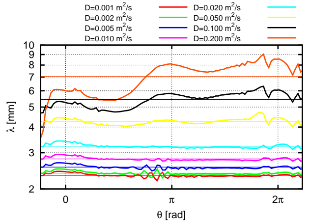
FIG. 10 (Color online) Dependence of \Lambda on the additional particle diffusion characterized by D_{\perp} . Shown are the profiles of the inverse logarithmic derivatives |\partial \ln n / \partial r|^{-1} overlaid by straight lines representing its respective \theta -averaged value.
