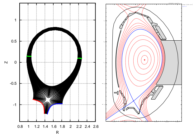
FIG. 1 Model geometry for ASDEX like magnetic field based on the conformal mapping presented in the Appendix A. On the left the computational domain (with reduced number of grid points to for clarity) is shown for R_0=1.65 m, h=1.2 m and rotation angle \xi=-0.15 . The points in red label the inner target ( \theta=-0.7 ), the points in blue the outer target ( \theta=6.98 ). The separatrix is located at r=h and 0 \leq \theta \leq 2\pi . The X-point is located at \theta=0 and \theta=2\pi , respectively. The right figure shows the equilibrium reconstruction of ASDEX Upgrade shot No. 32291 at t=2 s serving as a template for the conformal map in the left figure.
