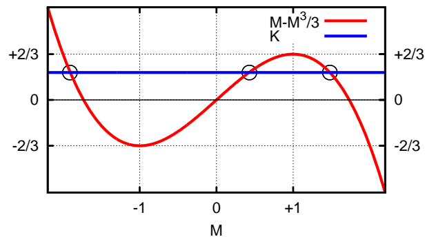
FIG. 5 (Color online) Illustration of a graphical solution of Eq. 19. If |K| < 2/3 three solutions exist (example K = 0.4 labeled by circles). For |K| = 2/3 two solutions exist and for |K| > 2/3 only a single real solution is possible.
