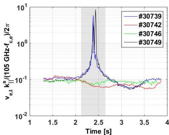
Figure 10. Time traces for the quantity v_{\parallel}k_{\parallel}^s/(\omega^s - s\omega_c) in the CTS measurement volume using the electron thermal velocity for v_{\parallel} and setting s = 1 . The shaded gray area marks the approximate time range where we find significant discrepancies between CTS and CXRS ion temperature measurements in discharges #30739 and #30749.
