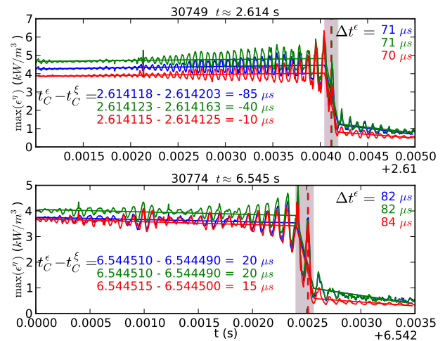
Figure 11: Time traces of the absolute value of SXR maximum for 2 crashes (with same 3 regularisations as in Fig. 3). The relative time evolution is robust and can be used to define a reference time t_C^\epsilon and a crash duration \Delta t^\epsilon from the best fit of 3 lines.
