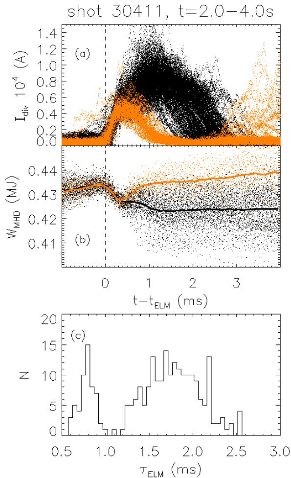
Figure 2. ELM synchronized time traces of (a) divertor currents and (b) stored energy. (c) histogram of the ELM duration calculated has the FWHM of the divertor current from frame (a). The orange color corresponds to the ELMs with \tau_{\text{ELM}} < 1.1 ms and the black color to the ELMs with \tau_{\text{ELM}} > 1.1 ms. The continuous lines in frame (b) highlight the conditional average of the stored energy for short (orange) and long ELMs (black). Data correspond to a stationary phase between t=2-4 s at P_{\text{NBI}}=5 MW with no N seeding.
