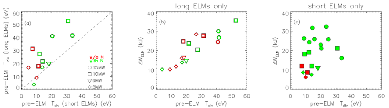
Figure 14. (a) log ELMs pre-ELM T_{div} versus short ELMs pre-ELM T_{div} . Only stationary intervals characterized by the presence of both long and short ELMs are considered. (b) ELM energy losses of long ELMs versus the corresponding pre-ELM T_{div} . (c) ELM energy losses of short ELMs versus the corresponding pre-ELM T_{div} .
