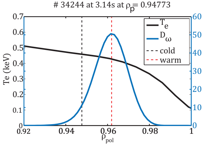
Figure 2. # 34244 at t = 3.14 s: Midplane edge channel of f = 110.27 GHz of the ECE diagnostics. The cold resonance position, determined by the magnetic field strength, is shown as black dashed line. A birthplace distribution of the observed intensity ( D_\omega ) is shown in blue. The peak of the ( D_\omega ) represents a warm resonance for a respective channel. The T_e profile is shown in a solid black line.
