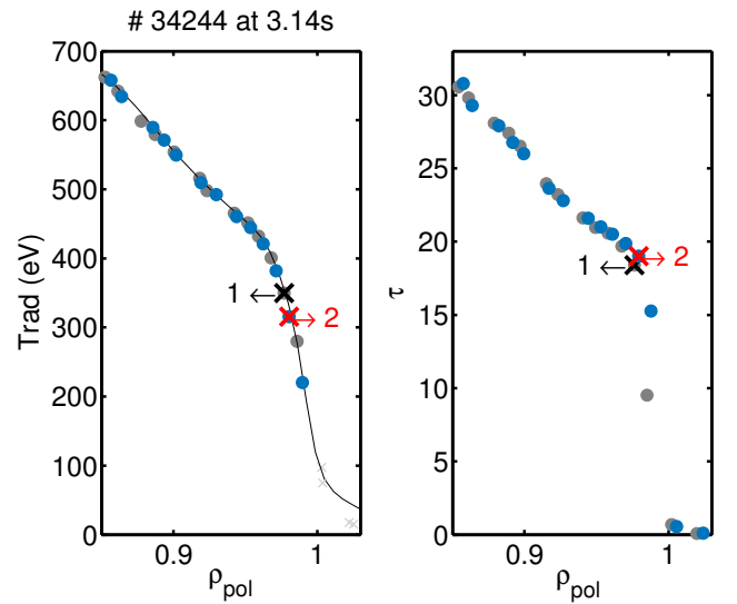
Figure 5. a) Modeled T_{\text{rad}} profile of the ECE system shown against warm resonances of respective channels. The dark gray circles correspond to a case with background density profile (1), and the blue circles correspond to a case with added Gaussian (2). Gray crosses are showing channels with cold resonances outside the separatrix. The channel analyzed in this manuscript is labeled as 1 for the case without perturbation, and 2 with perturbation present. b) Optical depth for ECE channels for case 1 and 2, marked as gray and blue circles, respectively.
