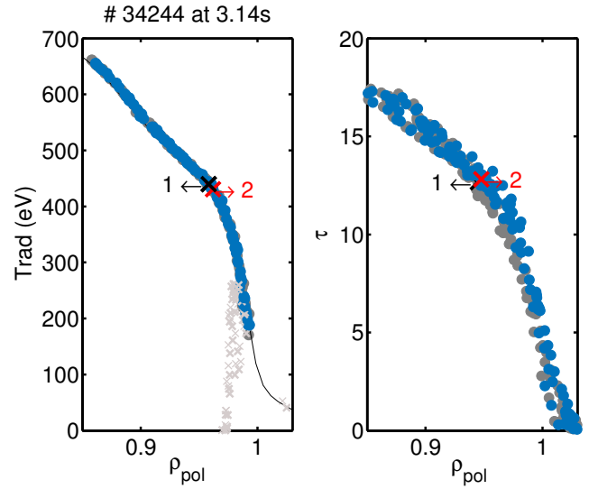
Figure 4. a) Modeled T_{\text{rad}} profile of the ECEI system shown against warm resonances. The dark gray circles correspond to a case without density perturbation (1), and the blue circles correspond to a case with the density perturbation (2). Gray crosses are showing channels with cold resonances outside the separatrix. The channel analyzed in this manuscript is labeled as 1 for the case without perturbation, and 2 with perturbation present. b) Optical depth for ECEI channels for case 1 and 2, marked as gray and blue circles, respectively.
