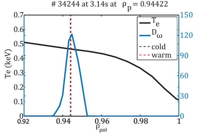
Figure 2. # 34244 at t = 3.14 s: Midplane edge channel of f = 110.27 GHz of the ECE diagnostics. The cold resonance position, determined by the magnetic field strength, is shown as black dashed line. A birthplace distribution of the observed intensity ( D_\omega ) is shown in blue. The peak of the ( D_\omega ) represents a warm resonance for a respective channel. The T_e profile is shown in a solid black line.
