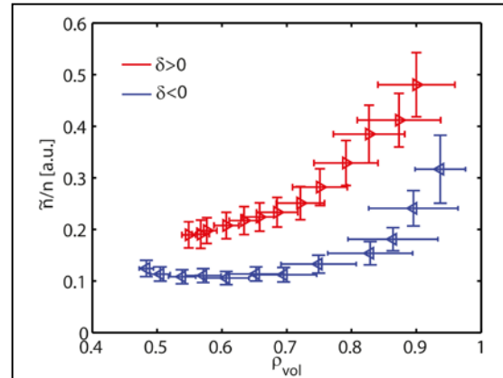
FIG. 6. Density fluctuation amplitude profile measured by tPCI in two plasmas with edge triangularity +0.5 and -0.3, respectively, with 0.45 MW central ECRH. (Reproduced from [56].)
