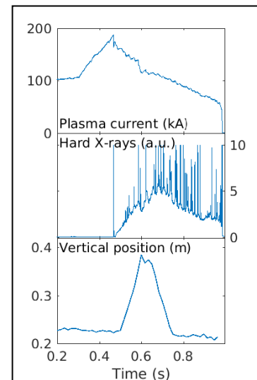
FIG. 2. Demonstration of RE ramp-down with the Hybrid Fast Controller with vertical 11-cm sweep. Plasma current (top), hard X-ray emission (middle), vertical position of magnetic axis (bottom). (Adapted from [22].)
