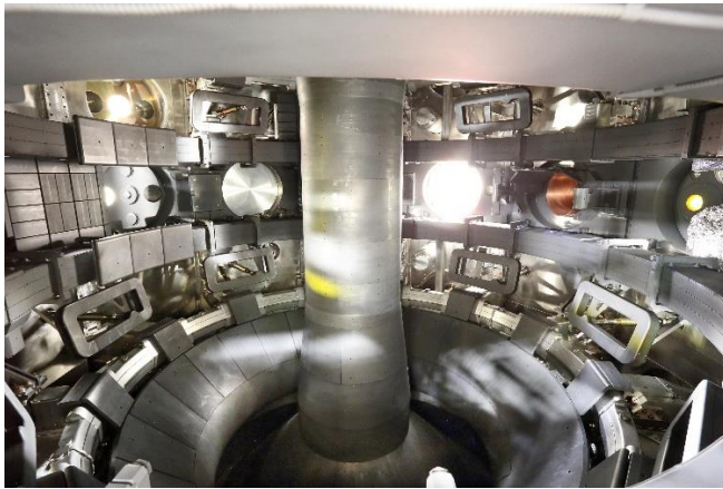
Figure 8: Photograph of the completed interior of MAST Upgrade prior to being pumped down.
