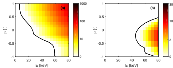
FIG. 4. Exponentially growing penalty function \xi above what is neoclassically expected by the TRANSF simulation (a) and in the null-measurement region (b).
