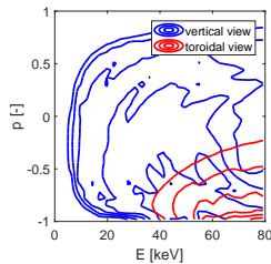
FIG. 2. (E, p) -space interrogation regions related to the experimentally accessible wavelength ranges in the toroidal ([660.2 – 662.25] nm) and vertical ([650.96 – 654.5] nm) views.
