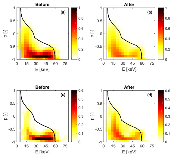
FIG. 6. Reconstructions of the FIDASIM (a)-(b) and experimental (c)-(d) signals before and after the sawtooth crash using \lambda_1 = 5 \times 10^9 and \lambda_0 = 1 . All plots are normalized by the same factor as in Figure 3.
