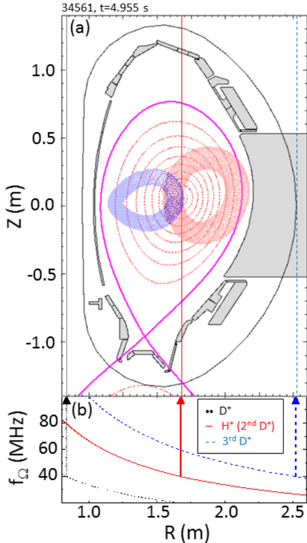
FIG. 6. (a) Frequency matched radial positions of the fundamental deuterium (dotted black line), the fundamental hydrogen and the 2 nd harmonic deuterium (solid red line), and the third harmonic deuterium (dashed blue line) cyclotron frequencies in discharge #34561. (b) The radial profiles of the above-mentioned frequencies calculated using a self-consistent kinetic equilibrium during core ICE. The two orbits in (a) correspond to barely confined fusion proton orbits. The orbit protruding to the HFS is for the counter-current pitch value of -0.72. The orbit protruding to the LFS is for the co-current pitch value of 0.45. Both orbits originate at the magnetic axis.
