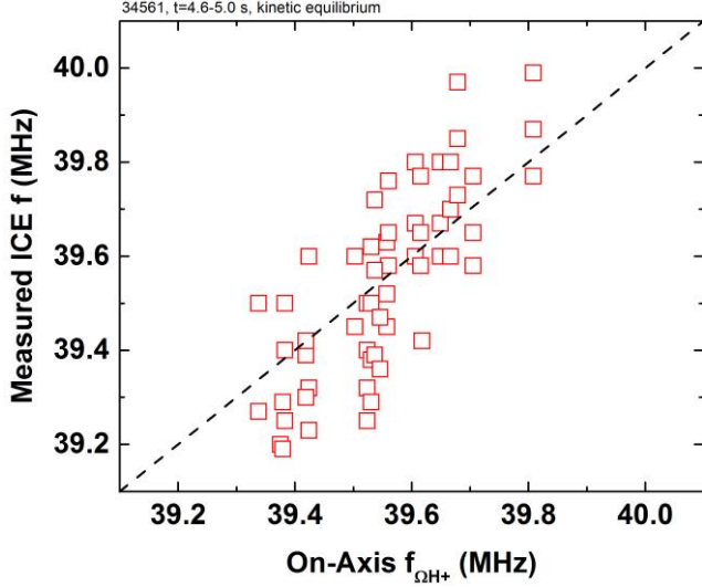
FIG. 4. Correlation between the measured ICE frequency and the estimated fundamental hydrogen cyclotron frequency on the magnetic axis. The data are from the last 6 NBI beam blips in discharge #34561 (Fig. 3 (i)-(l)), after the disappearance of a brief ELM-free H-mode. The dashed line corresponds to equality of the ICE and on-axis hydrogen cyclotron frequencies.
