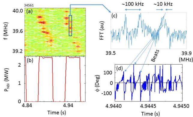
FIG. 5. Details of the measured ICE spectra (a) during the last two NBI pulses (b) in discharge #34561 (Fig. 4). The effect of frequency splitting at levels of \sim 100 kHz and \sim 10 kHz (c) and the confirmation of the fine \sim 10 kHz frequency splitting via a phase measurement (d). The periodic modulations of the measured phase are a result of the beatwave pattern formed by several closely spaced frequency peaks.
