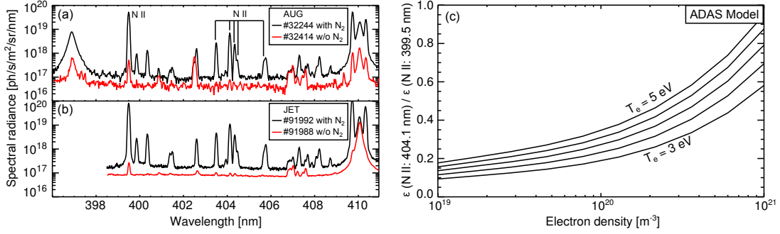
Figure 1: Time averaged spectrum measured in the (a) ASDEX Upgrade and (b) JET divertor with (black) and without (red) \text{N}_2 seeding. The ratio of two N II multiplet lines from a collisional-radiative model is shown for a range of electron temperatures and densities in (c).
