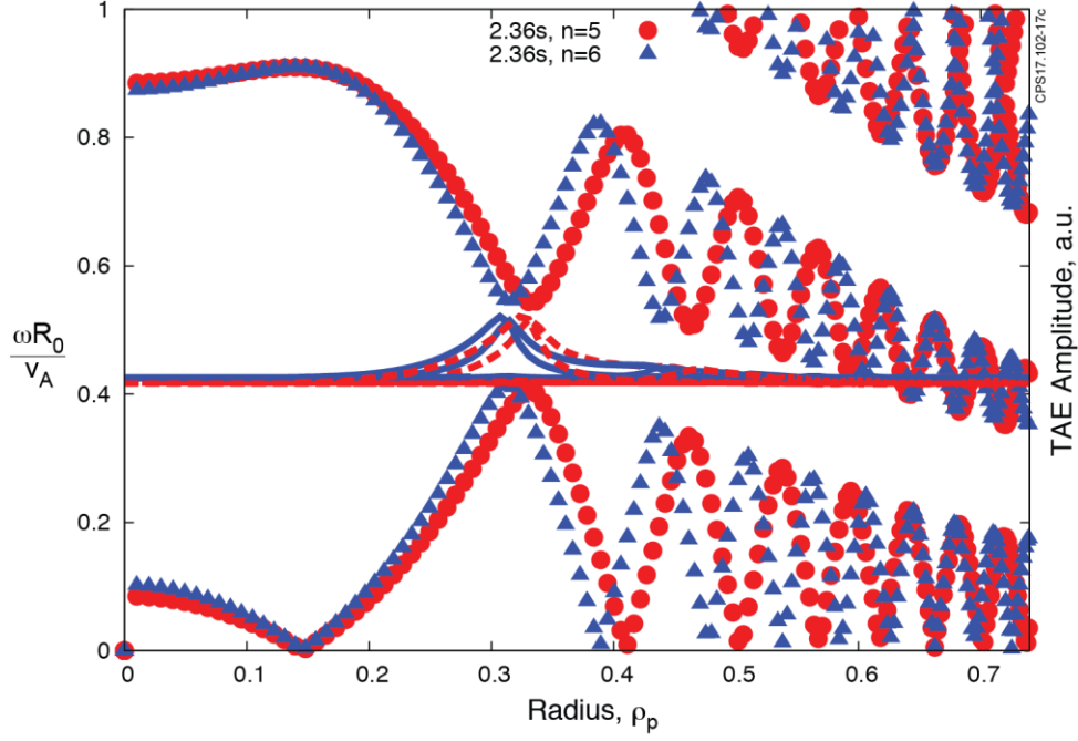
Figure 16. Core-localised TAEs with n=5 (solid blue line) and n=6 (broken red line) computed with the LIGKA code. Alfvén continua for n=5, 6 are shown with red circles and blue triangles respectively.
