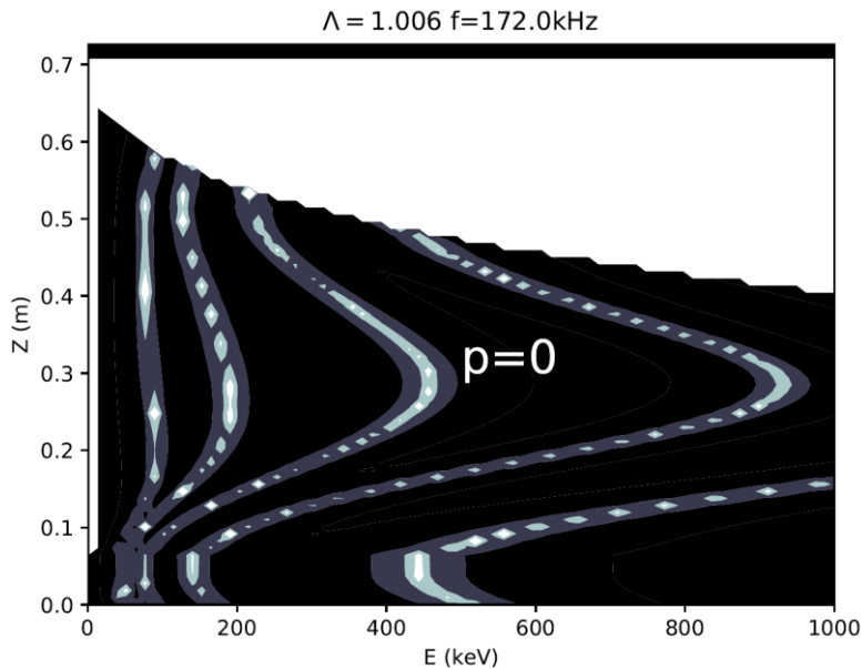
Figure 17: Resonance map for ICRH-driven TAEs with n=5 in AUG discharge #33150, t \sim 2.4 s. The resonance lines are shown in white for p=0, \pm 1 , and the most efficient resonance line with p=0 is marked.
