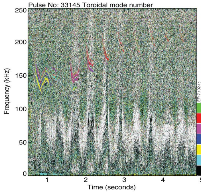
Figure 6 (colour online). Phase magnetic spectrogram showing toroidal mode numbers of the excited TAEs in Figure 5.
