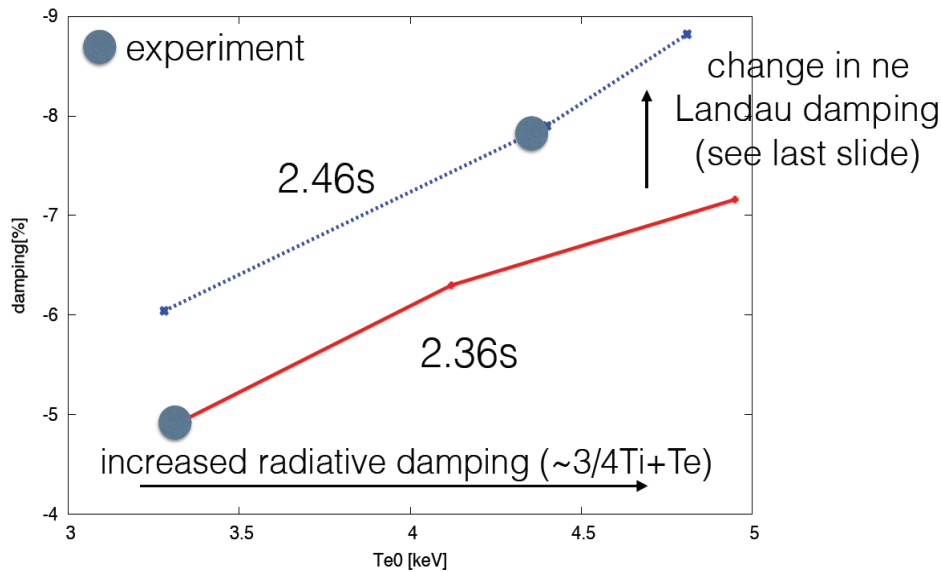
Figure 18. With ECRH applied at \rho_p \approx 0.3 , both ion Landau damping and radiative damping increase as shown by the LIGKA modelling.
