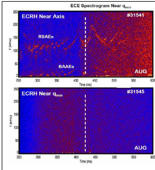
Figure 3. ECE data on AEs excited in two AUG discharges with ECRH applied near magnetic axis (top) and near q_{\min} (bottom) [4]. .
