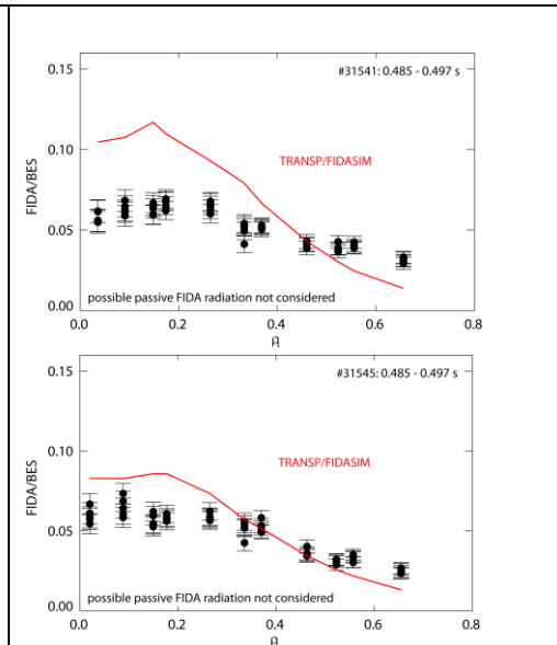
Figure 4. Radial profiles of NBI ions measured with the fast ion D_{\alpha} (FIDA) diagnostics and computed with the TRANSP code in the two comparison discharges. Here, \rho_t = (\psi_t / \psi_t(a))^{1/2} is radial coordinate associated with toroidal magnetic flux \psi_t .
