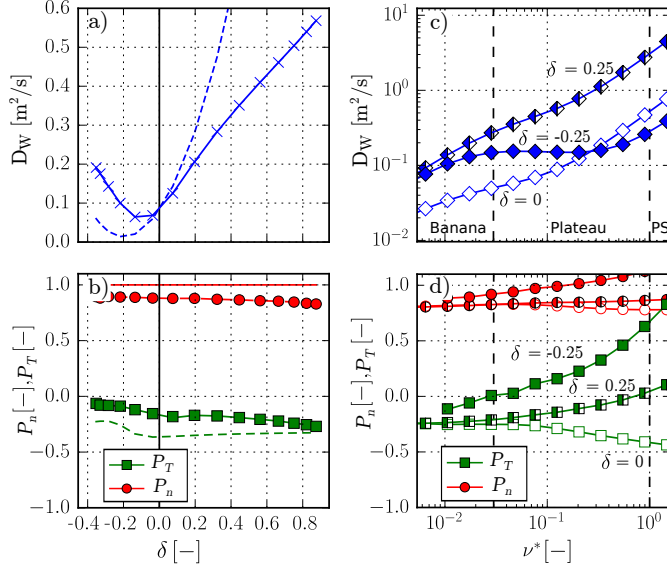
Figure 2. Neoclassical tungsten flux from the NEO code decomposed according to formula (10) scanned over a - b poloidal asymmetry and c - d normalized bulk ion collisionality \nu^* , W collisionality is Z_W^2 = 2045 times higher. a) Full line corresponds to D_W from NEO at r/a = 0.3 ( \varepsilon = 0.1 ), while the dashed line is an analytical model for the PS regime [18] normalized with respect to the D_W(\delta = 0) . b) Peaking factors P_T (green) and P_n (red) from NEO compared with analytical model for the PS regime (dashed lines). To avoid a non-physical singularity in the approximation at \delta/\varepsilon = -2 , a classical diffusion was included.
