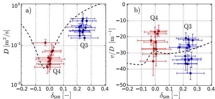
Figure 9. The neoclassical value of the transport coefficient (dashed lines) for the discharge #32324 at \rho_{\text{tor}} = 0.12 compared with the experimentally measured values (dots) in the Q3 phase (blue) and the Q4 phase (red) for the diffusion coefficient D a) and the drift coefficient v/D b).
