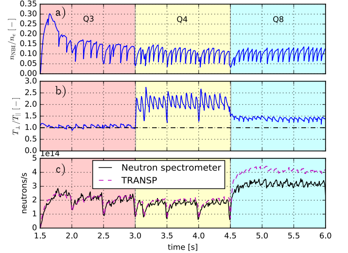
Figure 4. Temporal evolution of on-axis a) fast particles fraction n_{\text{NBI}}/n_e , b) temperature anisotropy T_\perp/T_\parallel and c) total neutron flux as calculated by TRANSP for the discharge #32566, compared with neutron spectrometer measurement [46].
