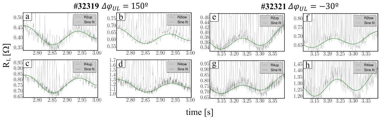
Figure 3. Loading resistances of the 3-strap antennas feeding lines in discharges #32319 (a-d) and #32321 (e-h). R2up designates a2, upper feeder and so on. A sine fit (green) is added to better visualize the base variation of the loading.
