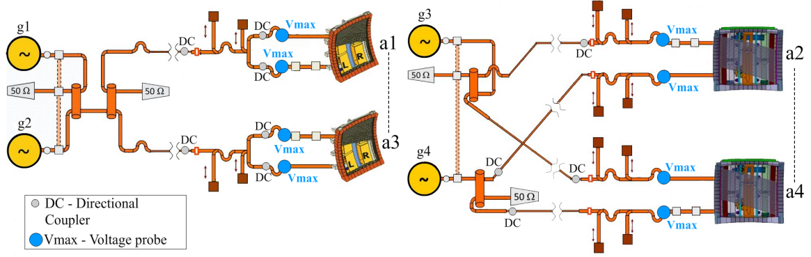
Figure 2. ASDEX Upgrade ICRH system. RF generators are marked from g1 to g4. Antenna 1 (a1) and antenna 3 (a3) are 2-strap antennas, antenna 2 (a2) and antenna 4 (a4) are 3-strap antennas.
