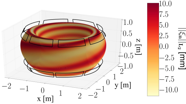
Figure 1. NEMEC 3D equilibrium of shot #32091 at t=2.9 s where the saddle coils have been artificially supplied with 5kAt and \Delta\varphi_{UL} = -140^\circ for this simulation. The normal displacement of the last closed flux surface \|\xi_n\|_{L2} is color-coded.
