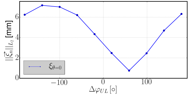
Figure 4. NEMEC LFS midplane normal displacement vector norm vs. different \Delta\varphi_{UL} .
