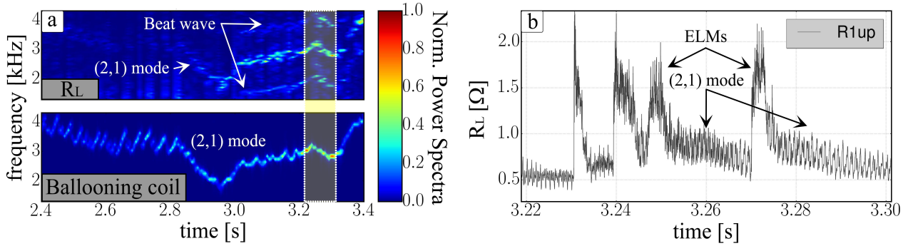
Figure 5. Discharge #32749. (a) Spectrograms of the loading resistance measured in the upper feeder of a1 and Ballooning coil for reference. The signature of an MHD mode is clearly visible on both signals. (b) Loading resistance during the highlighted time region.
