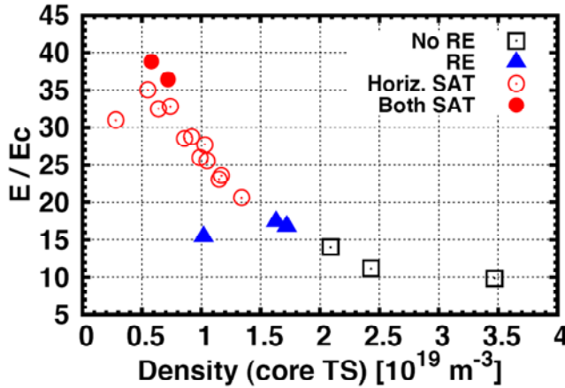
FIG. 8. Classification of runaway-electron discharges vs central density and normalized toroidal electric field, based on signals from heavily shielded HXR detectors: no RE = no signal, RE = finite signal, Horiz. SAT = midplane detector saturated, Both SAT = midplane and top detectors saturated. (Reproduced from [36].)
