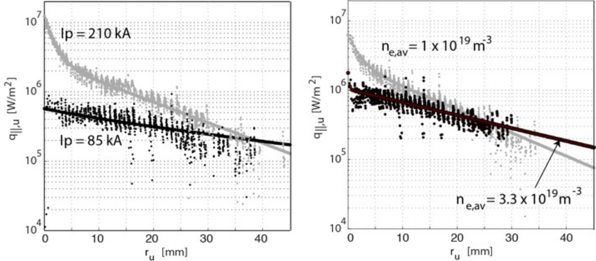
FIG. 7. Profiles of parallel heat flux to the target mapped to the outboard midplane for inboard limited plasmas for (left) two current values at line-averaged density 1.7 \times 10^{19} \text{ m}^{-3} and (right) two density values at a plasma current of 140 kA. (Reproduced from [28].)
