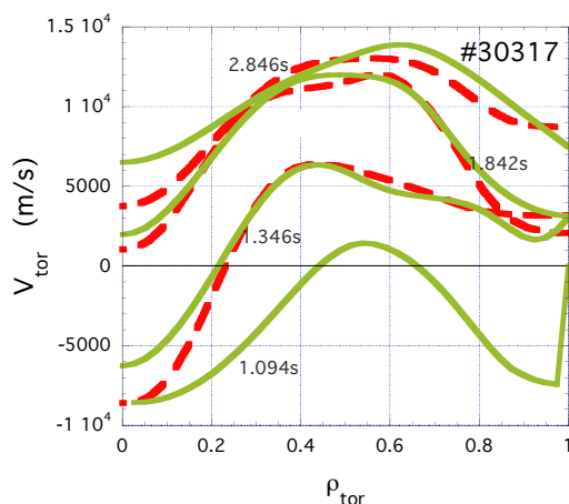
Figure 5: as figure 4 for AUG #30317 discharge. The ratio of the T_{\text{pump-out}} / S_{EC} \ll 10^{-3} so the effect is due to the turbulence effect.
