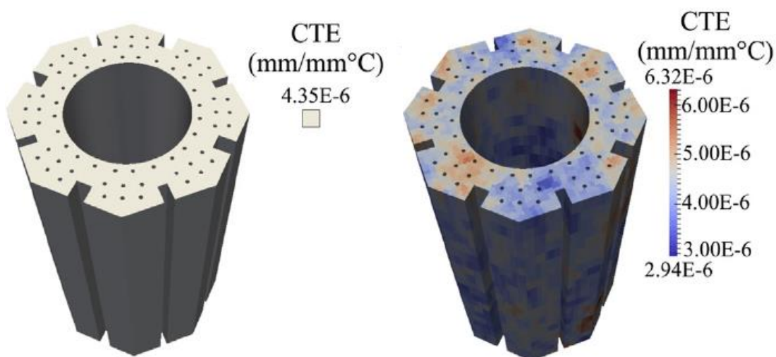
Figure 4. Coefficient of thermal expansion for a) the deterministic model and b) one stochastic realisation [34].
