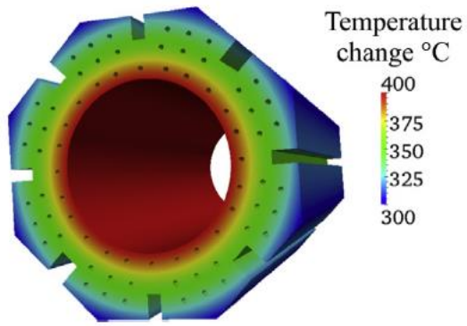
Figure 5. Temperature profile used to represent heating from fuel rod in the centre [34].
