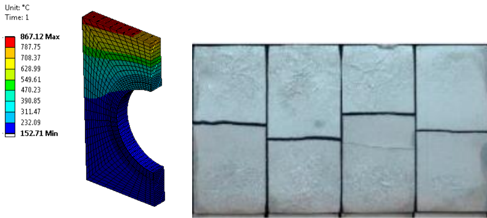
Figure 2. Fusion heat exchanger component having been tested a) computationally where results are identical each time and (isometric view) [23] b) experimentally where failure location changes due to range of variations (plan view) [24].
