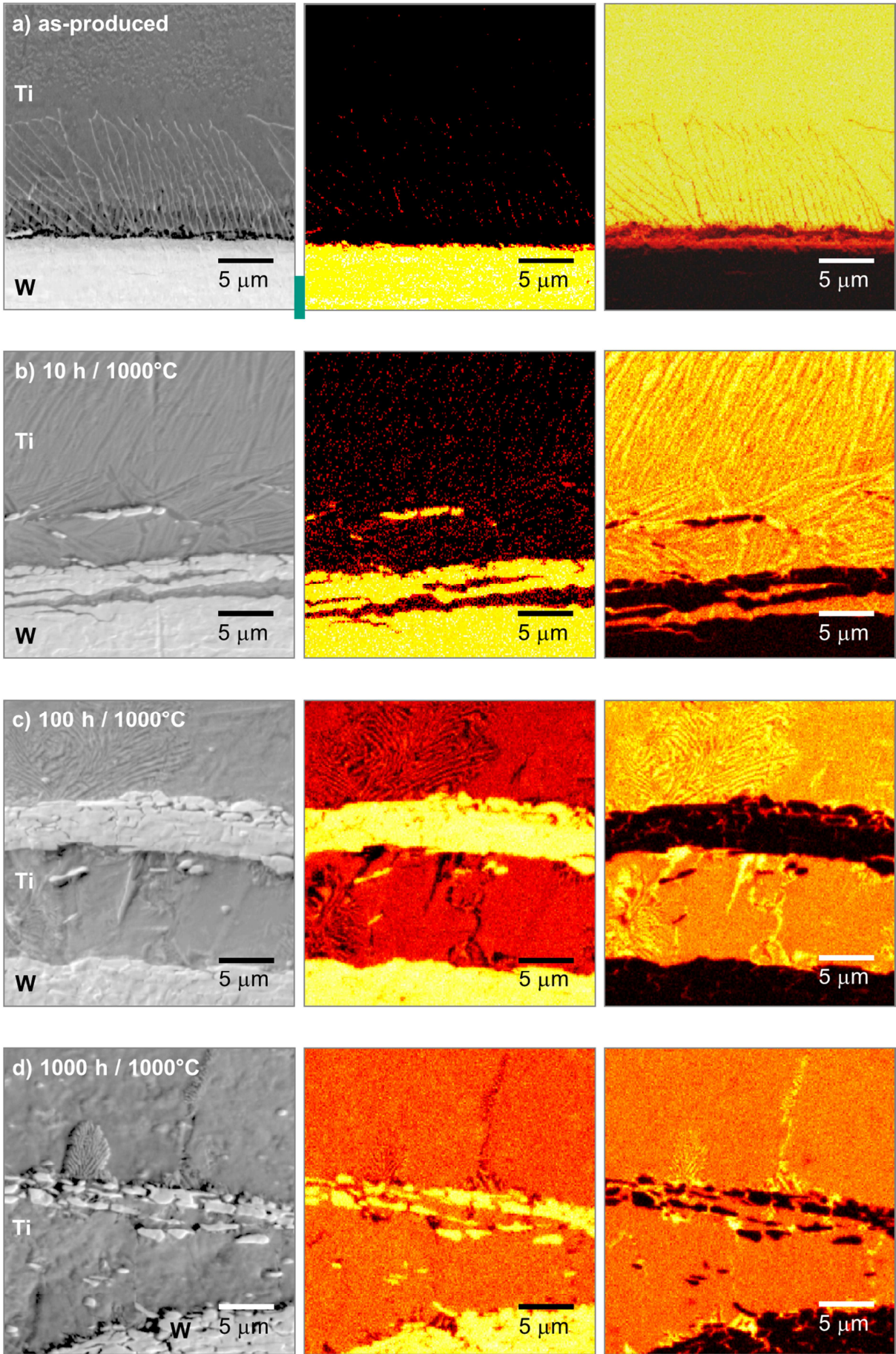
Fig. 7. AES analyses of tungsten titanium interfaces in different ageing conditions.
