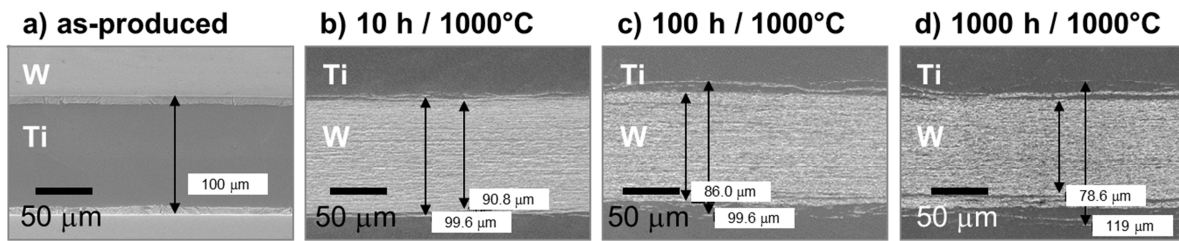
Fig. 8. SEM analyses of the movement of the interface. From left to right: (i) as-produced, (ii) annealed for 10 h at 1000°C, (iii) annealed for 100 h at 1000°C, and (iv) annealed for 1000 h at 1000°C.
