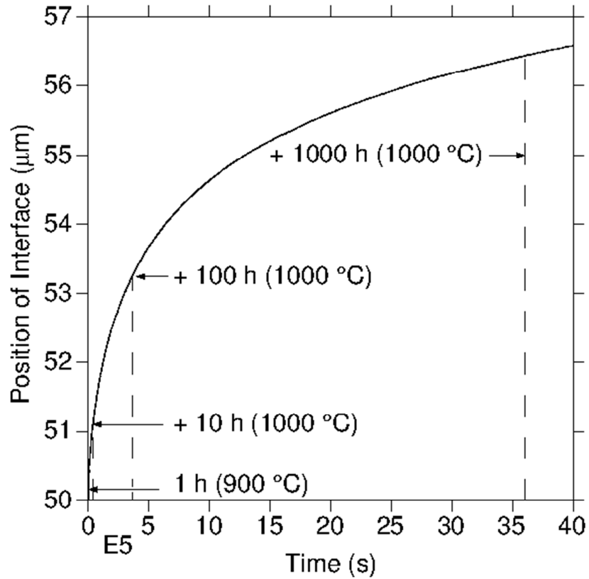
Fig. 6. Calculated interface position between the titanium and tungsten sheets during the heat treatment.
