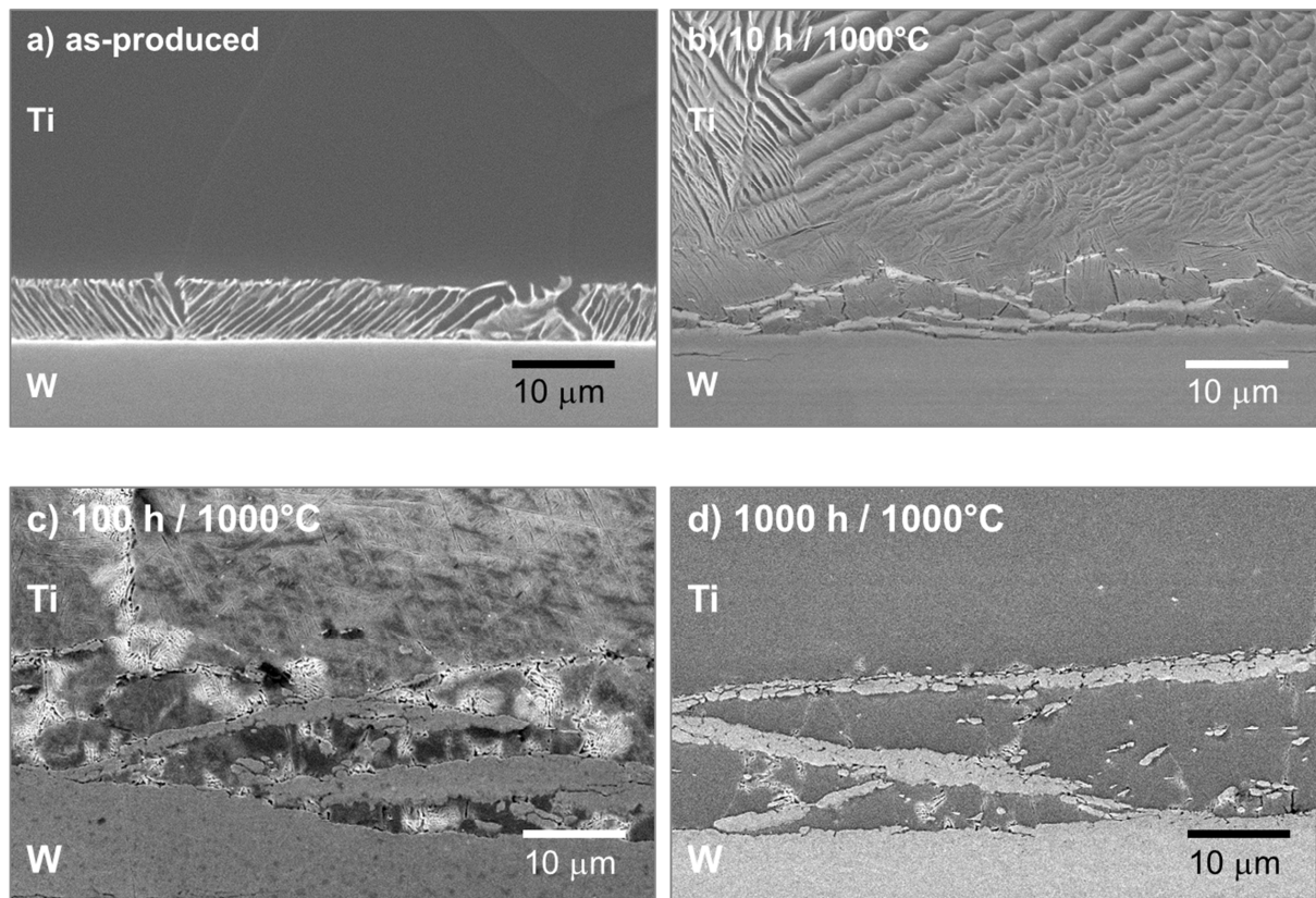
Fig. 2. Scanning electron microscope (SEM) analyses of the W-Ti interface in the four conditions analysed in this paper. These are (i) as-produced, (ii) annealed for 10 h at 1000°C, (iii) annealed for 100 h at 1000°C and (iv) annealed for 1000 h at 1000°C.
