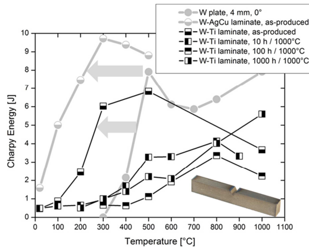
Fig. 10. Results of the Charpy impact tests. The dissipated energy is plotted against the test temperature. All samples were oriented in L-S direction.
