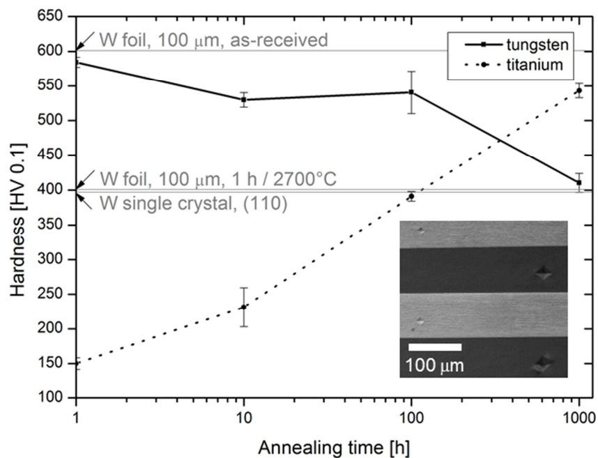
Fig. 11. Vickers hardness HV0.1 plotted against the annealing time. The W-Ti laminates were produced by diffusion bonding at 900°C for 1 h and then annealed at 1000°C for 10 h, 100 h, and 1000 h.
