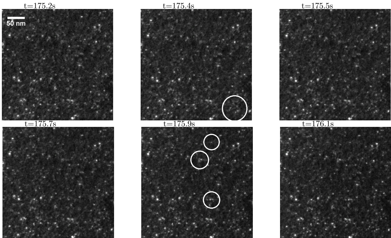
Fig. 1: A sequence of snapshots taken over 1s irradiation with 400keV ions showing the space- and time- correlated appearance of nano-scale defects. Contrary to the case in iron, where the defects produced at low fluence are very small [6], individual cascade events in tungsten produce correlated clusters of defects up to 10nm diameter, which appear at full brightness in a single frame and then do not subsequently evolve.
