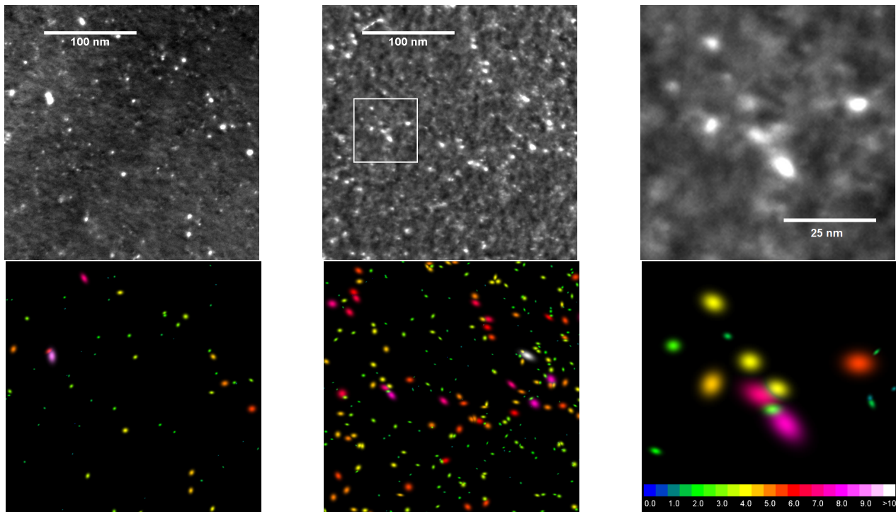
Fig. 2: Defect clusters produced in collision cascades of tungsten. Top: Weak-beam dark-field imaging ( g = 200 , \sim 3.8g ) of defect clusters in (left, centre) 150 keV, 400 keV W^+ ion irradiated samples, up to a fluence of \sim 10^{16} W^+ m^{-2} at 30 K. Top right: an enlarged view showing spatially correlated defects. Bottom: computed generated interpretations of the position and size of the defects in the images above. Defects are coloured according to their maximum diameter, with the scale (in nm) given in the coloured bar.
