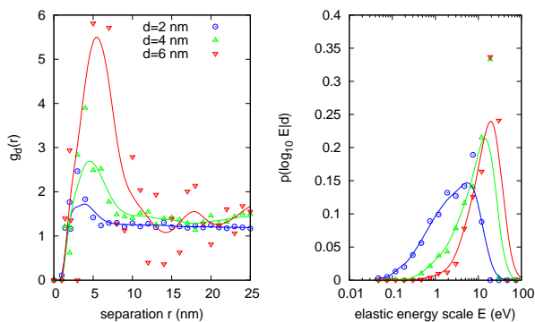
Fig. 5: Analysis of spatial correlations of defect clusters obtained from micrographs of 400 keV W^+ irradiated tungsten at 30 K. (a) The radial pair distribution function g_d(r) is plotted against the separation distance r for defects with diameters d > 0, 2, 4, 6 nm. The solid lines are to help guide the eye. The dashed lines are the expected curves if the positions of the defects are initially randomly placed within cascades (see text). (b) A characteristic elastic energy scale computed from the size and estimated separation of the loops (see text).
