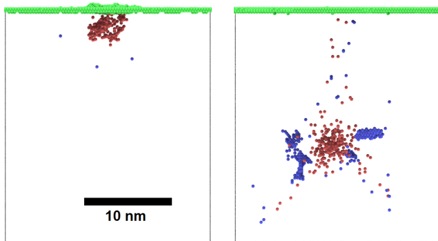
Fig. 4: Typical final state configurations of (left) 30keV and (right) 150keV collision cascades in tungsten foil simulated using MD. Red spheres denote vacant lattice sites, blue spheres are self-interstitials and green are surface atoms.
