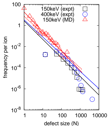
Fig. 3: Histogram of defect size ( N ) for both experiments and MD simulations. Loops smaller than 1.5\text{nm} were difficult to distinguish from the background image intensity fluctuations; the smallest size experimental bin is the accumulated frequency for diameter d < 1.5\text{nm} . The dashed line shows the cluster power law found for 150 keV cascades in bulk tungsten [11]. The histograms are normalized so that the area under the curves matches the total number of defects counted.
