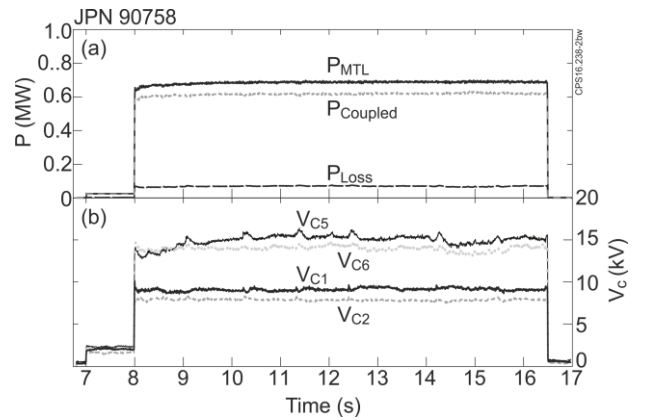
Fig. 2. Example of operation in CD phasing at 33MHz (upper half) on L-mode plasma. (a) MTL power, coupled power and losses (b) voltage at capacitors. The high mutual coupling between RDLs in CD operation leads to voltage imbalance between the straps of the two RDLs ( V_{C5} \sim V_{C6} > V_{C1} \sim V_{C2} ).
