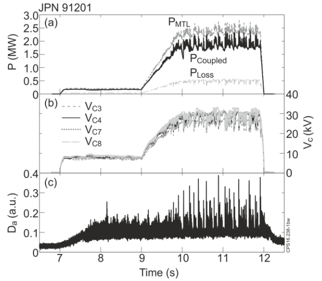
Fig. 1. Example of operation in dipole phasing at 29.2MHz (lower half) on ELMY plasma. (a) MTL power, coupled power and losses (b) voltage at capacitors (c) D-alpha.
