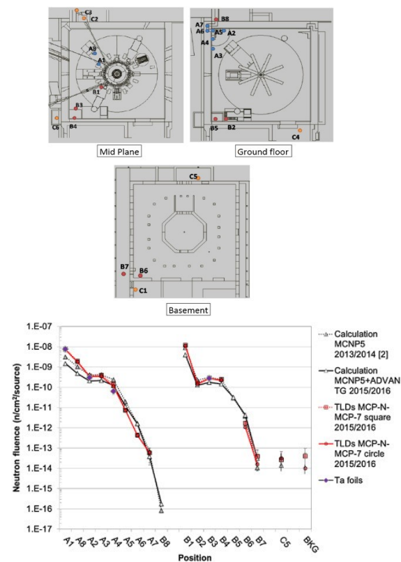
Figure 5. Calculated and measured neutron fluence with TLDs and Ta foils (from [7]).
