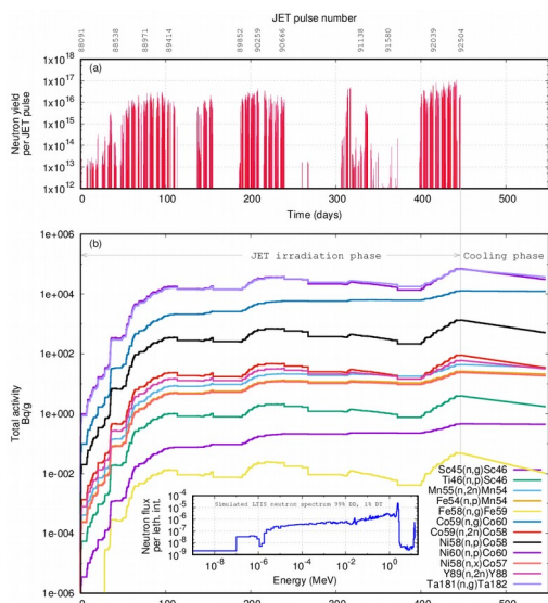
Figure 7: (a) JET neutron yield per pulse between 27/08/2015 and 15/11/2016; (b) Simulated specific activities calculated over time for dosimetry foils located within the long-term irradiation station assembly, exposed to JET experimental campaigns calculated using FISPACT-II.
