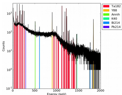
Figure 8: HPGc measurement taken from an Y foil 'CCFE1', showing the characteristic lines from Y-88 and also Ta-182, the latter isotope being measured due to Ta impurities in the Y foil.
