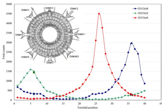
Figure 1. Fission chambers counts in 1200 s acquisition time as a function of the ^{252}\text{Cf} source position on central ring. The
