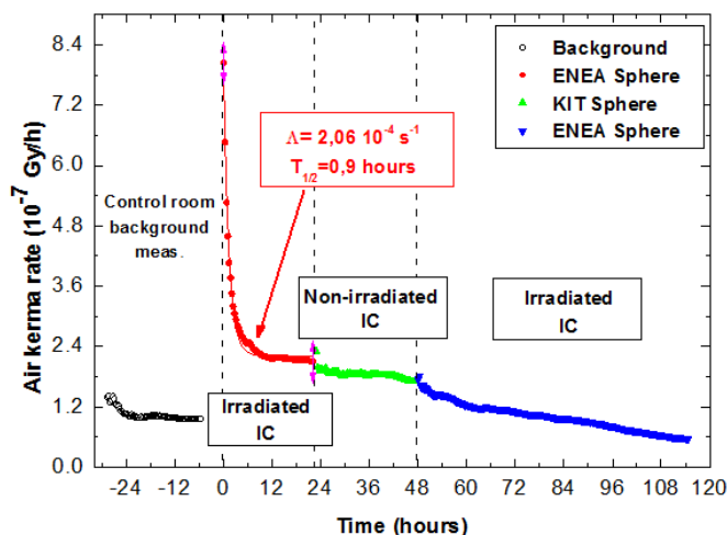
Fig. 4 Air kerma rate measured after the second irradiation test at FNG with the irradiated IC (i.e., ENEA IC 32002) and the non-irradiated IC (i.e., KIT IC 32002).
