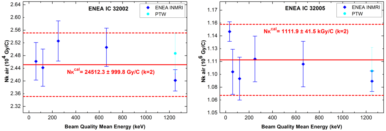
Fig. 1 N_{\text{Kair}} factors for the ENEA ICs 32002 (left) and 32005 (right) resulting from the INMRI (diamond-shaped points) and PTW (circle-shaped points) calibration. Error bars represent the expanded measurement uncertainty (coverage factor k=2 ). The 'equivalent' calibration factor N_{\text{K}}^{\text{cal}} is plotted as solid line; dashed lines represent the limits of the expanded uncertainty ( k=2 ) associated to N_{\text{K}}^{\text{cal}} .
