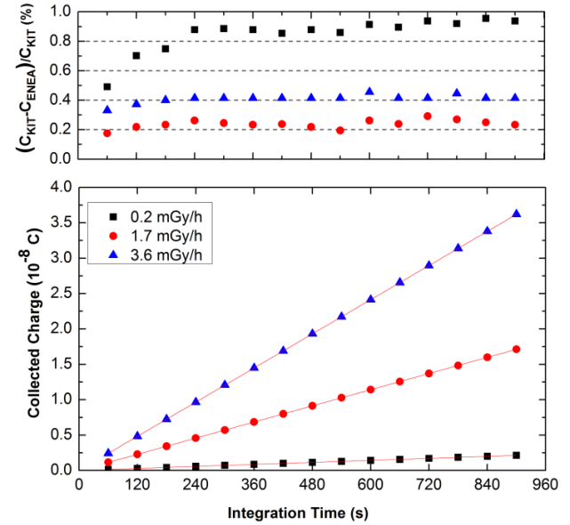
Fig. 3 Bottom: Collected charge measured with the ENEA dosimetry system at different dose rates (0.2, 1.7 and 3.6 mGy/h). Top: normalized difference of collected charge measured with the KIT and ENEA systems.
