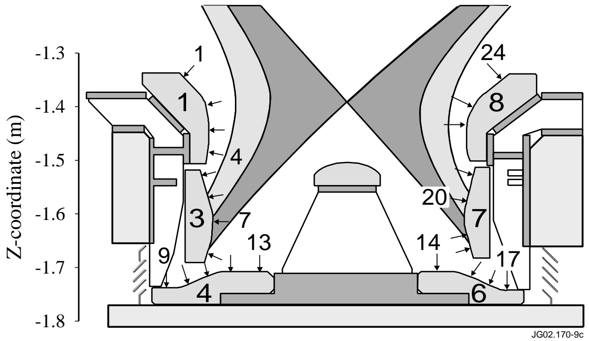
Figure 10: Poloidal cross-section of the Mk-IIIGB divertor, the flux deposition profiles and distribution of mechanical measurement points
