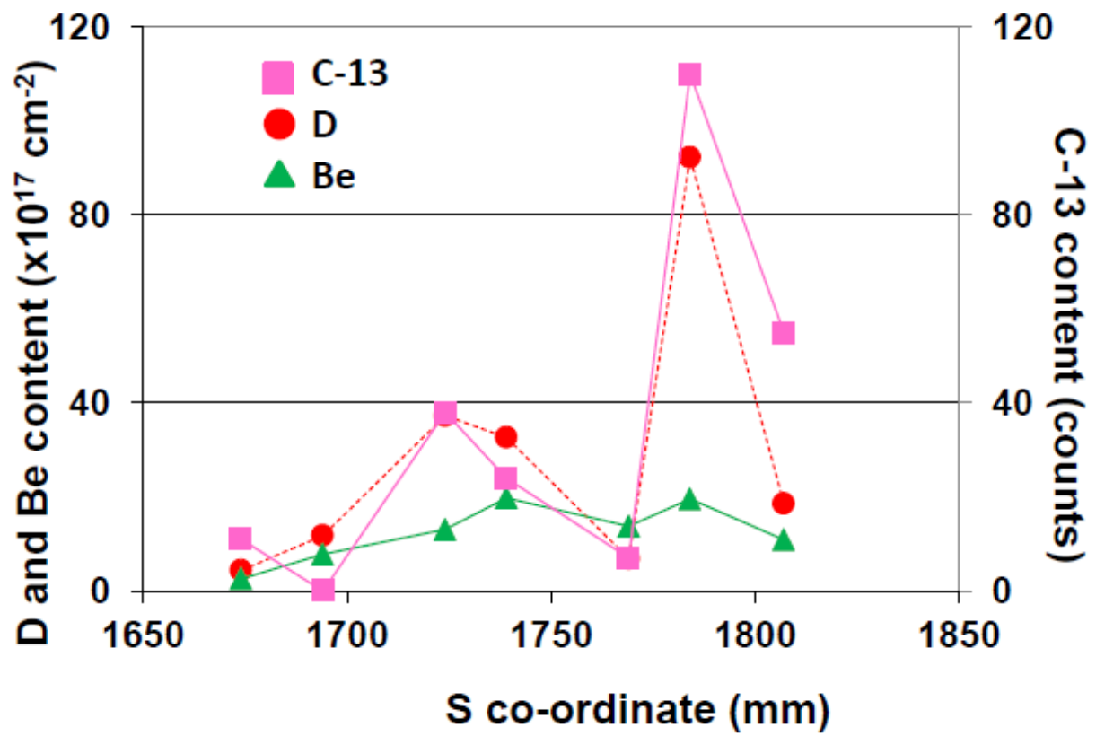
Figure 30: Levels of Be and D, and \text{C}^{13} counts, along Tile 7 (from bottom to top) measured by NRA
