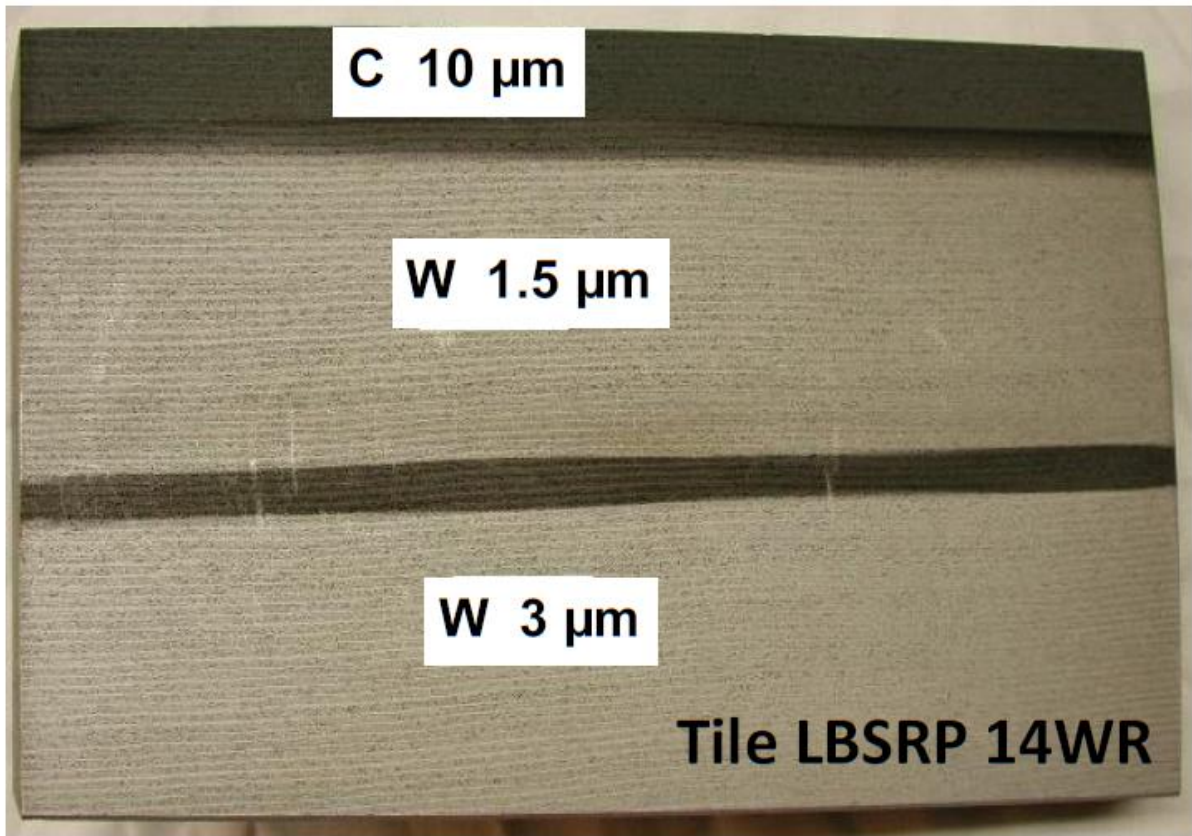
Figure 40: Tile LBSRP 14WR coated with two thicknesses of W and a 10 μm stripe of C (on a W interlayer), before mounting in JET in 2004
