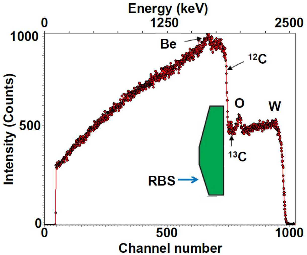
Figure 27: An RBS spectrum from the W stripe about one-third the way up the Tile 7 surface as shown in the sketch, after exposure in JET 2001-4
