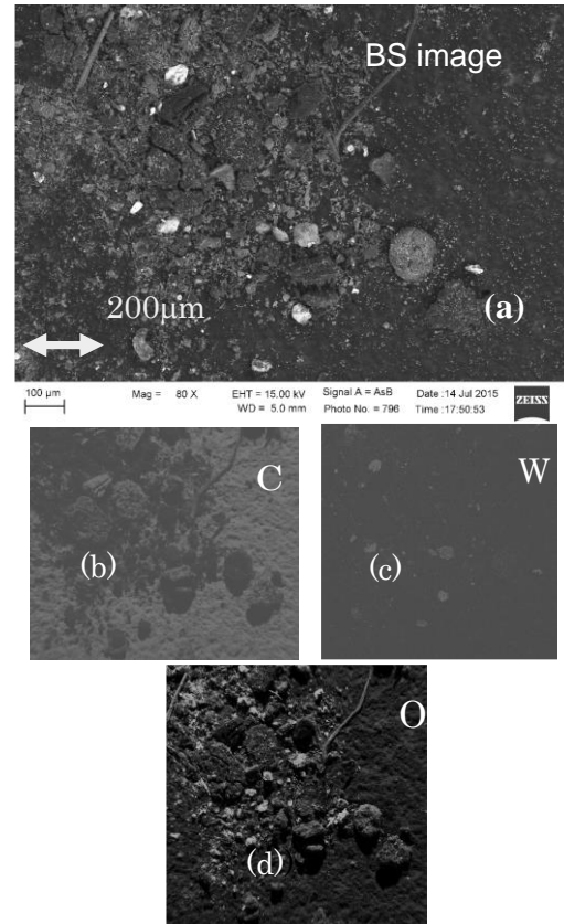
Figure.2 (a) Surface morphologies of overall dust particles measured by SEM / backscattering detector. (b)-(d) 2-D mapping images of C, W, O compositions measured by EDX. The same scale was used in SEM and EDX images.
