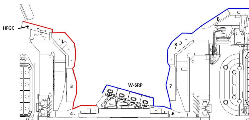
Figure.1 Schematic drawing of cross section of the divertor surface areas for dust vacuuming shown at the inner divertor in red and the outer divertor in blue. The masses of dust collected from the inner and outer divertor are 0.7 and 0.3 g, respectively [3].
