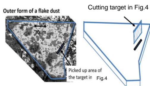
Figure.3 Surface morphology of a Be flake dust before FIB treatments. A hatching region is a picked up area of the target in Fig.4.
