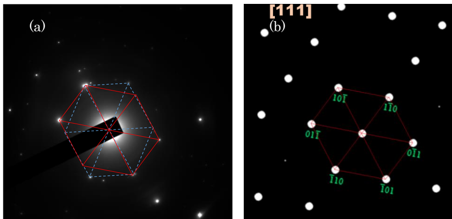
Figure.5 Diffraction pattern in the zone axis incident measured by TEM for (a) a Be flake dust as shown in Fig.3 and (b) reference data of metal beryllium.
