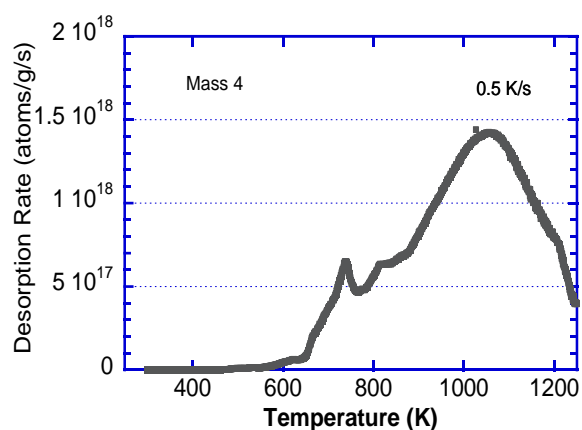
Figure.6 Thermal desorption spectrum for ILW dust particles.
