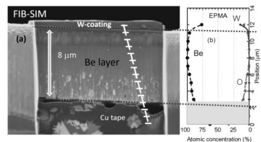
Figure.4 (a) Cross-section image of beryllium flake dust measured by SIM on FIB. A broken line shows measurement positions by EPMA. (b) An atomic concentration is measured by EPMA for the cross-section.
