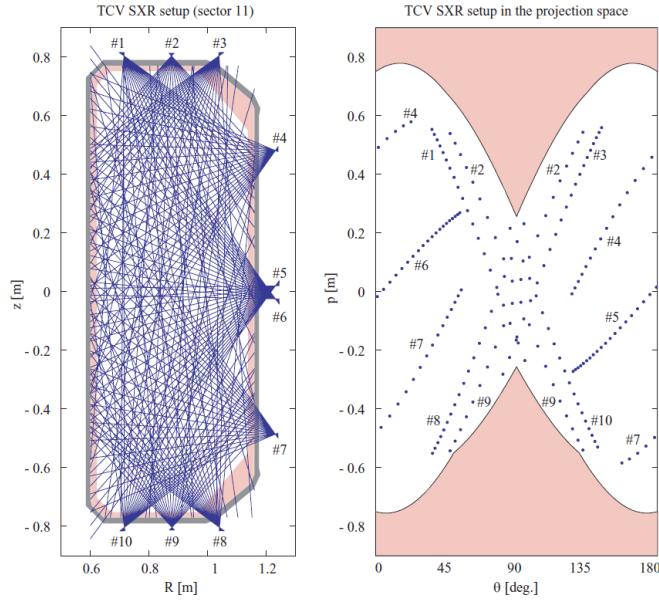
Fig. 1 The Soft X-ray tomography setup at tokamak TCV [3]. While number of the measured line integrated projections is rather high (left) the actual coverage in the projection space is still quite sparse (right).
