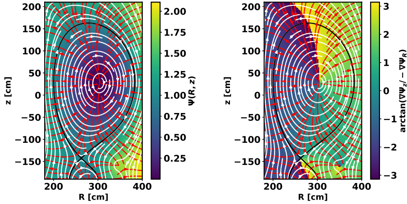
Fig. 5 Left: Two-dimensional plot of the normalised magnetic flux function \Psi_N(R, z) as reconstructed by EFIT at JET, including Last Closed Flux Surface in black (the value of the flux is normalised to the value at this contour). The red arrows mark the gradient of the \Psi function and the white arrows the perpendicular direction. Right: A similar plot of inverse tangent of the direction perpendicular to the gradient of \Psi . This function is then used in order to find proper weights for the derivative (smoothing) matrix with preferential smoothing along the magnetic flux contours.
