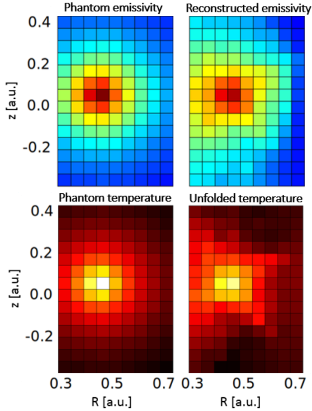
Fig. 4 Preliminary results of the combined tomography and unfolding MFR code, with phantom functions in left column and combined 2D tomography and unfolding results in the right column. In the top row, the spatial distribution of the DT neutron emissivity is shown, while the bottom row presents the model temperature profile and the unfolded temperature distribution, based on spectral width of the DT neutron energy.
