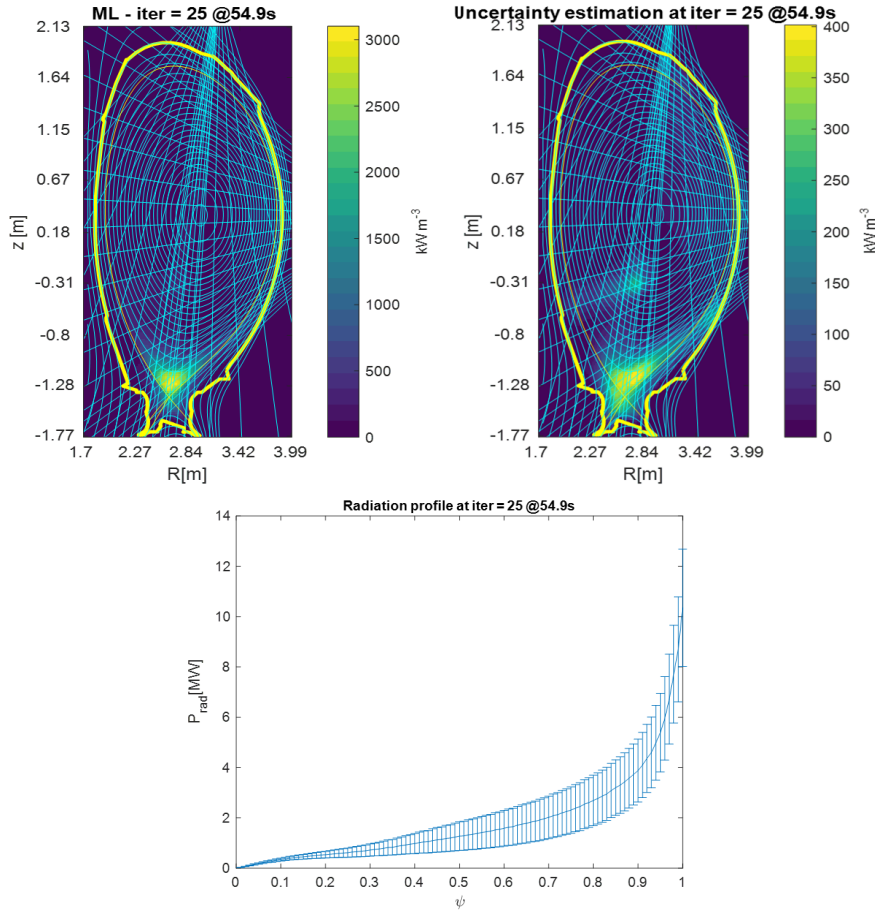
Fig. 3 Illustration of the ML bolometry for the JET pulse #84887 at t = 54.9s : reconstruction (top-left), image variance (top-right) and radiation profile PRAD versus the coordinate with the estimate of the uncertainties in the emitted power (bottom).
