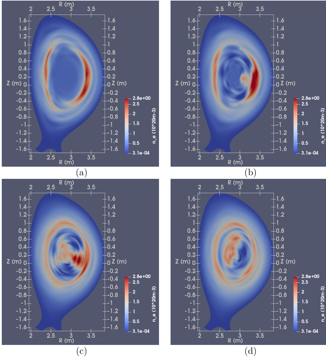
Figure 9. The density evolution during the thermal quench for the SPI, with the time corresponding to each figure being (a) t = 0.844 \text{ms} , (b) t = 0.893 \text{ms} , (c) t = 1.12 \text{ms} and (d) t = 1.26 \text{ms} . The kink motion “drags” the particles accumulated near the q = 1 surface into the plasma core.
