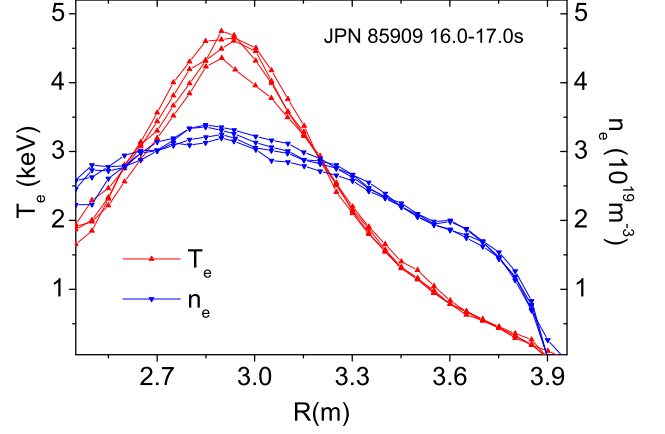
FIG. 4. Electron density and temperature profiles measured by the LIDAR Thomson scattering at JET shot #85909 in time between 16–17 s.
