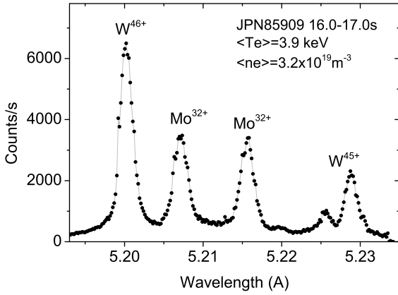
FIG. 3. Tungsten ( W^{45+} and W^{46+} ) and molybdenum ( Mo^{32+} ) x-ray lines observed in the spectrum measured at JET (shot #85909) for the T_e \approx 3.9 keV and n_e \approx 3.2 \times 10^{19} \text{ m}^{-3} .
