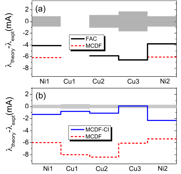
FIG. 8. Comparison of previous (a) and present (b) theoretical and experimental wavelengths of Ni1,2 and Cu1,2,3 lines. The previous experimental wavelengths are taken from Refs. [15, 21], while theoretical ones from Refs. [25, 28]. The experimental uncertainties are represented by shaded area.
