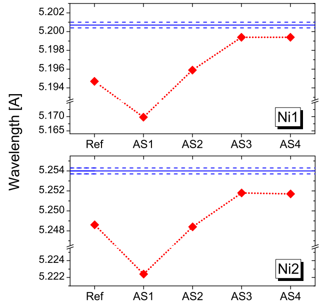
FIG. 6. The MCDF-CI wavelength calculations for Ni1 (upper) and Ni2 (bottom) tungsten lines as a function of active set (ASn) compared to the experimental values. The dotted lines with diamond symbols represent the MCDF-CI calculations, while solid and dashed lines show the experimental values and their uncertainties.
