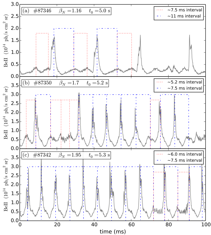
Figure 9 Emission of Be II from the inner divertor, starting at time t_0 , showing the ELMs in JET-ILW discharges (a) 87346, (b) 87350 and (c) 87342 all with high gas puff but with different (increasing) \beta_N . The dotted and dashed boxes denote the time intervals shown in each panel (the different heights of these merely aid distinguishing between them).
