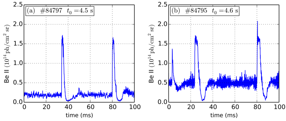
Figure 8 Emission of Be II from the inner divertor, starting at time t_0 , showing the ELMs in the low gas puff discharges (a) 84797 and (b) 84795, which do reach the peeling-ballooning boundary at the ELM onset time.
