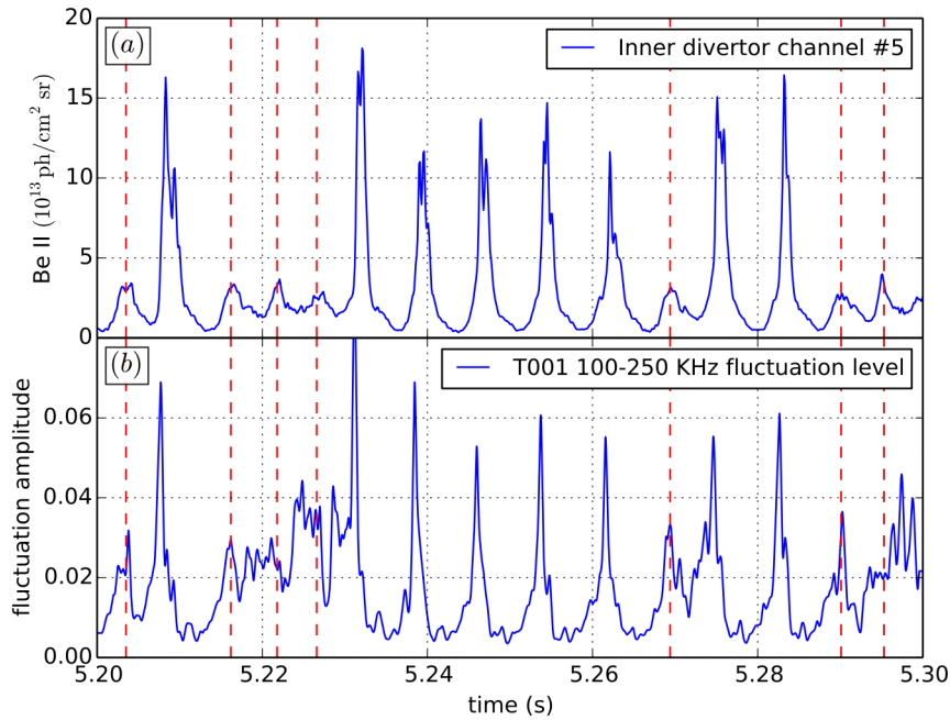
Figure 17 (a) Be II light emission in discharge 87350 compared to (b) the magnetic field fluctuation amplitude in the 100-250kHz range. The vertical dashed lines align with the peak of the oscillations in Be II emission. The magnetics data is taken from the T001 Mirnov coil positioned outboard of the plasma above the mid-plane.
