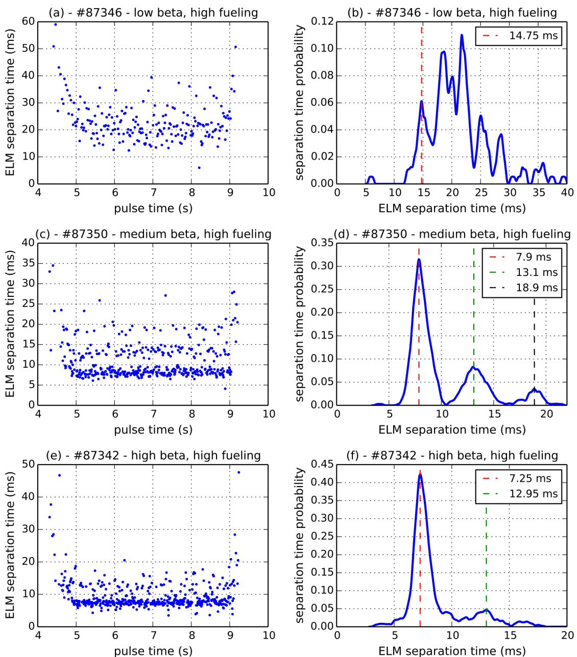
Figure 10 ELM separation time through the pulse for discharges (a) 87346, (c) 87350 and (e) 87342 and their corresponding ELM time probability distributions (b), (d), (f).
