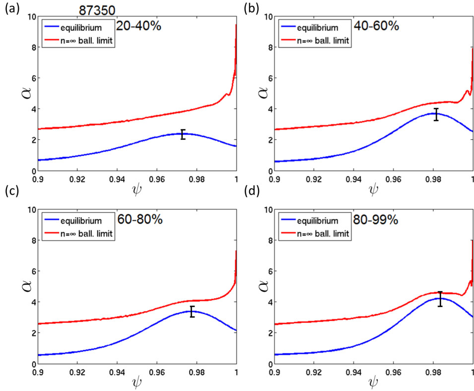
Figure 6 Comparison of the measured edge pressure gradient profile (blue, lower curve) with the ideal MHD ballooning limit (red, upper curve) as a function of normalised flux for JET-ILW discharge 87350 for each time window: (a) 20-40%, (b) 40-60%, (c) 60-80% and (d) 80-99%. \psi is the poloidal flux, normalised to \psi=1 at the separatrix. The vertical line is the 1\sigma error bar in the measured value of the maximum \alpha .
