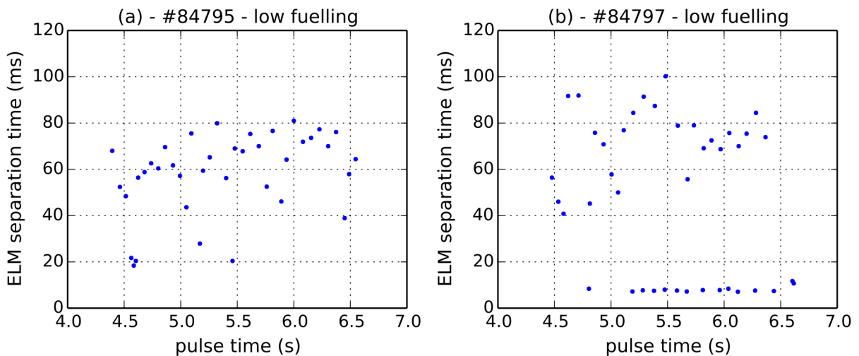
Figure 11 ELM separation times for the low gas puff shots (a) 84795 ( \beta_N=1.7 ) and (b) 84797 ( \beta_N=1.3 ).
