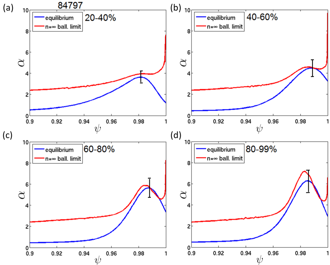
Figure 2 Comparison of the measured edge pressure gradient profile (blue, lower curve) with the ideal MHD ballooning limit (red, upper curve) as a function of normalised flux for JET-ILW discharge 84797 for each time window: (a) 20-40%, (b) 40-60%, (c) 60-80% and (d) 80-99%. \psi is the poloidal flux, normalised to \psi=1 at the separatrix. The vertical line is the 1\sigma error bar in the measured value of the maximum \alpha .
