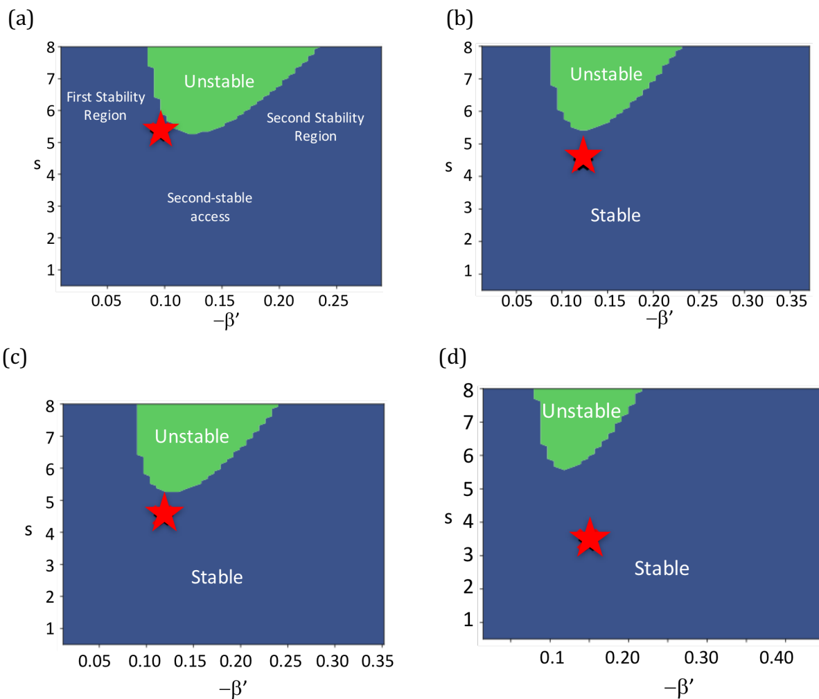
Figure 4 s - \alpha diagrams for the \psi=0.98 surface of discharge 84795 for (a) the 20-40% time window; (b) the 40-60% time window; (c) the 60-80% time window, and (d) the 80-99% window (note, \beta' is proportional to the normalised pressure gradient parameter, \alpha ). The red star denotes the equilibrium parameters.
