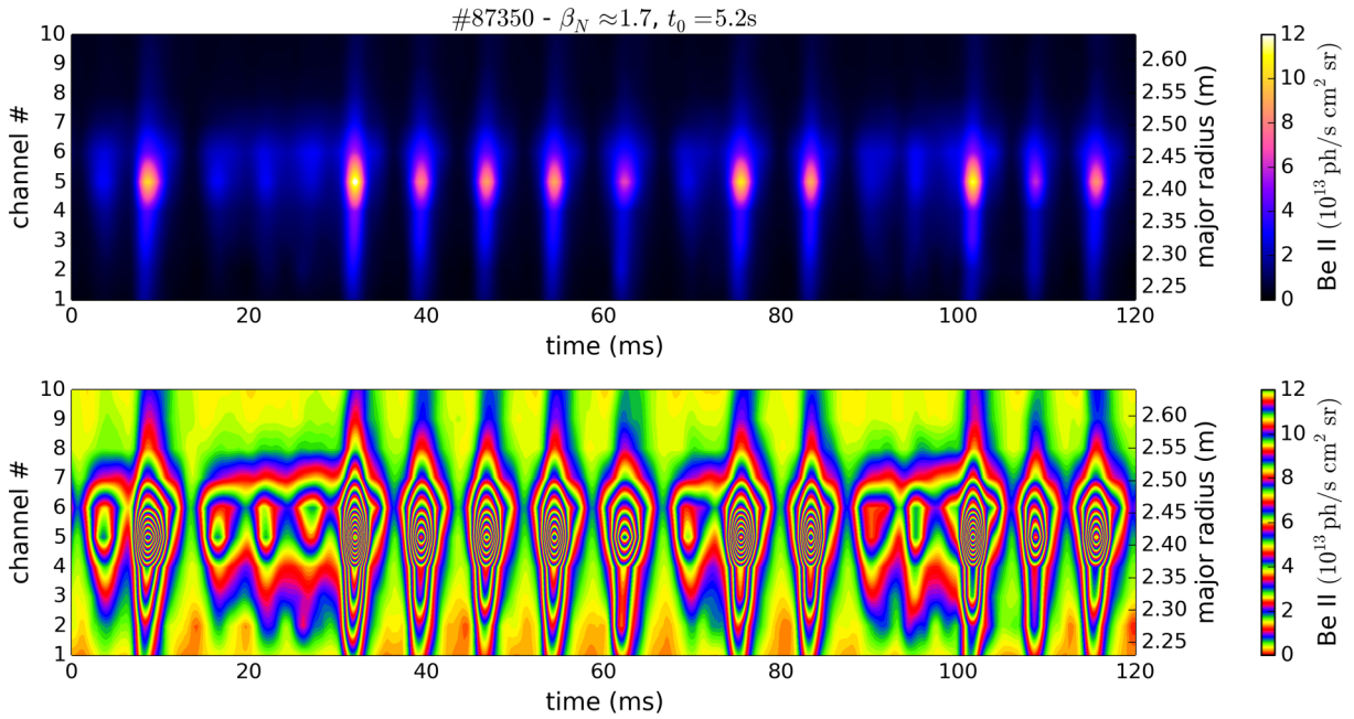
Figure 13 Be II light emission showing clear ELMs and fainter oscillations (upper) and the corresponding prism contour plot, emphasising changes in Be II emission, showing oscillations and ELMs. The channels are viewing the inner divertor region (see right-hand axis for major radius); channels 4-8 view the inner target. Shot 87350 – medium \beta , high gas puff, starting at time t_0=5.2s .
