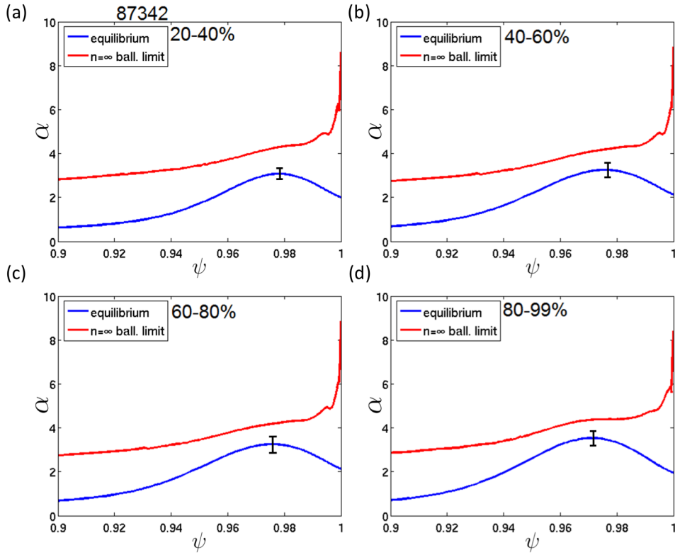
Figure 7 Comparison of the measured edge pressure gradient profile (blue, lower curve) with the ideal MHD ballooning limit (red, upper curve) as a function of normalised flux for JET-ILW discharge 87342 for each time window: (a) 20-40%, (b) 40-60%, (c) 60-80% and (d) 80-99%. \psi is the poloidal flux, normalised to \psi=1 at the separatrix. The vertical line is the 1\sigma error bar in the measured value of the maximum \alpha .
