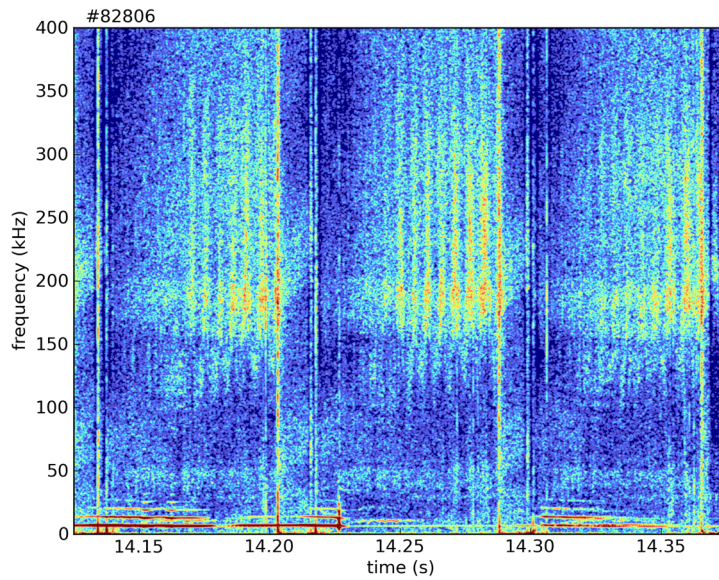
Figure 15 Spectrogram for JET discharge 82806, showing high frequency (150-350kHz) fluctuations in magnetic field with modulated amplitude occurring between the ELMs (characterised by the events that span all frequencies).
