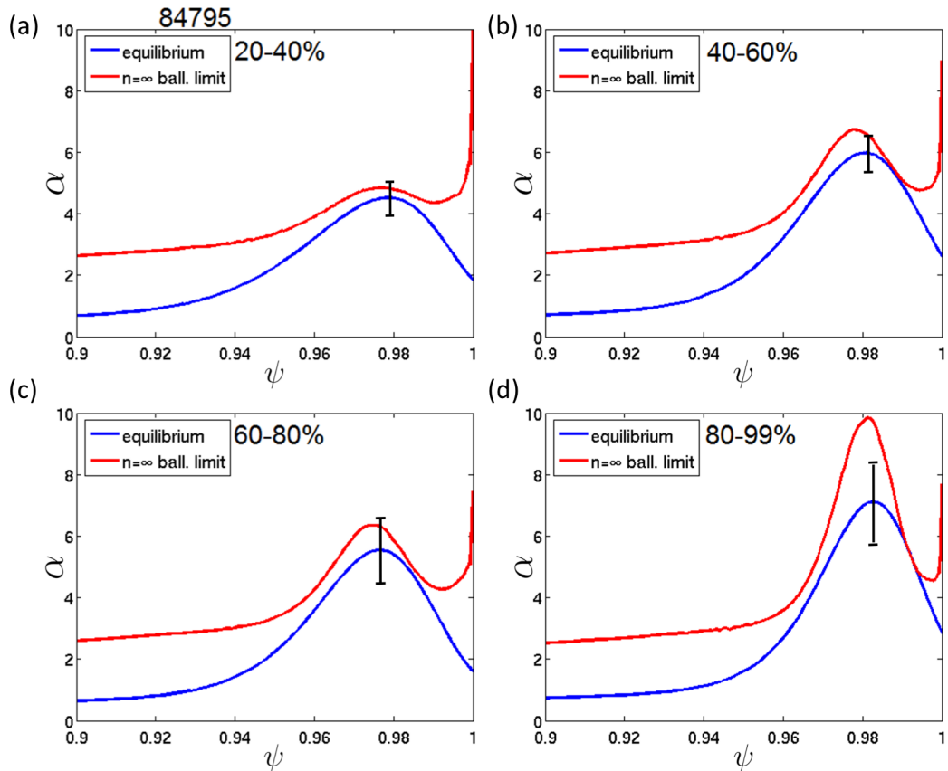
Figure 3 Comparison of the measured edge pressure gradient profile (blue, lower curve) with the ideal MHD ballooning limit (red, upper curve) as a function of normalised flux for JET-ILW discharge 84795 for each time window: (a) 20-40%, (b) 40-60%, (c) 60-80% and (d) 80-99%. The vertical line is the 1\sigma error bar in the measured value of the maximum \alpha .
