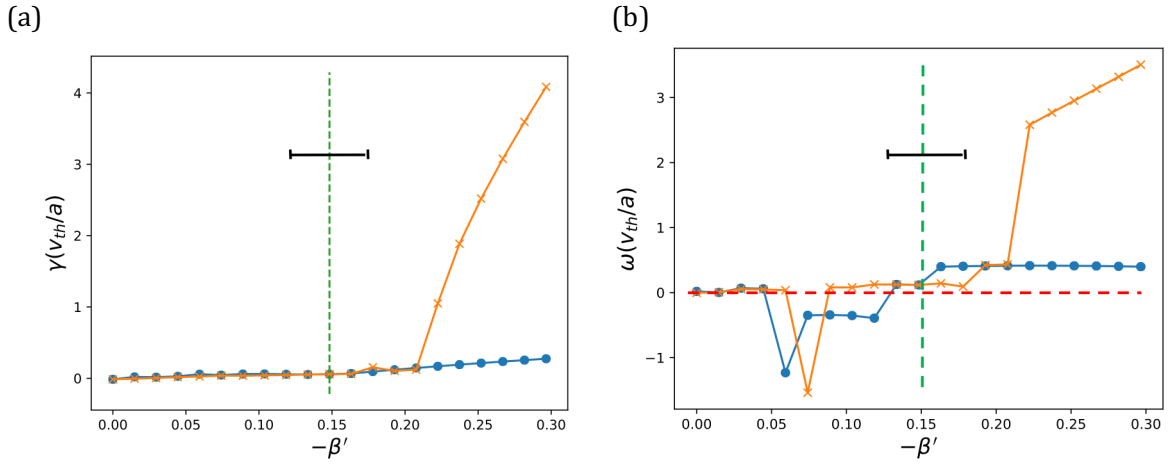
Figure 5 (a) Growth rate \gamma and (b) mode frequency \omega from a local solution to the gyrokinetic equation provided by the GS2 code for the 80-99% window of discharge 84795 at \psi=0.98 , which is in the ideal ballooning second stability region (corresponding to Fig 4d). We have fixed k_y \rho_s = 0.1 (i.e. n=24 ), and \omega < 0 corresponds to propagation in the electron diamagnetic direction. The vertical dashed line denotes the equilibrium value of normalised pressure gradient, \beta' , about which we perturb by increasing density and temperature gradients at the same rate (ie fixed \eta_{i,e} ). The blue curve with full circles shows the result for self-consistently modifying the local equilibrium, while the yellow curve with crosses shows the result when the equilibrium is not adjusted with \beta' ; \gamma and \omega are normalised to v_{th}/a ( v_{th} is the thermal velocity and a the minor radius). The horizontal bar is the 1\sigma error in the experimental value of \beta' .
