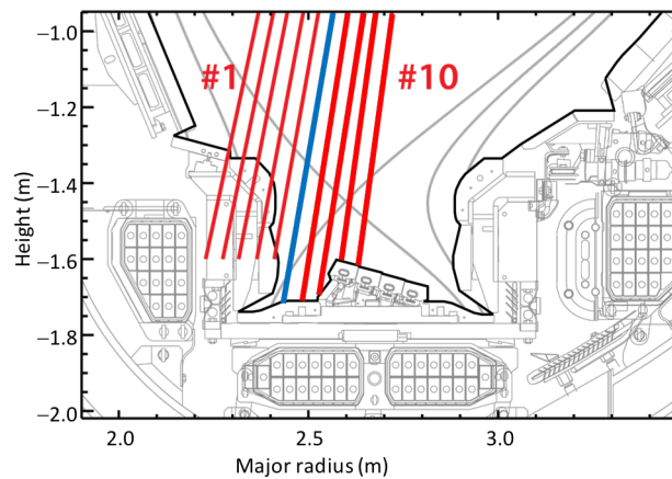
Figure 14 Lines of sight for the Be II emission data shown in Fig 13 with channel #1 at the left increasing to channel #10 at the right. Superimposed is the separatrix for shot 87350 at t=5.7s . The blue line denotes the line of sight for channel #6, which is close to the strike point – the peak in emission is between channels #5 and #6.
