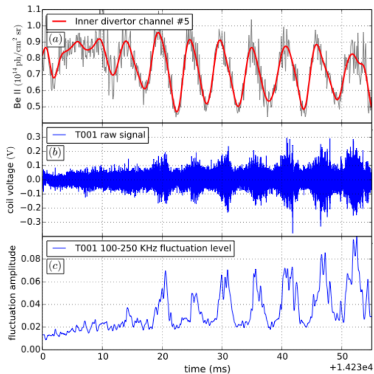
Figure 16 (a) Oscillations in the Be II light emission from the inner divertor during an inter-ELM period in discharge 82806 (red curve shows smoothed data) compared to (b) Mirnov coil data from the T001 coil positioned outboard of the plasma above the mid-plane, and (c) fluctuation amplitude integrating over the 100-250 kHz frequency range.
