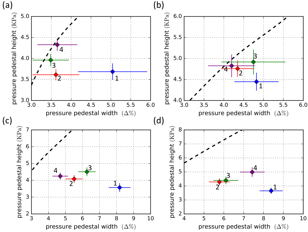
Figure 1 Evolution of pedestal height and width for JET discharges (a) 84797, (b) 84795, (c) 87350 and (d) 87342 (1: 20-40% blue diamond; 2: 40-60% red diamond; 3: 60-80% green diamond; 4: 80-99% purple diamond). The curve shows the peeling-ballooning boundary evaluated for the 80-99% period. (a) and (b) are low gas puff, while (c) and (d) are high gas puff.
