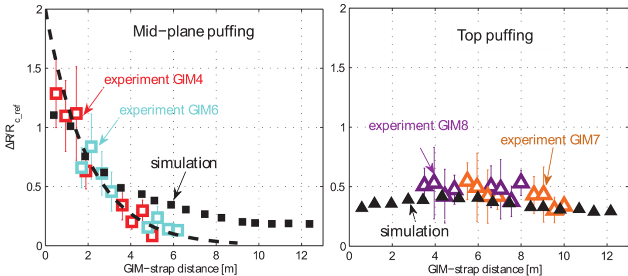
Figure 10. Relative Change of Coupling Resistances (RCCR) vs. GIM-antenna strap distance. For the calculated RCCR values, because they are largely symmetry along \phi=0^\circ , only those in the toroidal range [0, 180^\circ] are shown in the figure. The experimental RCCR values are reproduced from [10]. Left: RCCR during mid-plane gas puffing, in which the dashed line is a fit of the experimental data. Right: RCCR during top gas puffing.
