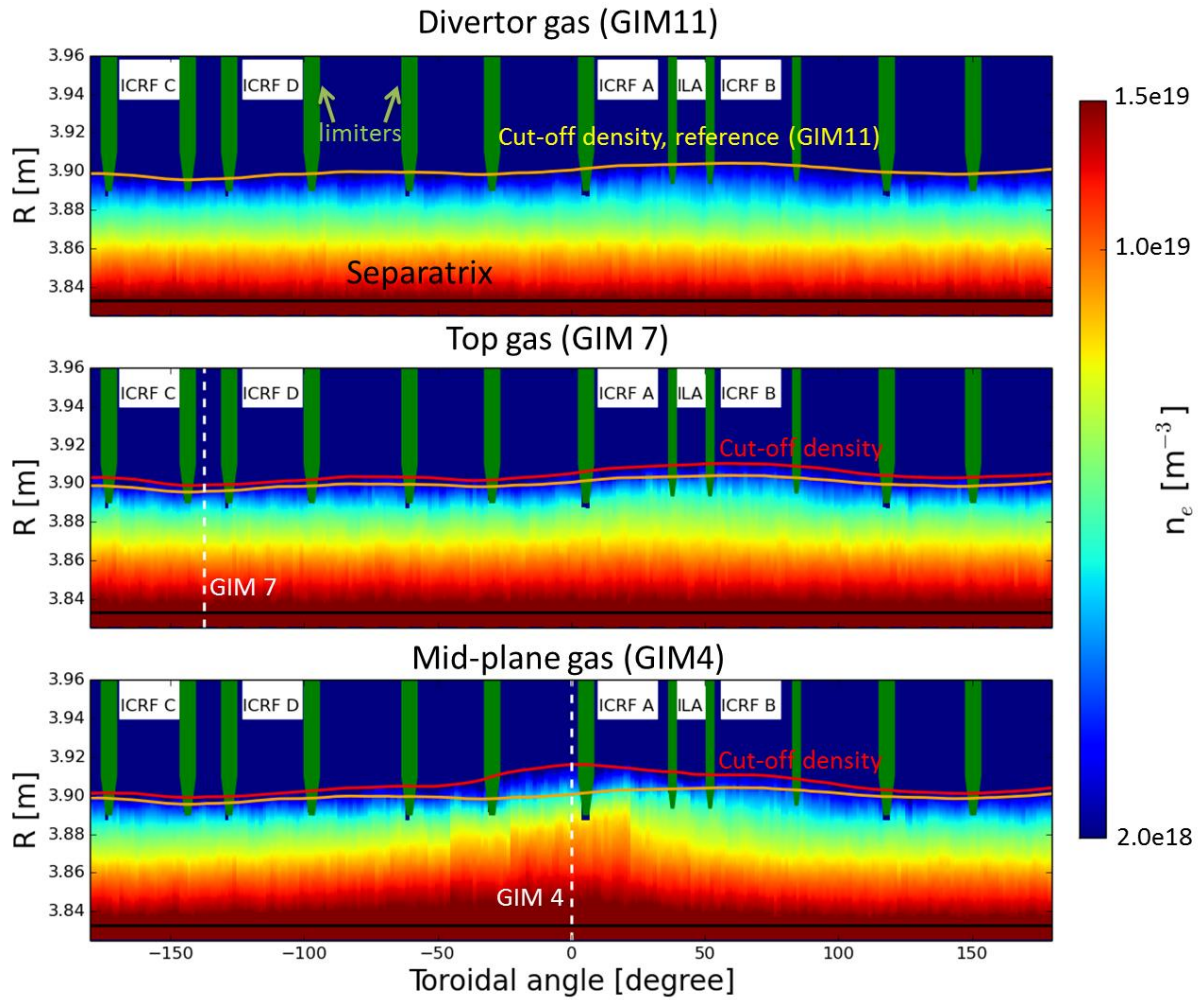
Figure 8. Toroidal cross-sections of the electron density in the outer mid-plane for the divertor, top and mid-plane gas puff cases. The yellow solid line is the position of cut-off density for divertor gas puffing and reported in the second and third subfigures as reference line. The red solid-line is the position of cut-off density for top or mid-plane gas puffing.
