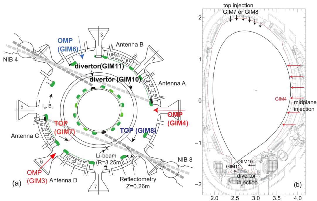
Figure 1. (a) Top view of JET illustrating the toroidal locations of the plasma facing wall components, the GIMs and the key density diagnostics; (b) poloidal cross-section of JET shows the gas route puffed from different GIMs. Figure reproduced from [5].
