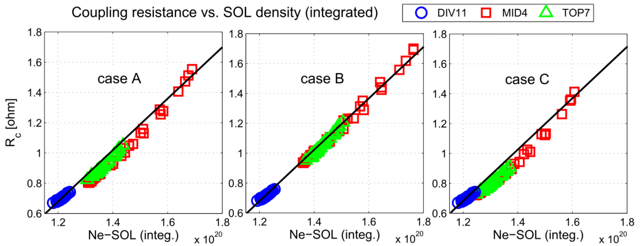
Figure 12. Measured coupling resistance vs. integrated SOL density.
