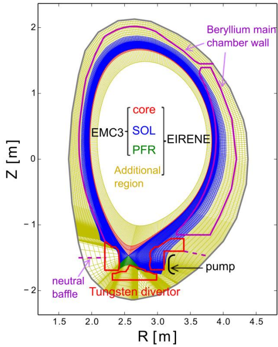
Figure 2. A poloidal cross-section of the EMC3-EIRENE computation grid.
