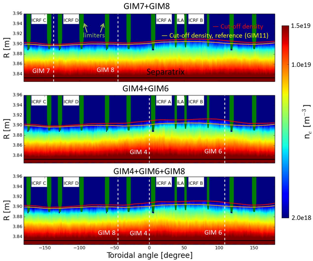
Figure 14. Toroidal cross-sections of the electron density in the mid-plane for combined gas puffing scenarios.
