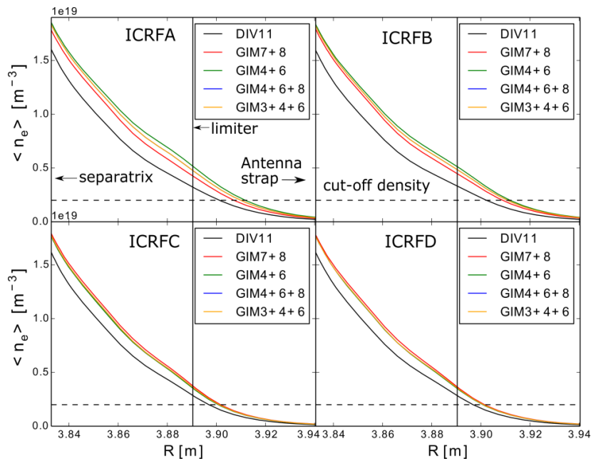
Figure 15. Averaged density in front of the antennas for combined gas puffing scenarios.
