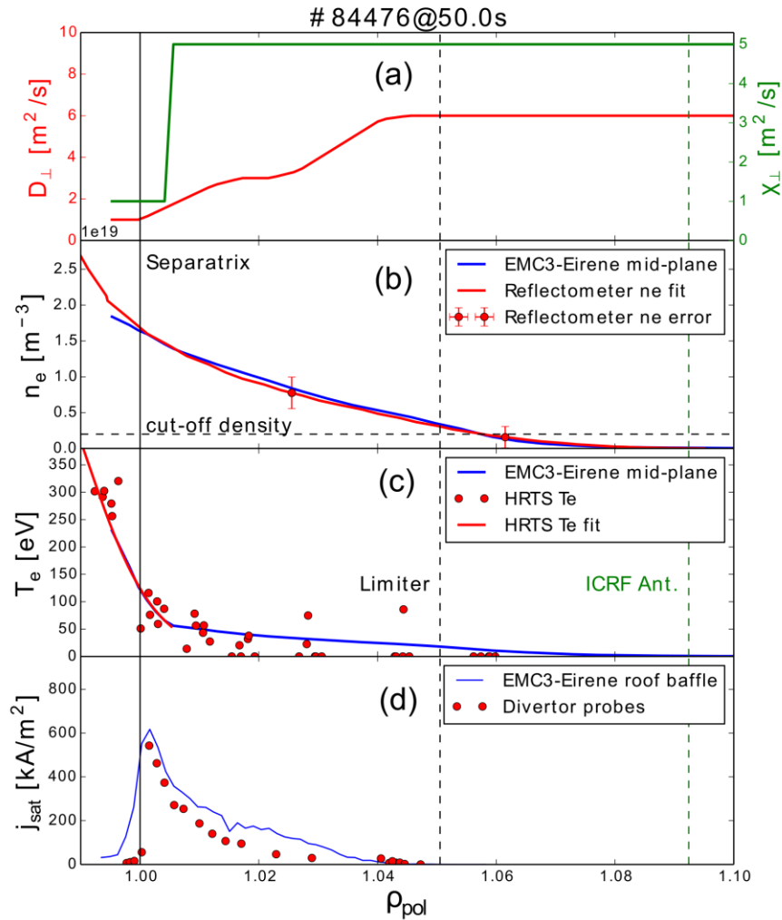
Figure 4. Matching the background plasma parameters with experiments: (a) perpendicular plasma transport coefficients D_{\perp} and \chi_{\perp} ; (b) comparisons of mid-plane electron density, the error bars correspond to the statistical dispersion of the reflectometry data; (c) comparisons of mid-plane electron temperature; (d) comparisons of particle fluxes to the divertor (around the outer strike point in the roof baffle).
