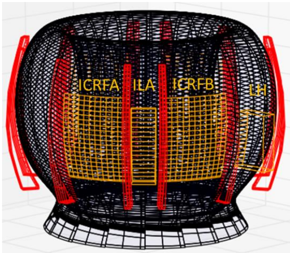
Figure 3. 3D structure of the computational grid, the limiters and the antennas.
