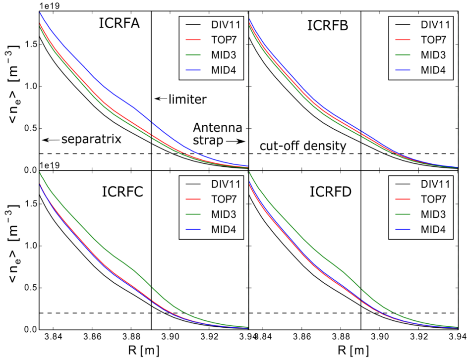
Figure 9. The calculated average density in front of the ICRF antennas for the divertor (GIM11), top (GIM7) and mid-plane (GIM3 and GIM4) gas puff cases. ICRFA means ICRF antenna A.
