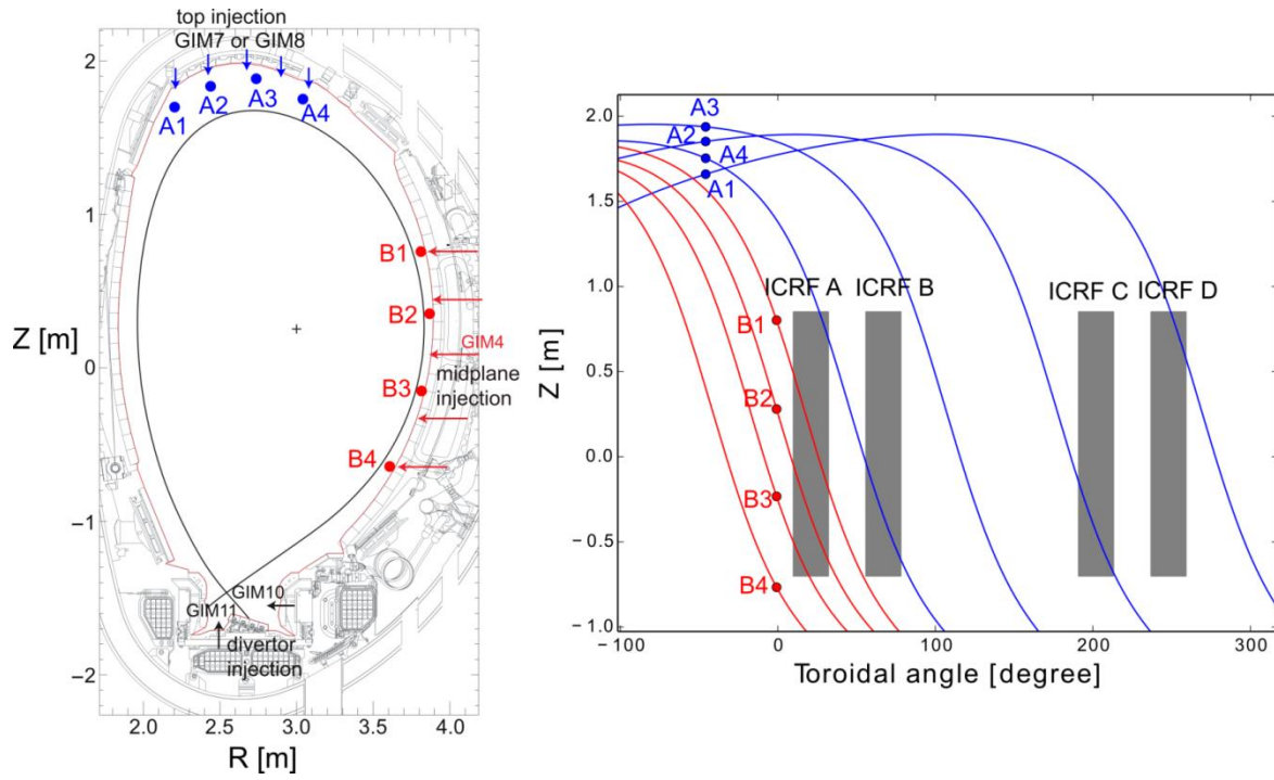
Figure 13. Field line tracings starting from the top gas cloud (points A1, A2, A3 and A4, toroidal angle= -45^\circ ) and mid-plane gas cloud (points B1, B2, B3 and B4, toroidal angle= 0^\circ ), respectively.
