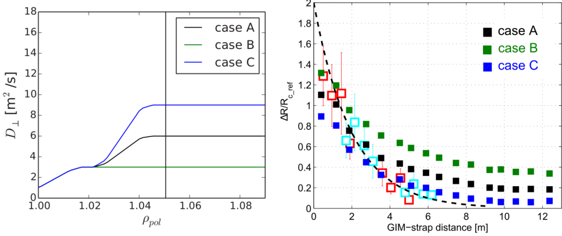
Figure 11. Influences of the particle transport coefficient D_{\perp} on the ICRF coupling. Left: particle transport coefficients in the three cases investigated; right: the corresponding relative change of coupling resistances.
