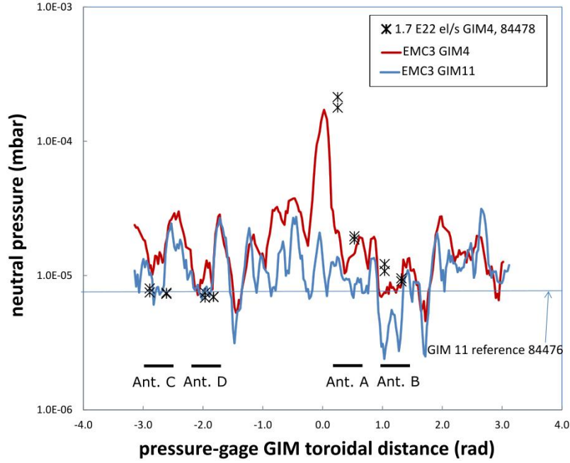
Figure 6. Comparisons of simulated and experimental gas pressure during mid-plane (GIM4) and divertor (GIM11) gas puffing. The pressure measurements are made in the A2 antennas in-vacuum transmission lines (un-pumped).
