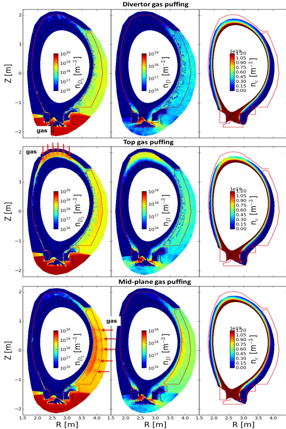
Figure 5. Poloidal cross-sections of the neutral density ( n_{D_2} for molecular and n_D for atom) and electron density ( n_e ) during divertor, top and mid-plane gas puffing, respectively. The poloidal cross-sections are chosen at toroidal positions where the GIMs are located.
