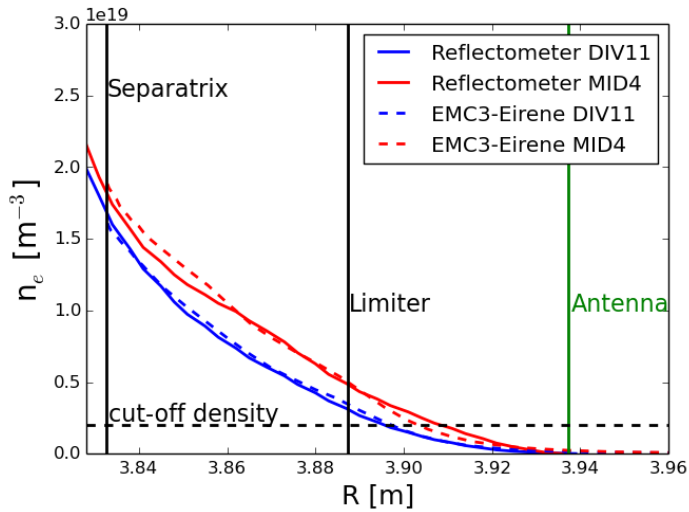
Figure 7. Comparisons of simulated and experimental density (measured with reflectometer) for mid-plane (GIM4) and divertor (GIM11) gas puffing. DIV11 means divertor puffing with GIM11 and MID4 means mid-plane puffing with GIM4.
