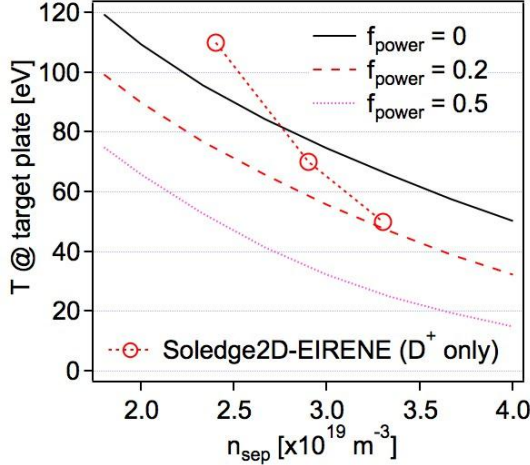
Fig. 17: Plasma temperature in front of the target plates as a function of separatrix (upstream) density from a two points model, for P_{SOL}=6MW and \lambda_Q=5mm and various levels of radiated power in the SOL. Open circles are pure deuterium Soledge2D-EIRENE calculations for the same parameters.
