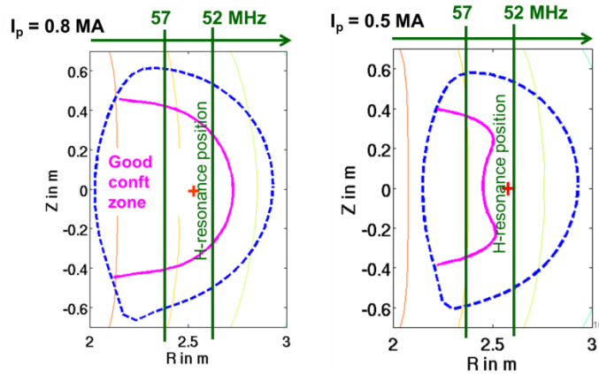
FIG. 9. Poloidal views of WEST equilibria at 0.8 and 0.5 MA in steady state computed by CEDRES++ see Fig.2. The unshifted H resonance positions are indicated in green for two ICRH frequencies: 52 and 57 MHz. In magenta are shown the limits of the good confinement region.
