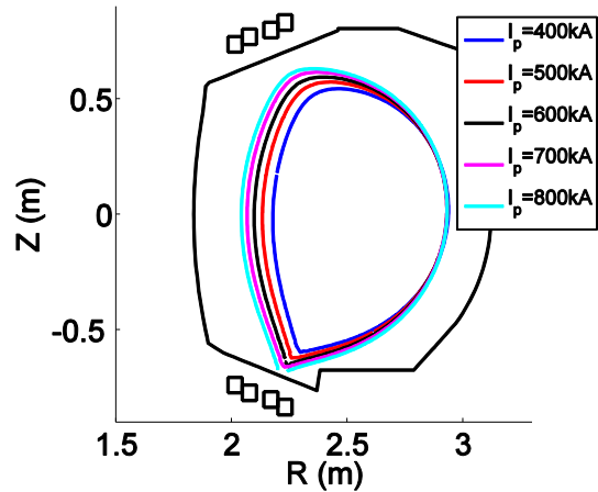
FIG.2. CEDRES++ free boundary set of equilibria for B_T = 3.7 T (at 2.5 m); with a fixed external radius of 2.93 m and with the steady state divertor coil current of 200 kA.turn.
