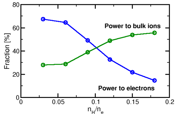
FIG. 12. Influence of the hydrogen minority concentration on the power split between electrons and bulk ions.
