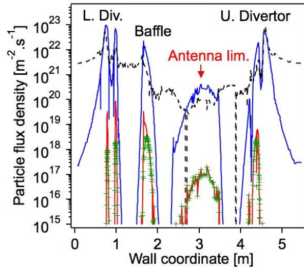
Fig. 19: Particle flux densities as a function of the poloidal location, from the lower to the upper divertor via the low field side elements (baffle and antenna limiters). D^+ flux (solid blue), D flux (dashed black), W gross influx from ions (solid red) and net influx from ions (green crosses), i.e. accounting for prompt redeposition, but without sheath rectification..
