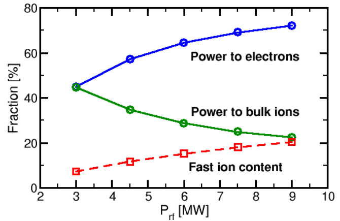
FIG. 11. Power split between electrons and bulk ions (solid lines) when the coupled RF power is varied between 3MW and 9MW, at 6% H minority concentration. Also shown is the fast ion content (dashed line).
