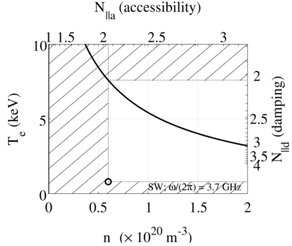
FIG. 7. LHCD accessibility diagram at 3.7 GHz
