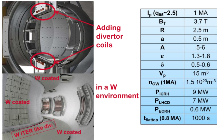
Fig. 1: CAD views of WEST and a table summarizing the WEST main parameters.
