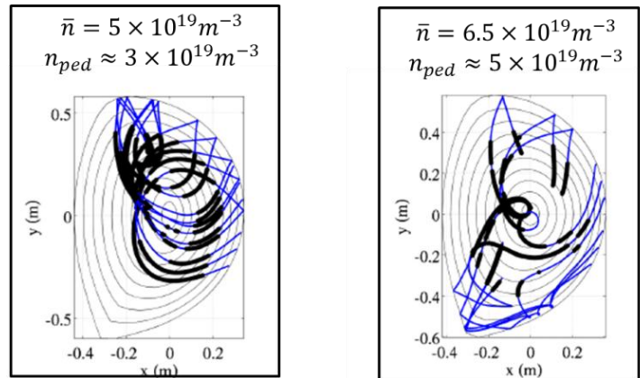
FIG. 8. C3PO-LUKE LH modelling for two WEST scenarios.
