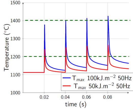
FIG.16: Estimate of the temperature increase of the W monoblocks linked to ELMs, for a steady state heat load of 10 \text{ MW/m}^2 , and large type I ELMs of 50 and 100 \text{ kJ/m}^2 , red and blue curve respectively, 50 Hz frequency. The W recrystallization temperature range is bordered by green dashed lines.
