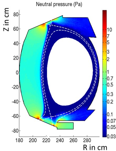
FIG.13. Neutral pressure in a poloidal cross section of WEST modeled by SolEdge2D-EIRENE [Buf13]
