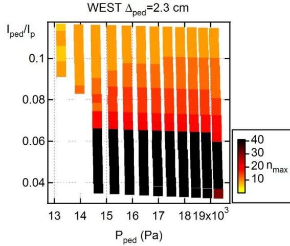
Fig. 15: Ideal MHD limit computed by MISHKA [Huy07] for I_p=0.8 MA. The low wave number modes are the peeling modes and the higher wave number modes are the ballooning modes.
