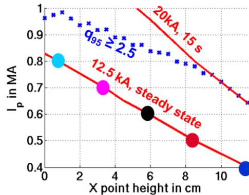
FIG.3. At fixed B_T=3.7 T, range of accessible I_p and X point heights corresponding to the references equilibria illustrated by FIG.2. The limits due to the divertor coils are in red, one for the steady state and one corresponding to the maximal divertor coils current. In blue is the limit corresponding to q_{95}=2.5 .
