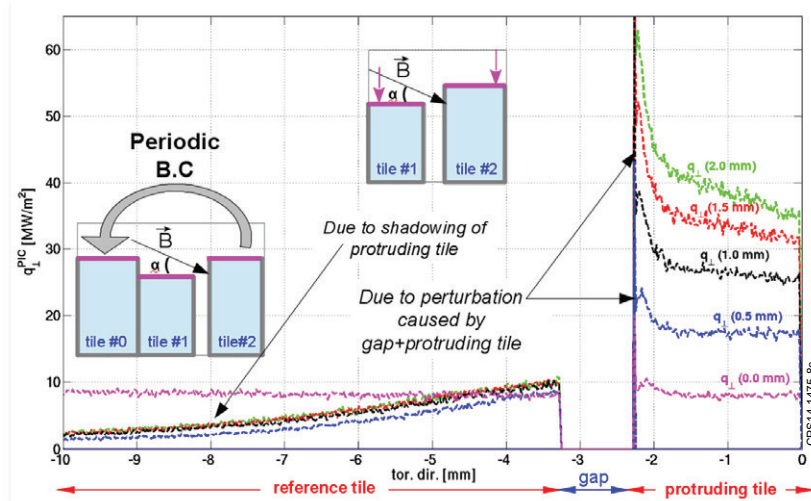
Figure 8: Power deposition profiles on the top surface of the lamella for scenario S3 and the 4 simulated misalignments
