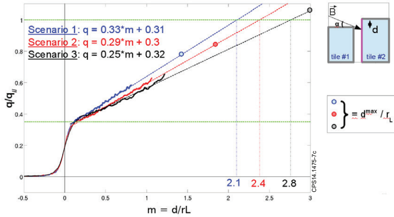
Figure 7: Scaling of the power deposition profiles on the lamella side (normalized to q_{||} ) as a function of the misalignment normalized to r_L
