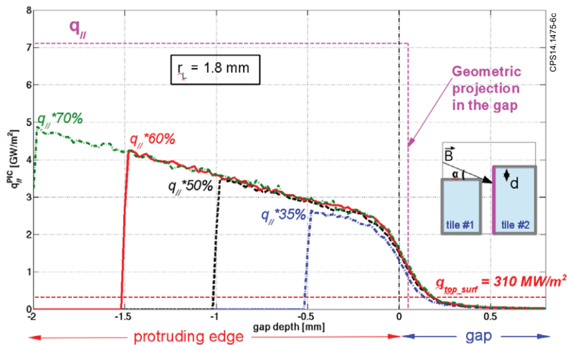
Figure 6: Power deposition profiles along the misaligned lamella side (including down below the surface defined by the neighboring lamella) for scenario S1 and 4 simulated misalignments. The theoretically expected power fluxes on the top surface and the parallel heat flux in the absence of any finite Larmor radius effects are marked for comparison
