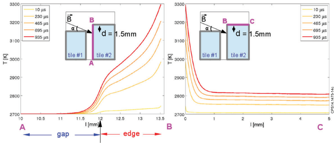
Figure 14: Spatial profiles of the surface temperature on the side (left) and top (right) of the lamella for at different times and for a misalignment of d = 1.5\text{mm} for ELM plasma parameters corresponding to Scenario S2
