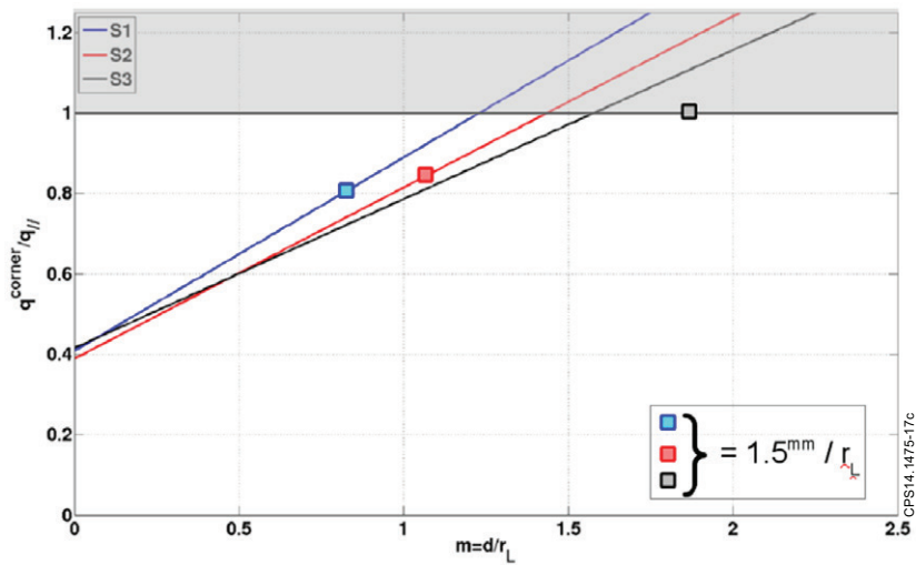
Figure 17: Scaling law for the power flux normalized to q_{||} falling on the corner of the lamella for different ELM scenarios as a function of the misalignment normalized to r_L .
