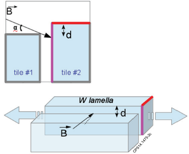
Figure 2: Schematic of the (semi-infinite) lamella as modeled in the 2D PIC simulations
