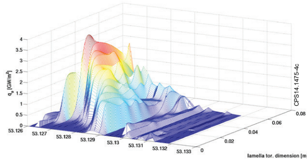
Figure 4: Temporal evolution of the spatial distribution of the power density falling on the lamella during one ELM, measured by IR thermography for 1 of the 5 melting discharges (JET Pulse Number 84779)
