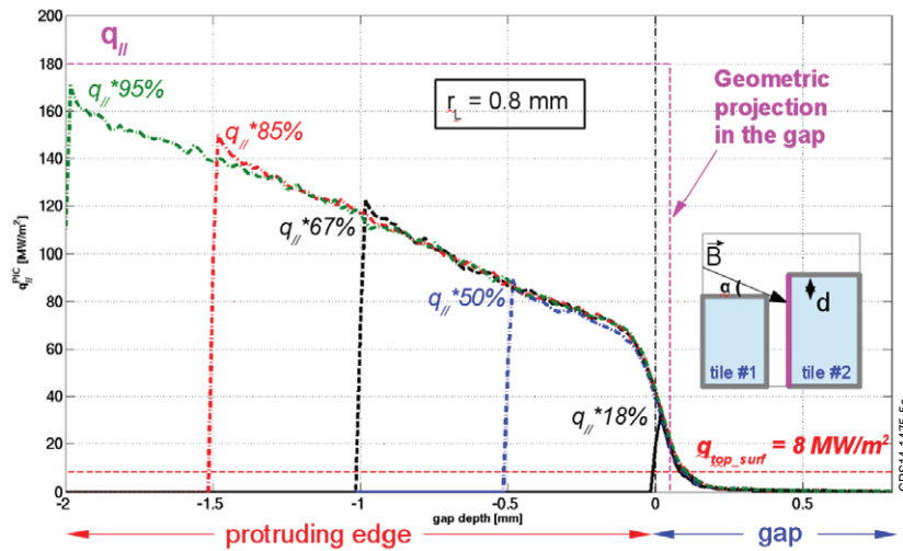
Figure 5: Power deposition profiles along the misaligned lamella side (including down below the surface defined by the neighboring lamella) for scenario S3 and 4 simulated misalignments. The theoretically expected power fluxes on the top surface and the parallel heat flux in the absence of any finite Larmor radius effects are marked for comparison
