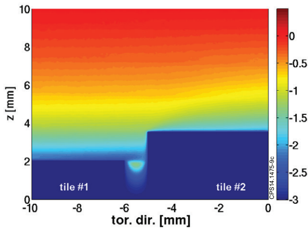
Figure 9: Electric field at the side of the lamella from the bottom of the gap to the top corner for 2mm protruding distance computed by 2D PIC calculations
