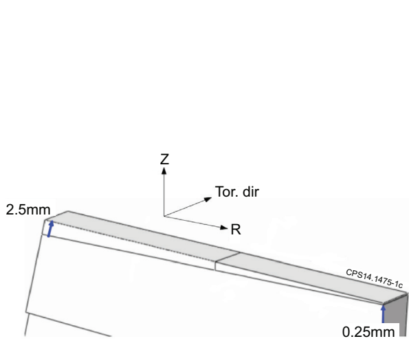
Figure 1: Schematic of the special protruding lamella in the JET divertor [10]
