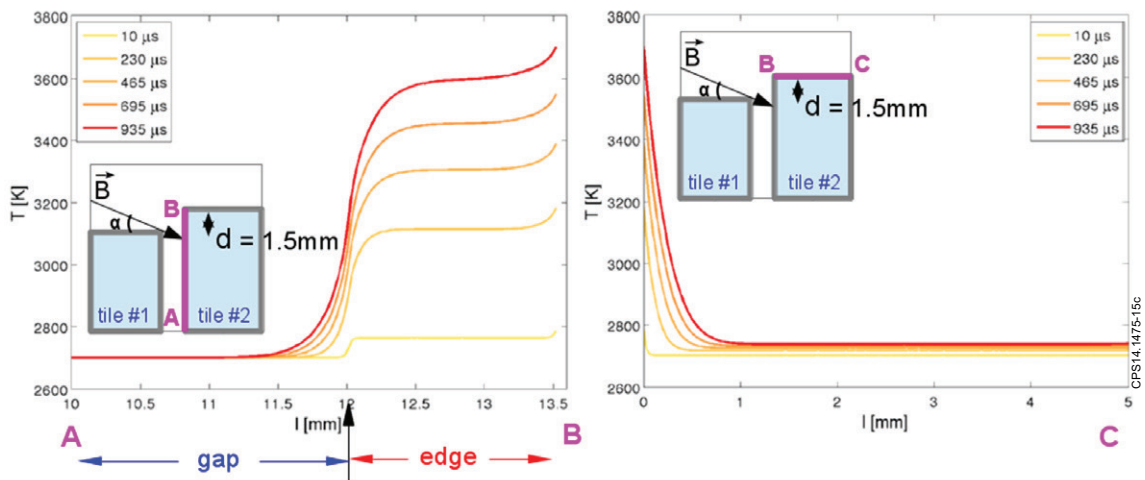
Figure 15: Spatial profiles of the surface temperature on the side (left) and top (right) of the lamella for at different times and for a misalignment of d = 1.5\text{mm} for ELM plasma parameters corresponding to Scenario S2
