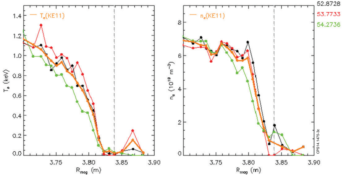
Figure 3: Pedestal profiles of electron temperature (left) and density (right) given by Thomson scattering for 1 of the 5 melting discharges (JET Pulse Number 84781) at 3 different times corresponding to the lamella exposure to high heat loads
