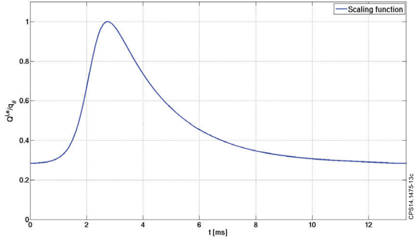
Figure 13: Temporal evolution of the normalized power flux for 1 ELM in JET
