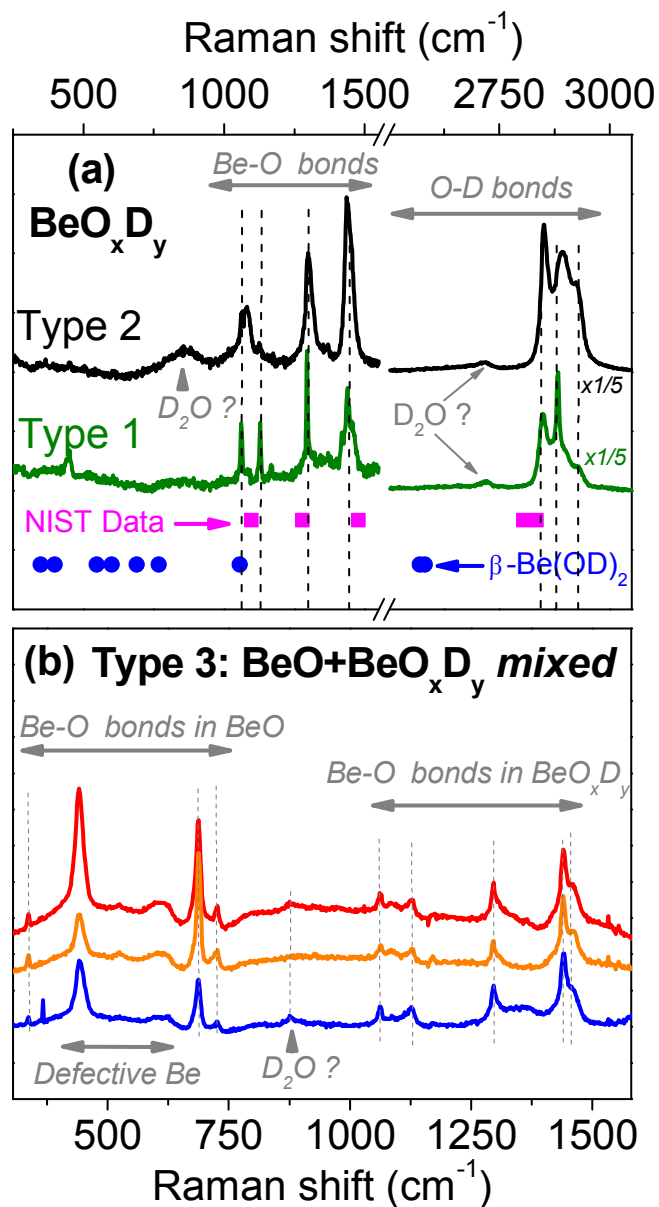
Figure 2. Raman spectra of the 2011-2012 campaign tile in various zones. (a) Identification of Type 1 and Type 2 deuterioxides. The intensity corresponding to the 2700-3000 \text{cm}^{-1} spectral range has been divided by 5. Blue points are from [30] and magenta points are from [31] (b) Identification of Type 3 deuterioxide, coexisting with the oxide. A background due to carbon contamination was removed in (a) and (b).
