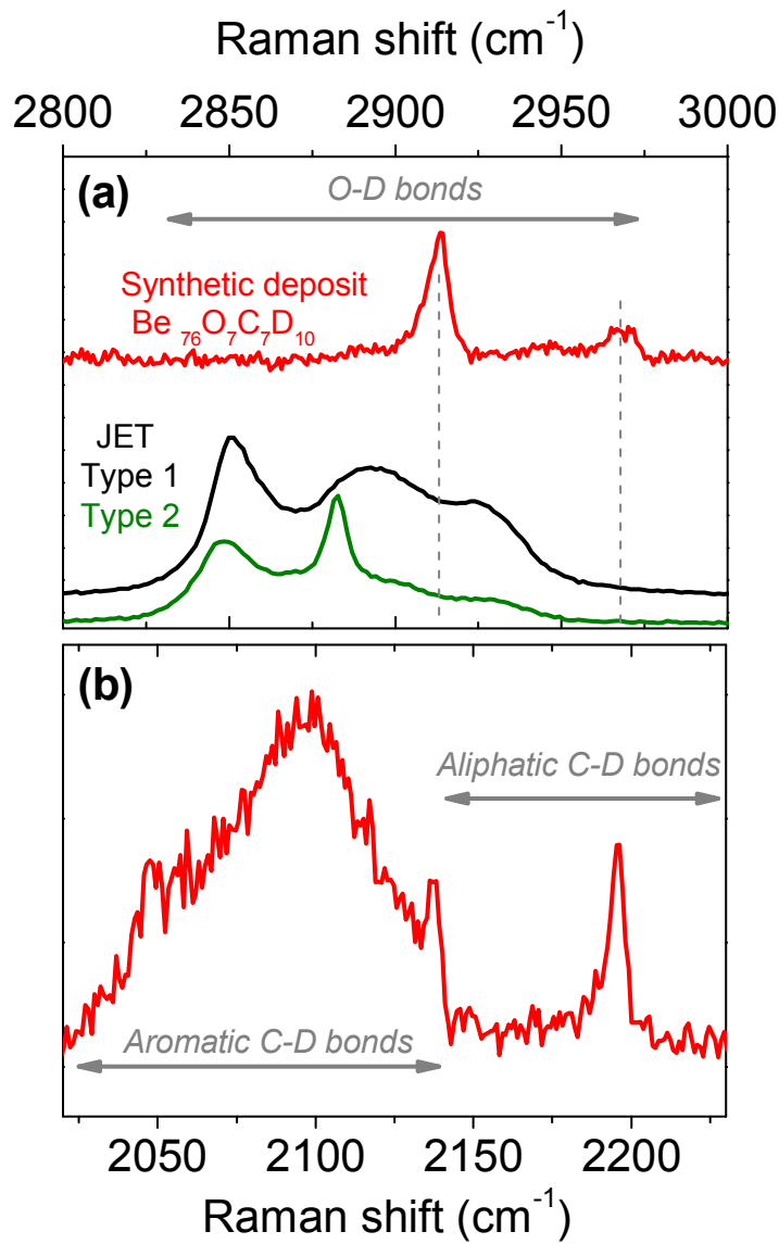
Figure 5. Comparison of a sample mimicking JET tile 1 divertor deposit (non-melted) and the 2011-2012 campaign tile (melted). (a) O-D spectral region. (b) C-D spectral region. Note that a very intense background, not yet understood, has been subtracted from the synthetic deposit spectrum.
