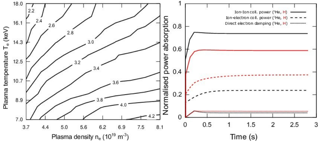
FIG. 7. Difference in total collisional power to the bulk ions (in MW) for a ^3\text{He} compared to H minority scheme (left). Ion-ion collisional heating (solid), ion-electron collisional heating (dashed) and direct electron heating (dotted) for n_e = 6.e10^{19} and T_e = T_i = 8.9 \text{ keV} (right)
