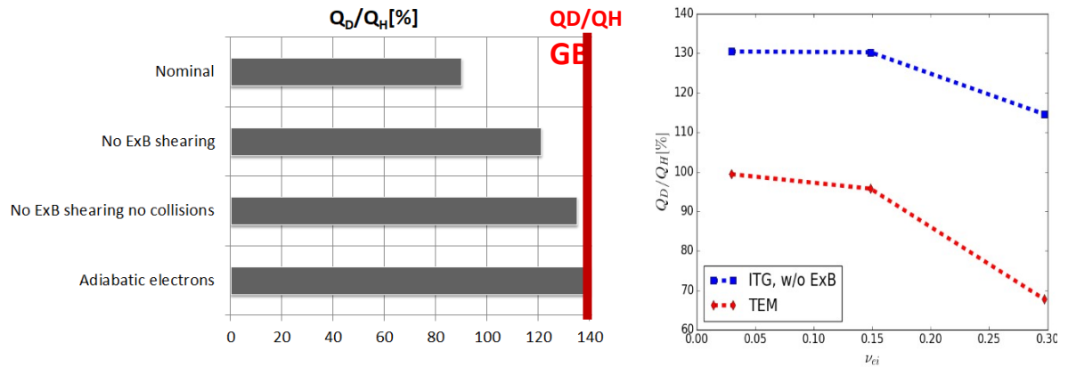
FIG.4. Ratio of the ion heat flux in deuterium and hydrogen Q_D/Q_H obtained with GENE from the discharge 91450. The vertical red line determines the GyroBohm scaling (Left) Dependence of the ratio Q_D/Q_H on collisionality for ITG vs TEM
