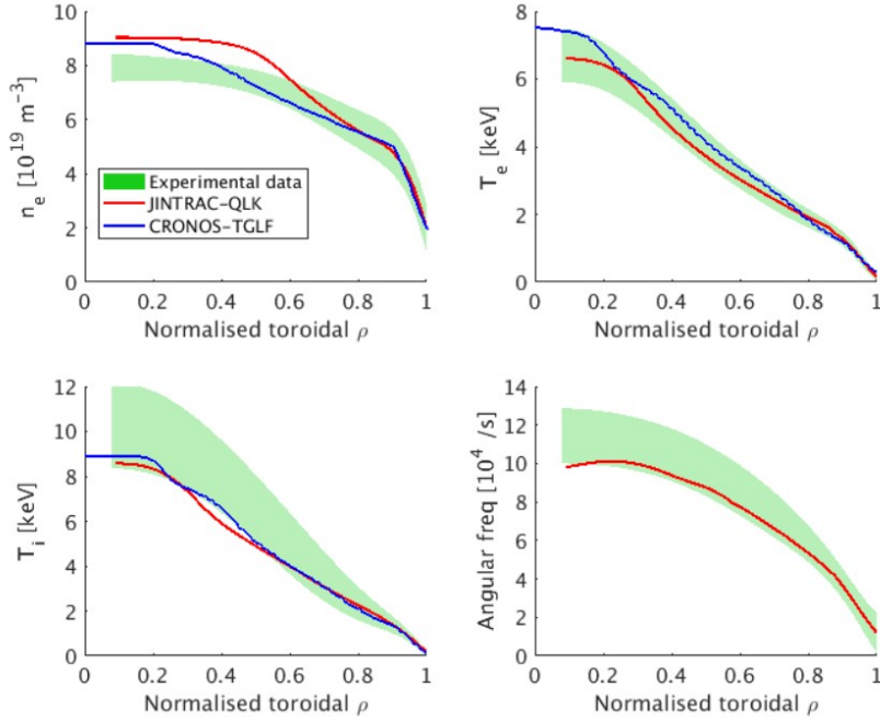
FIG. 1. Comparison between simulated and experimental temperature (electron, T_e , and ion, T_i ) and electron density ( n_e ) profiles for the discharge 92436 at t=50.4\text{s} simulated with CRONOS and TGLF taking the experimental rotation profile. Comparison between simulated and experimental temperature (electron and ion), electron density and rotation profiles for the discharge 92436 at t=50.4\text{s} simulated with JINTRAC and Qualikiz. High Resolution Thomson Scattering (HRTS) is used for n_e and T_e , Charge Exchange (CX) for T_i and the toroidal rotation. The profiles are shifted in order to have T_e=100\text{eV} at the separatrix.
